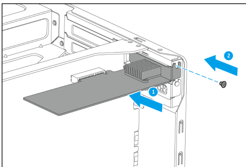
PCIe low-profile port
