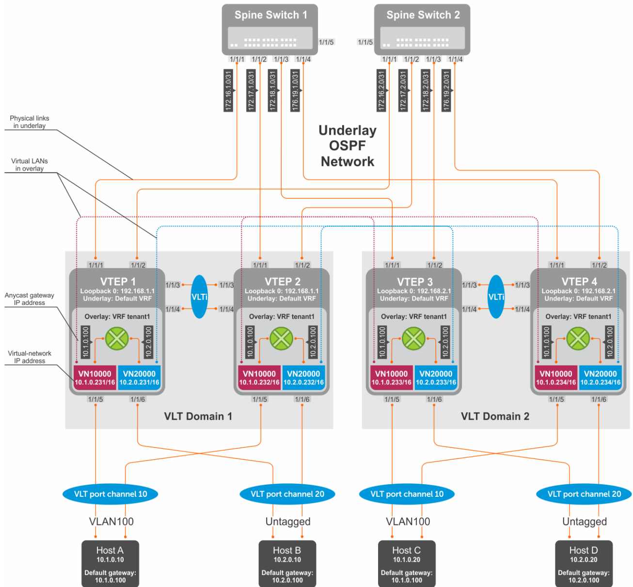
Figure 12. Static VXLAN use case
