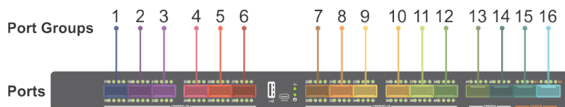
Figure 7. MX9116n Fabric Switching Engine unified port groups
