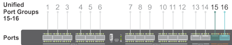
Figure 5. MX9116n Fabric Switching Engine — Unified port groups
