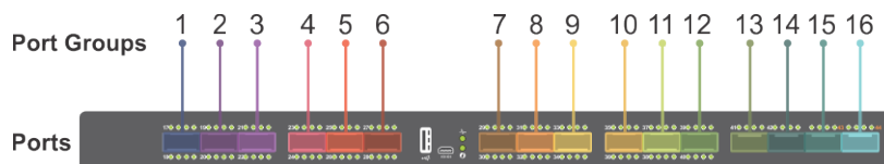
Figure 3. MX9116n Fabric Switching Engine unified port groups
