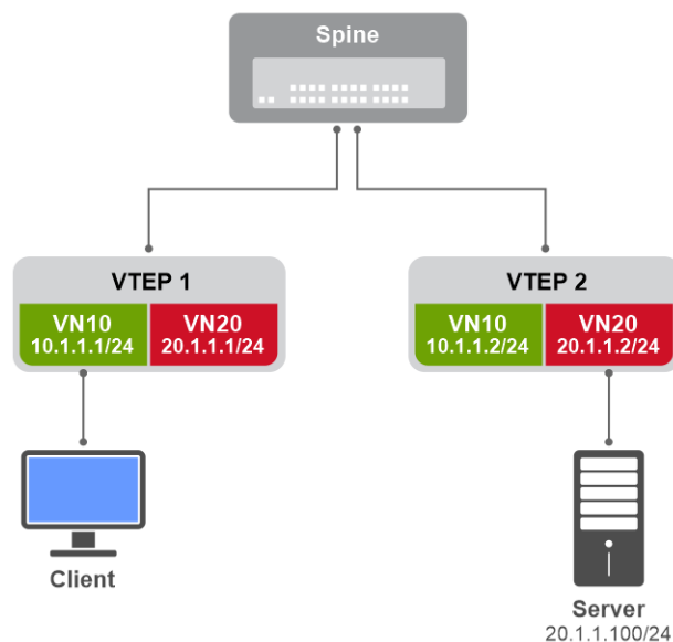
Figure 9. Route leaking between VRFs with asymmetric IRB routing
