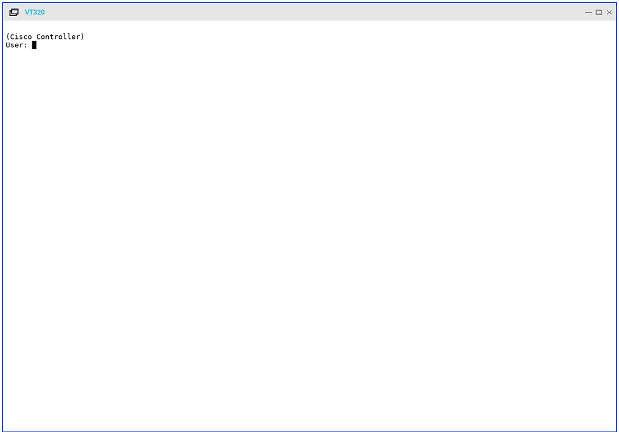
Figure 37. Telnet window
