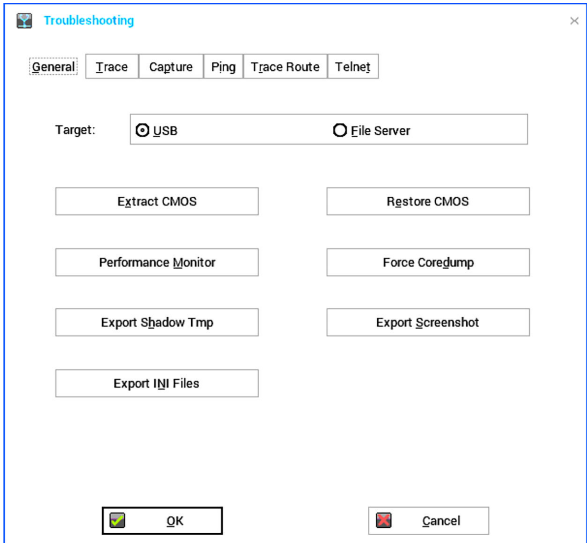
Figure 31. General
