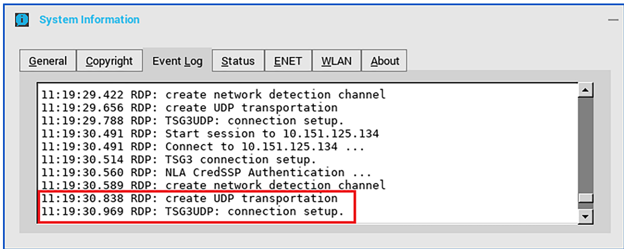
Figure 23. Event log
