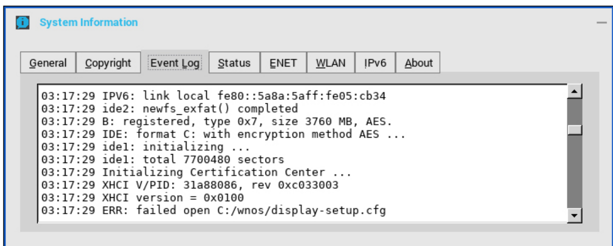
Figure 30. Event log tab
