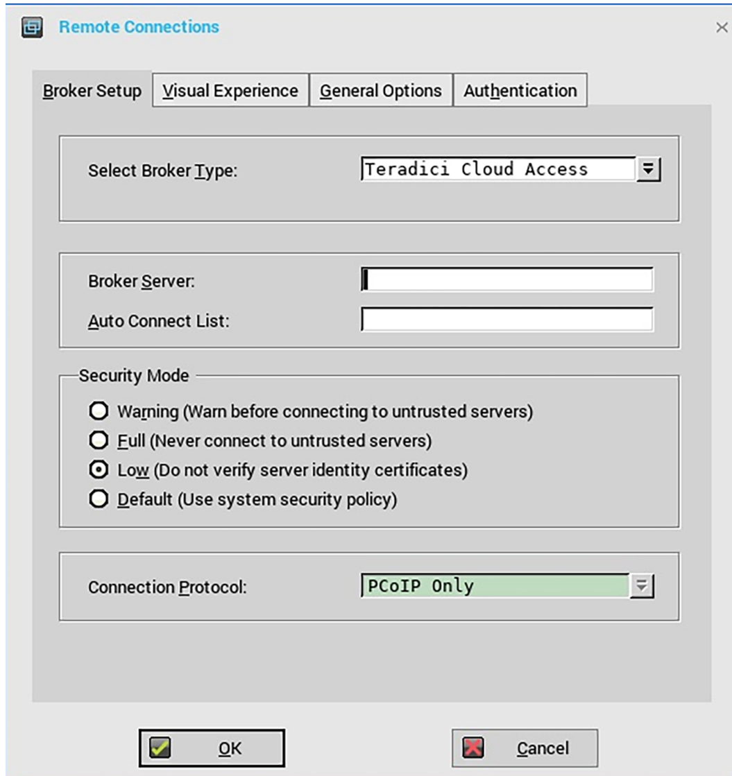
Figure 24. Broker setup - Teradici Cloud Access
