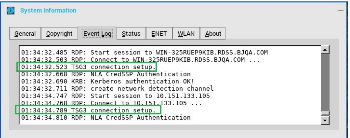
Figure 22. Event log tab
