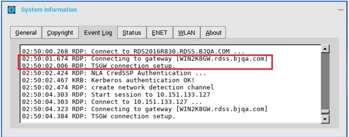
Figure 21. Event log tab
