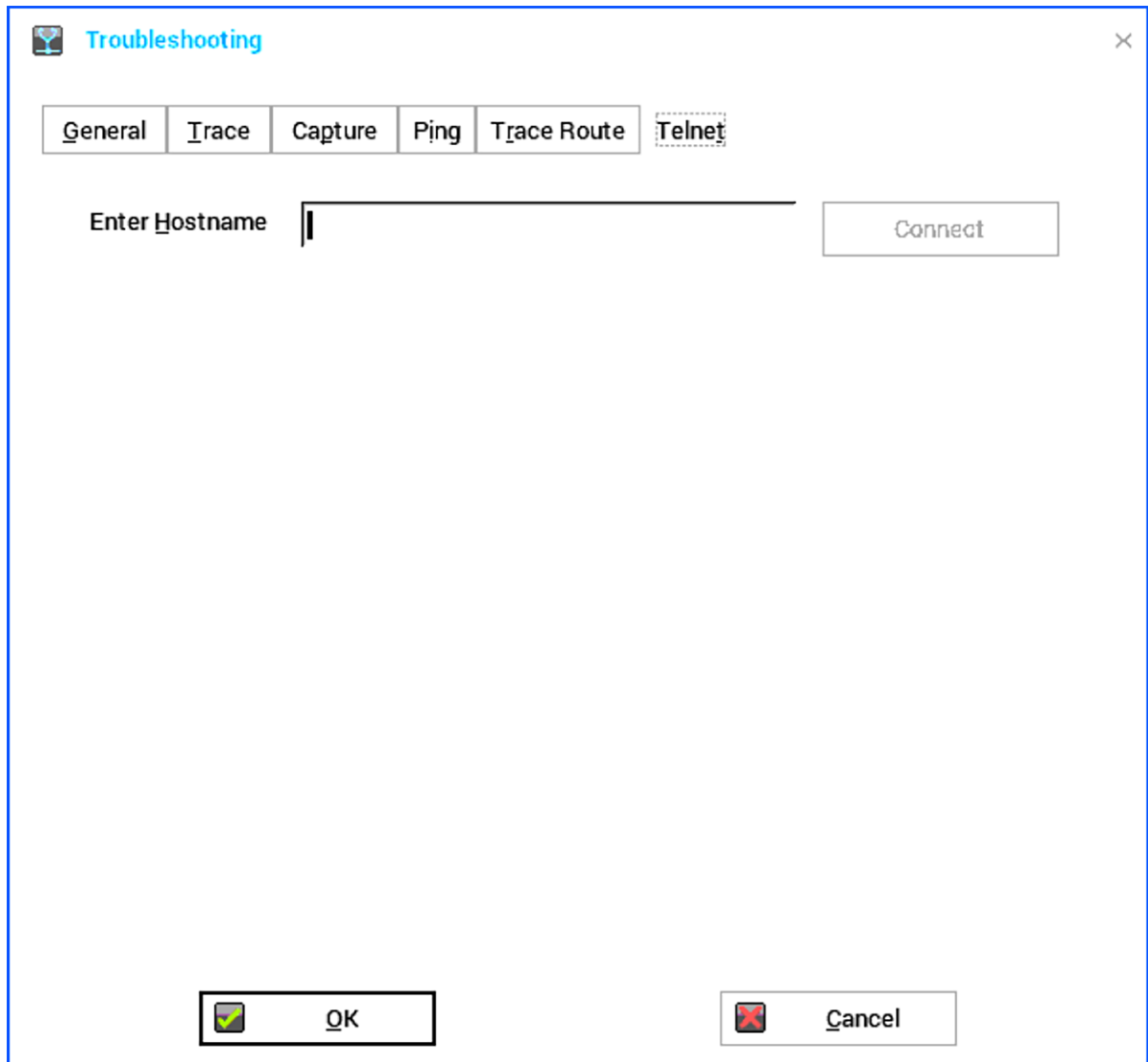
Figure 36. Telnet
