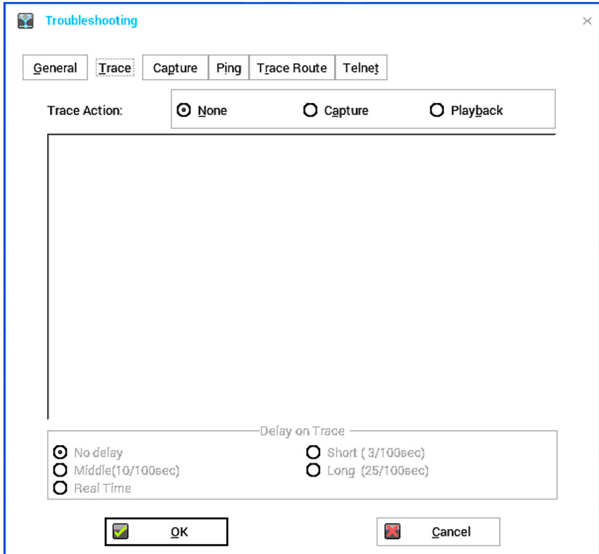
Figure 32. Trace
