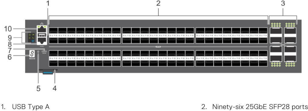
The S5296F-ON switch I/O-side view:
