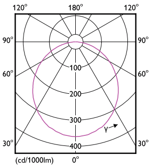
Light Distribution Diagram - 59469 MESON 175 20W 40K WH recessed
