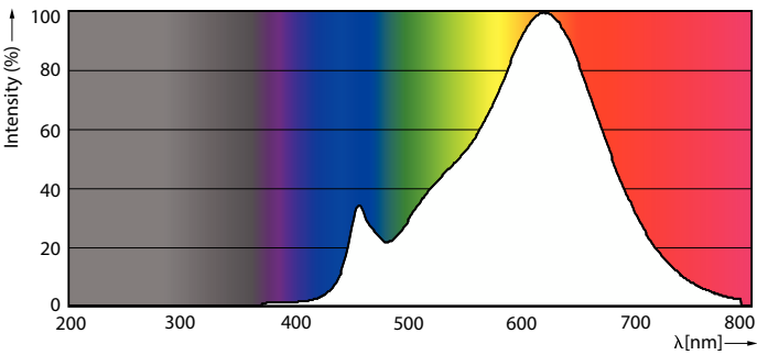
Spectral Power Distribution Colour - 5.5BA11/PER/927-922/CL/G/E26/WGX 1FB T20
