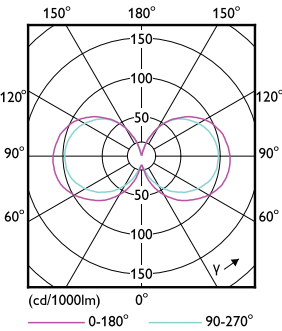
Light Distribution Diagram - 5.5BA11/PER/927-922/CL/G/E26/WGX 1FB T20
