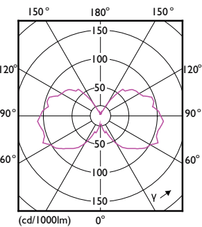
Light Distribution Diagram - 4.5A19/VIN/820/E26/CL/GL/DIM 4/FBH T20
