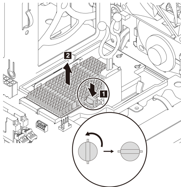
Figure 133. Removing the heat sink from the M.2 solid-state drive holder
