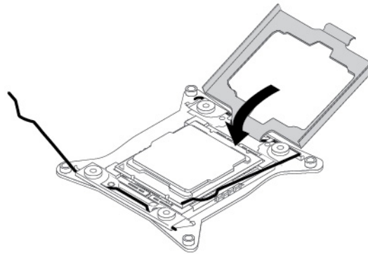
Figure 167. Closing the microprocessor retainer
