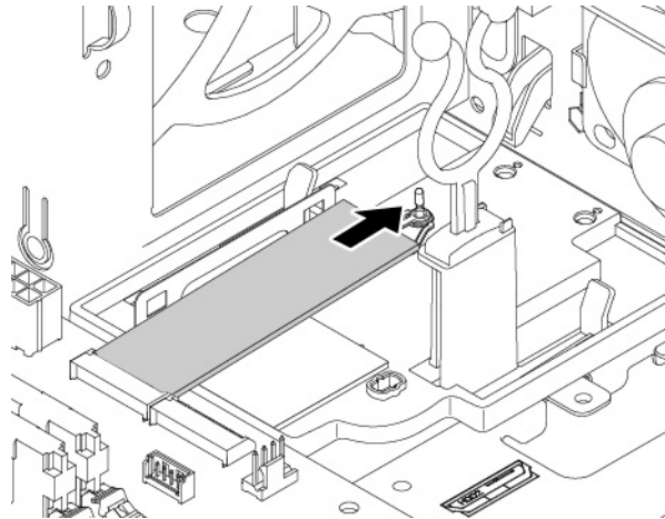
Figure 135. Removing the M.2 solid-state drive
