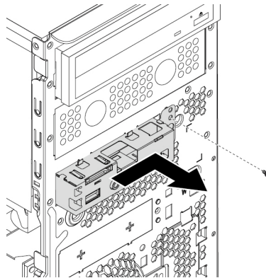
Figure 146. Removing the front audio and USB assembly
