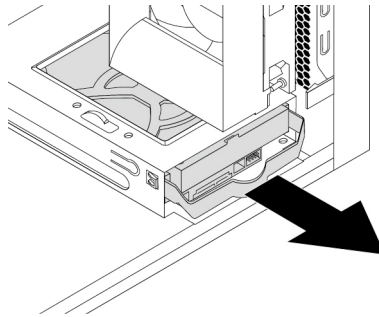
Figure 85. Removing the secondary storage drive
