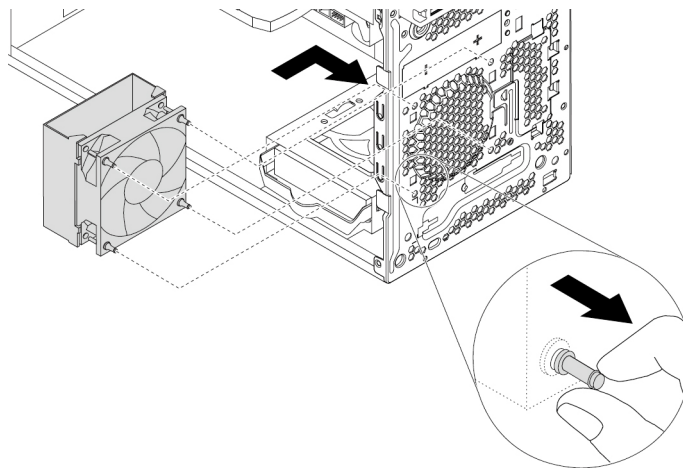
Figure 93. Installing the front fan assembly
