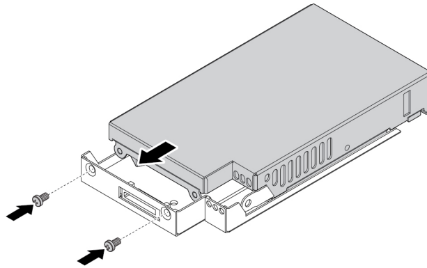
Figure 130. Installing the cover of the M.2 solid-state drive carrier
