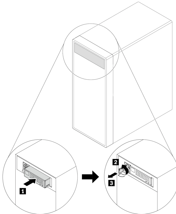
Figure 131. Reinstalling the M.2 solid-state drive carrier
