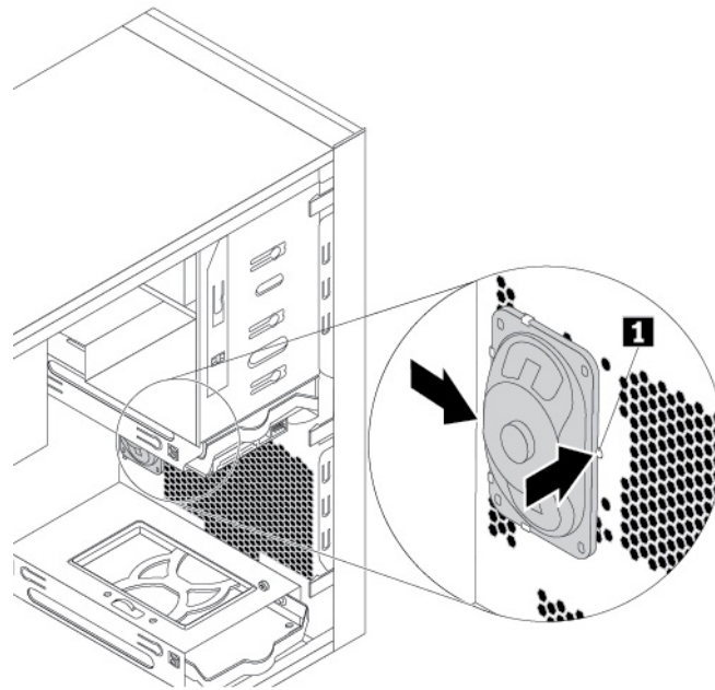
Figure 144. Removing the old internal speaker
