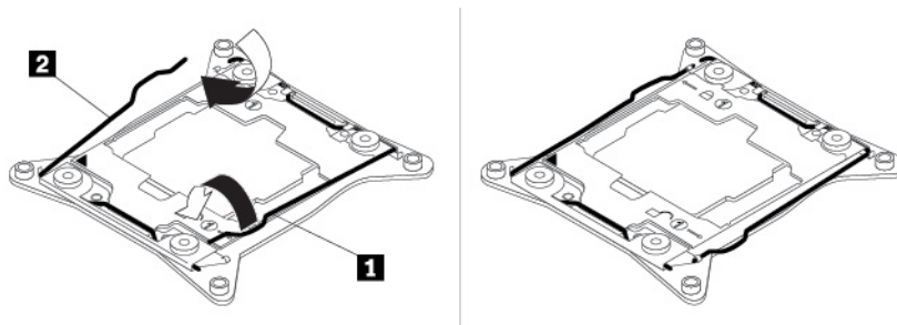
Figure 168. Securing the microprocessor in the socket
