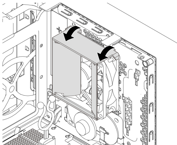
Figure 132. Removing the cover of the front fan assembly
