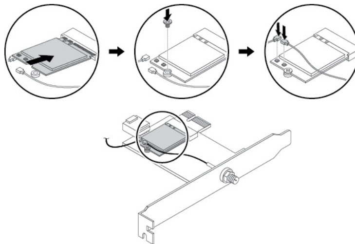
Figure 161. Installing the Wi-Fi antenna cables
