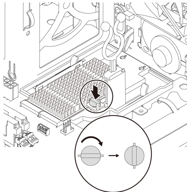
Figure 141. Securing the heat sink to the M.2 solid-state drive holder
