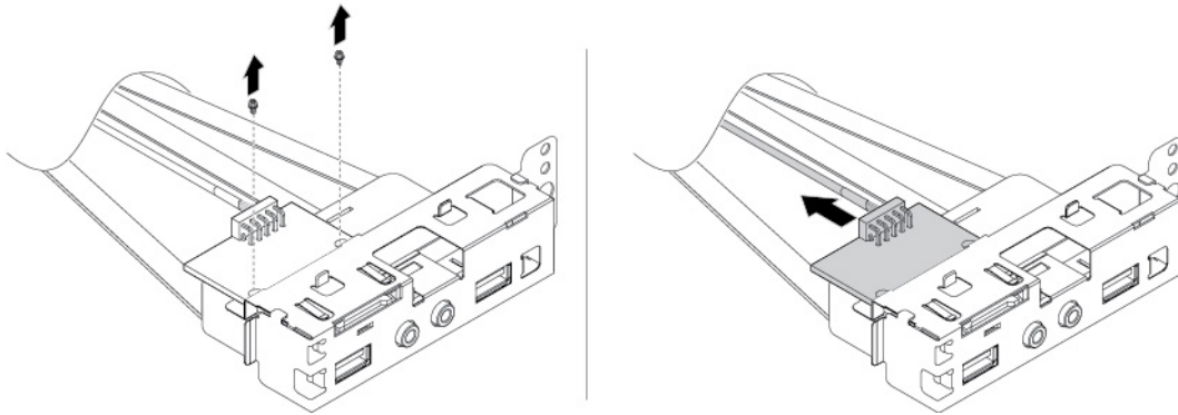
Figure 148. Removing the card reader
