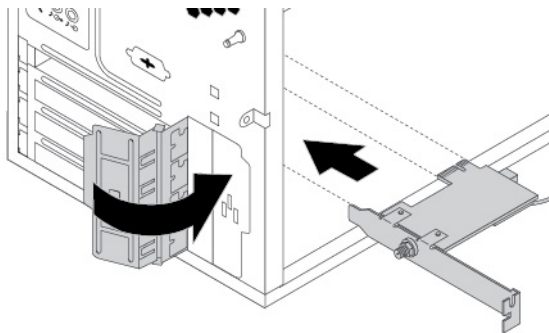
Figure 159. Installing the Wi-Fi adapter card
