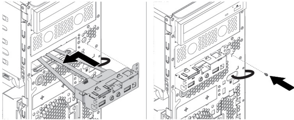
Figure 147. Installing the front audio and USB assembly
