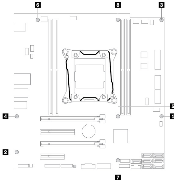
Figure 169. Removing the eight screws that secure the system board
