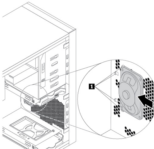
Figure 145. Installing the internal speaker
