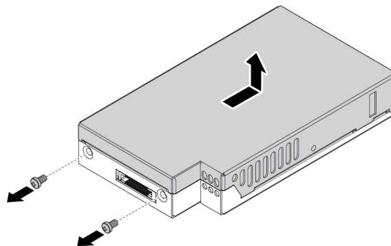
Figure 127. Removing the cover of the M.2 solid-state drive carrier
