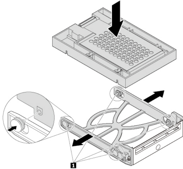
Figure 50. Installing the converter with the 2.5-inch storage drive into the plastic bracket
