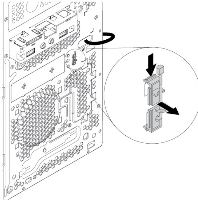
Figure 142. Removing the thermal sensor
