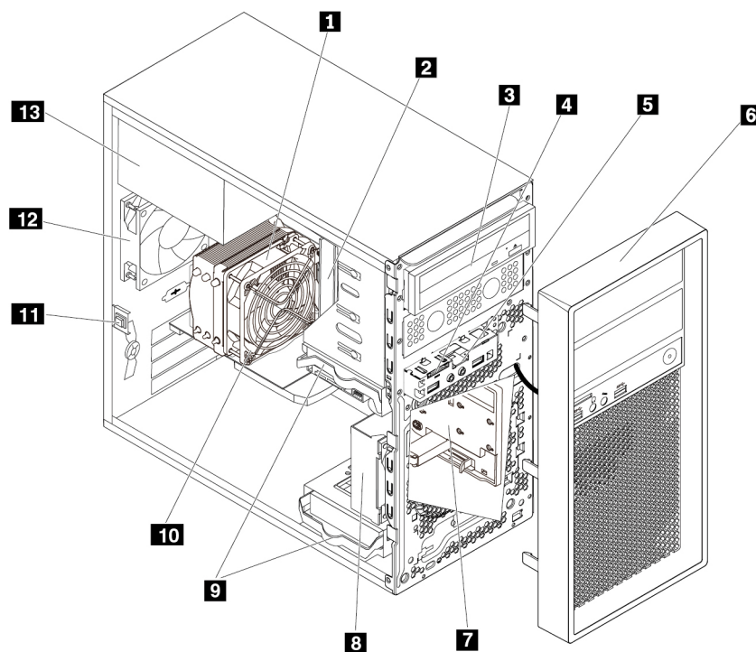
Figure 3. Component locations
