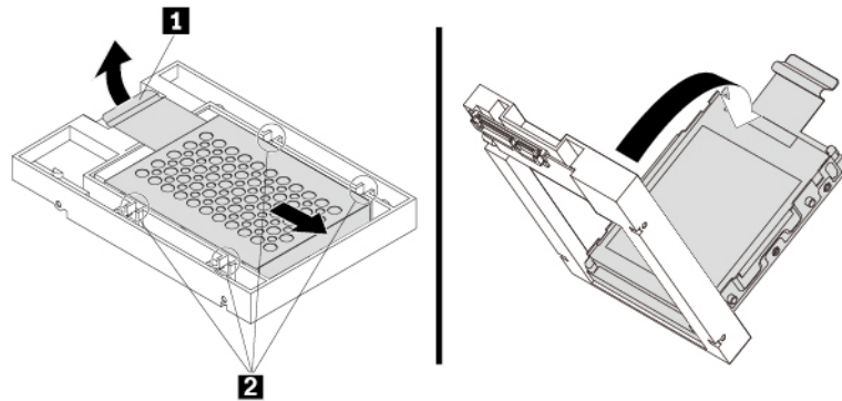
Figure 46. Removing the adapter from the converter
