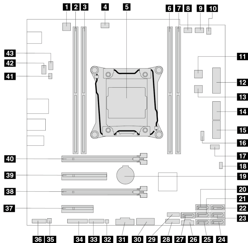
Figure 8. System board part locations
