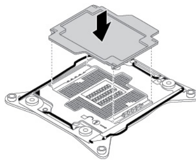
Figure 173. Installing the microprocessor socket cover
