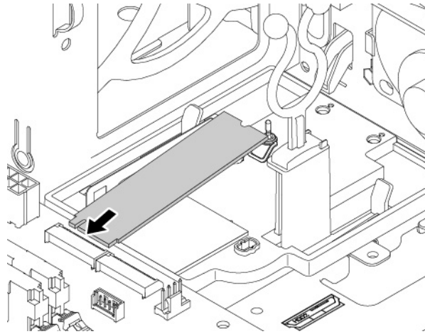
Figure 138. Installing the M.2 solid-state drive
