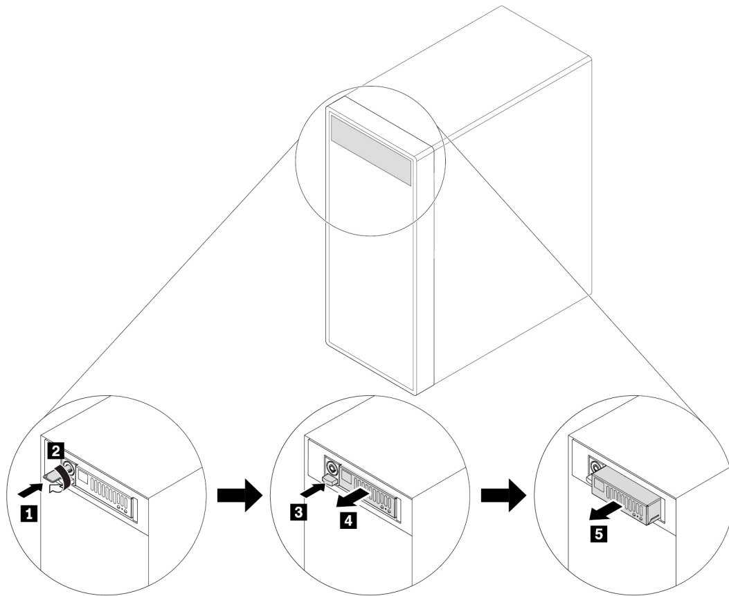
Figure 126. Removing the M.2 solid-state drive carrier
