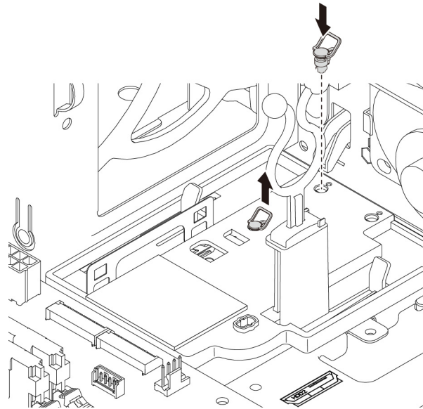
Figure 136. Adjusting the location of the retention latch on the M.2 solid-state drive holder
