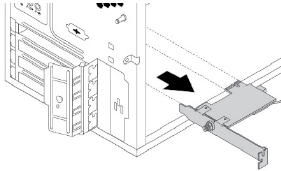
Figure 158. Removing the Wi-Fi adapter card
