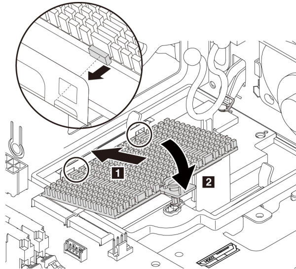
Figure 140. Installing the heat sink onto the M.2 solid-state drive holder
