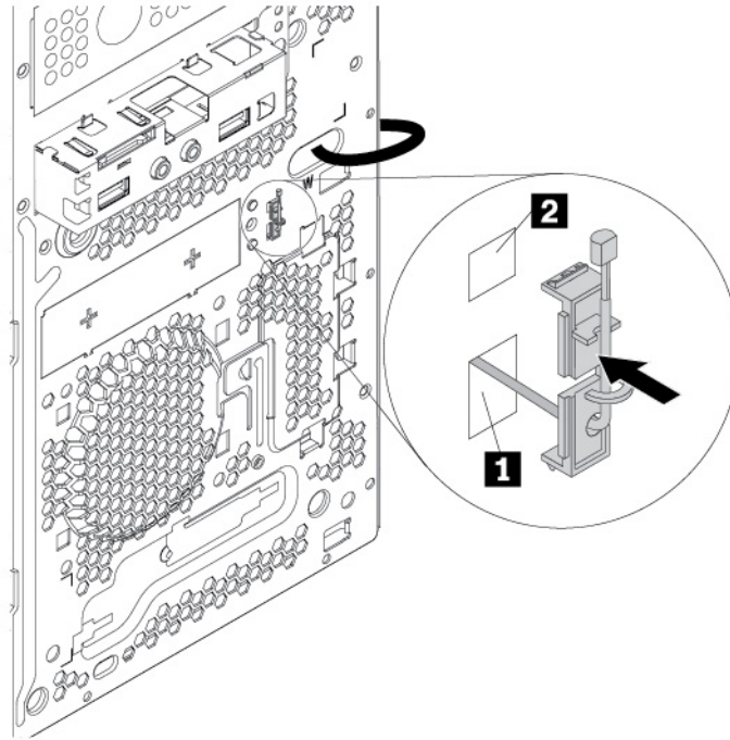
Figure 143. Installing the thermal sensor
