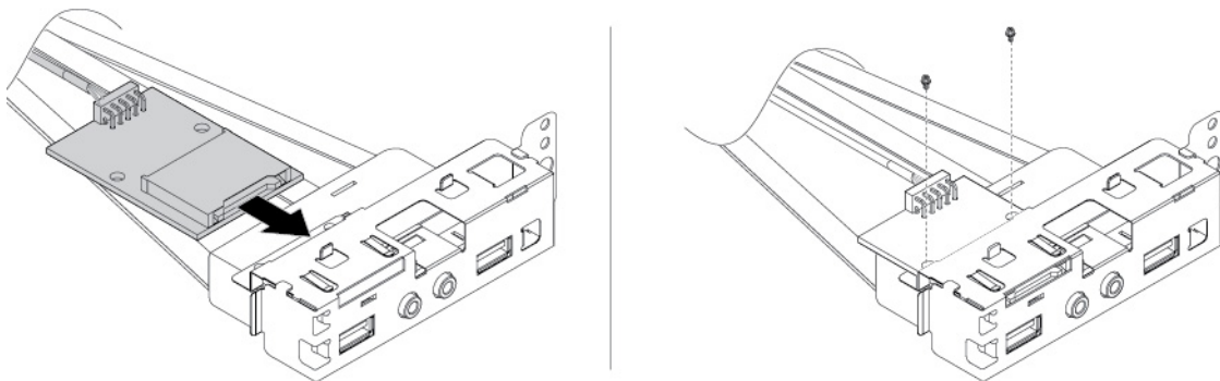
Figure 149. Installing the new card reader
