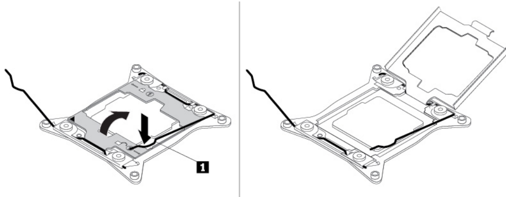
Figure 163. Opening the microprocessor retainer
