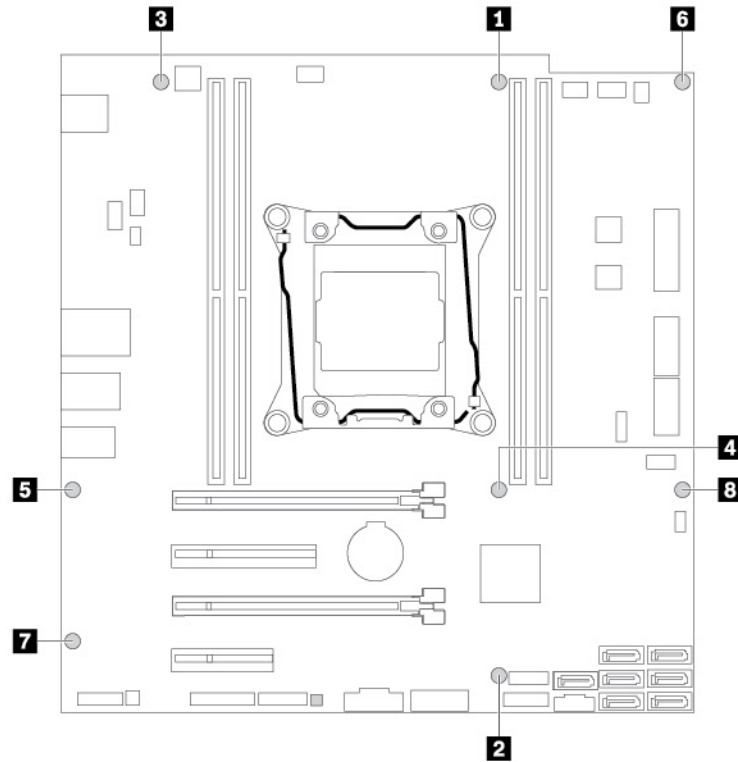
Figure 170. Installing the eight screws to secure the system board
