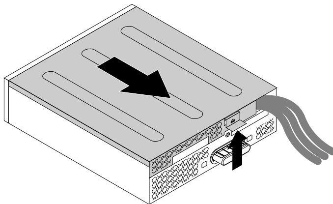
Figure 96. Removing the flex module cover
