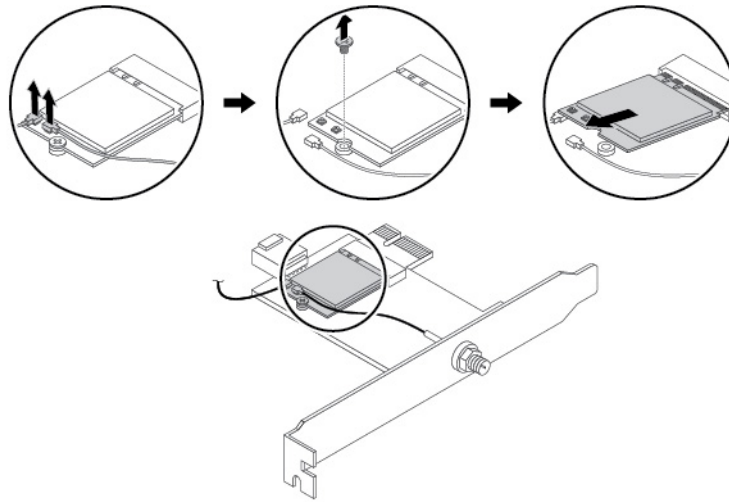
Figure 160. Removing the Wi-Fi card module
