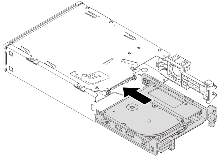
Figure 74. Installing the new 2.5-inch storage drive with bracket into the kit
