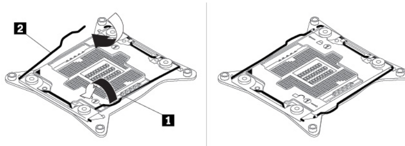
Figure 172. Securing the microprocessor in the socket
