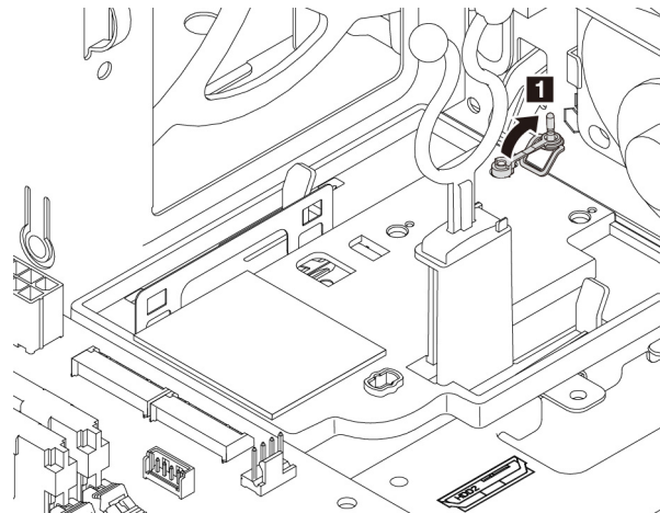
Figure 137. Pulling the handle of the retention latch
