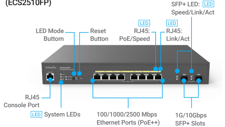
CloudSwitch MGPlus 8 Full PoE (ECS2510FP)
