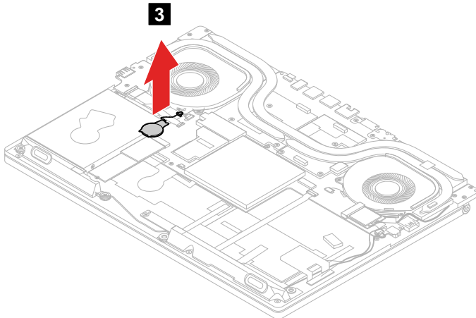
Figure 10. Remove the coin-cell battery
