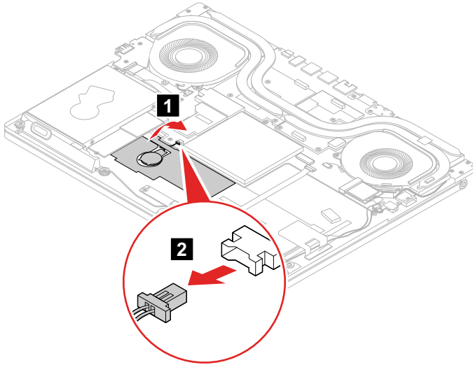
Figure 9. Lift the aluminum foil and detach the connector
