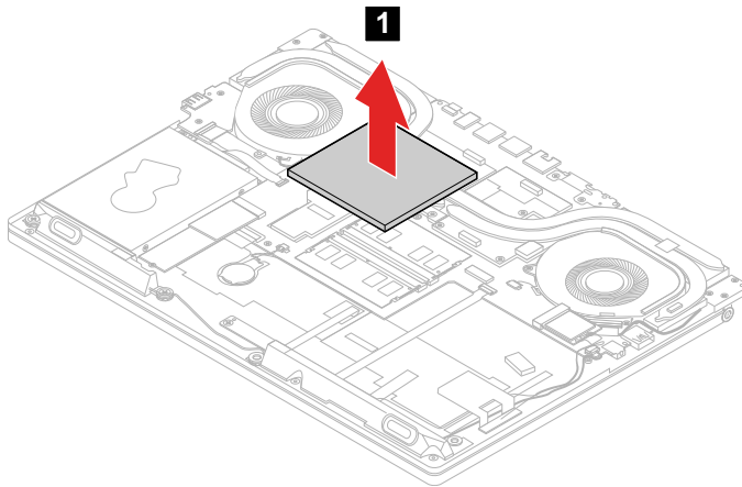
Figure 20. Remove the memory module shielding
