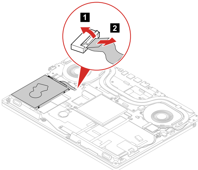
Figure 15. Detach the HDD cable connector
