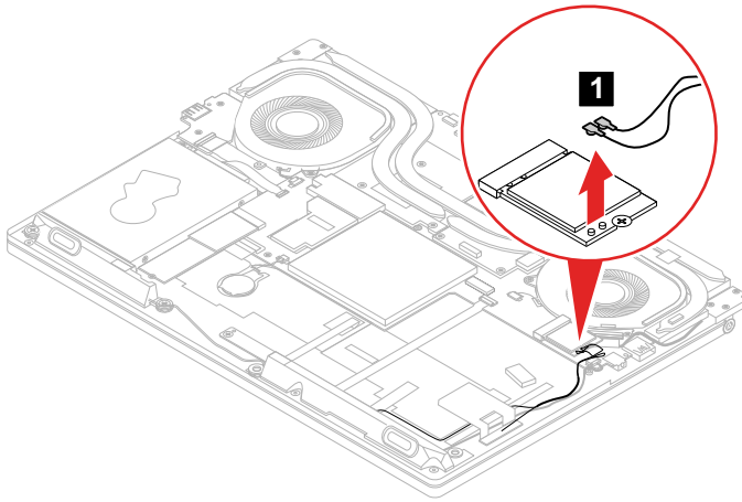
Figure 22. Detach the connectors
