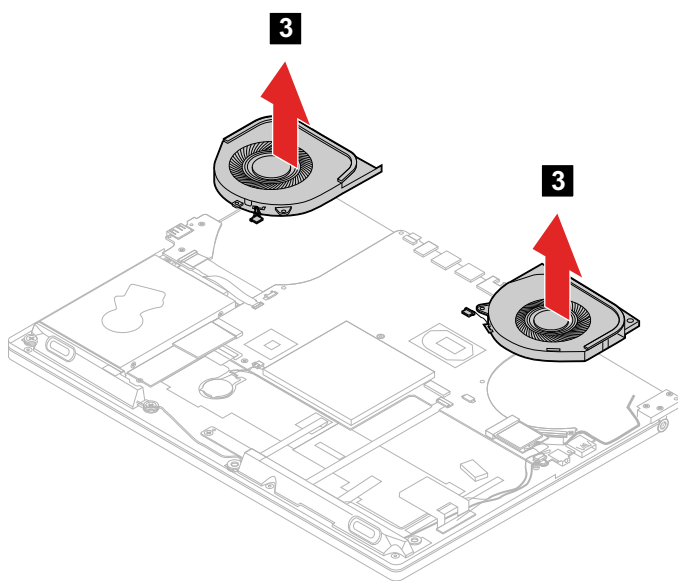
Figure 29. Remove the 2 fans
