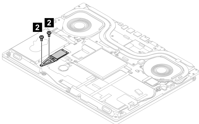
Figure 12. Remove the 2 screws (for 2242)
