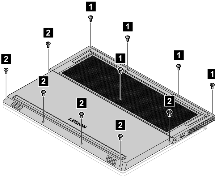
Figure 3. Remove the 11 screws
