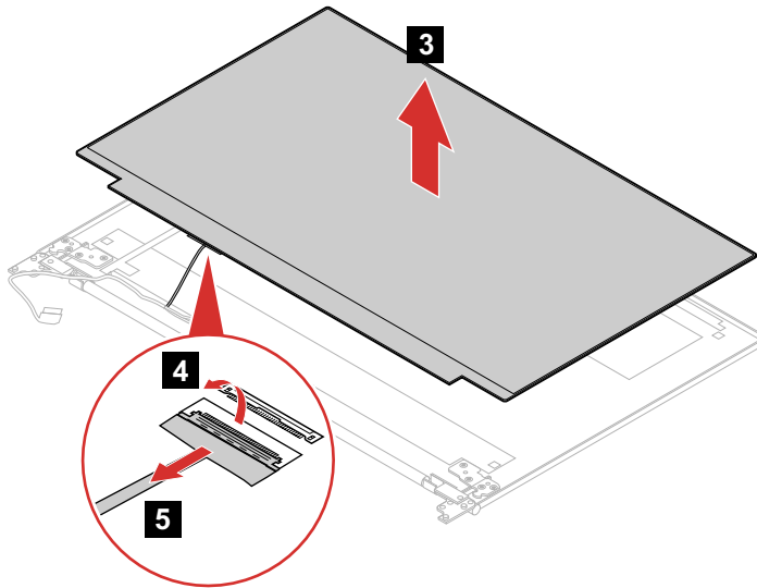
Figure 46. Detach EDP cable connector
