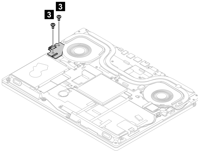
Figure 31. Remove the 2 screws
