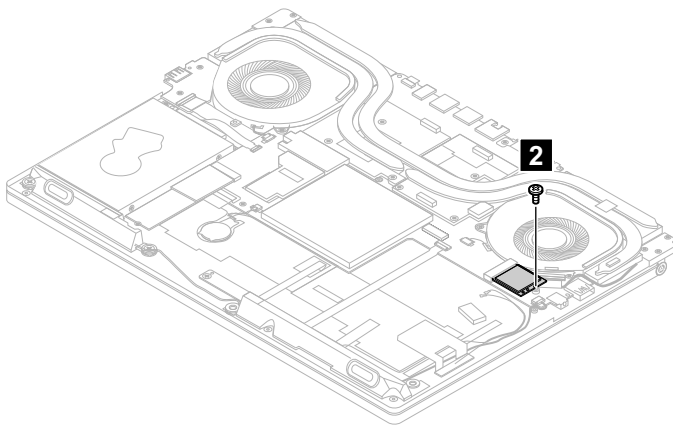
Figure 23. Remove 1 screw
