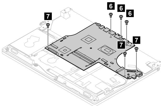
Figure 37. Remove the 6 screws
