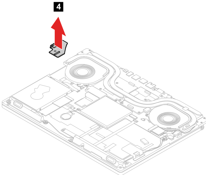
Figure 32. Remove the I/O board
