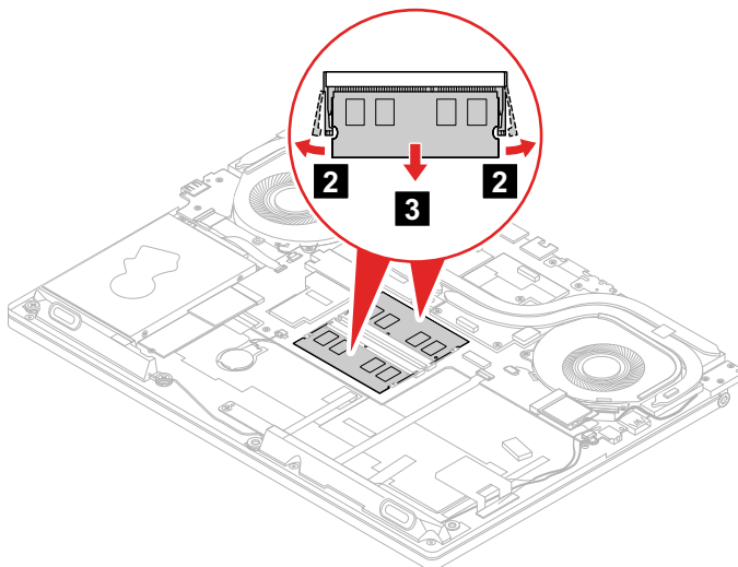
Figure 21. Remove the memory modules
