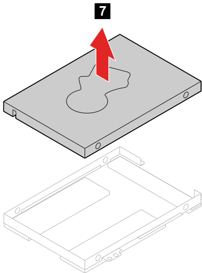
Figure 19. Separate HDD from its bracket
