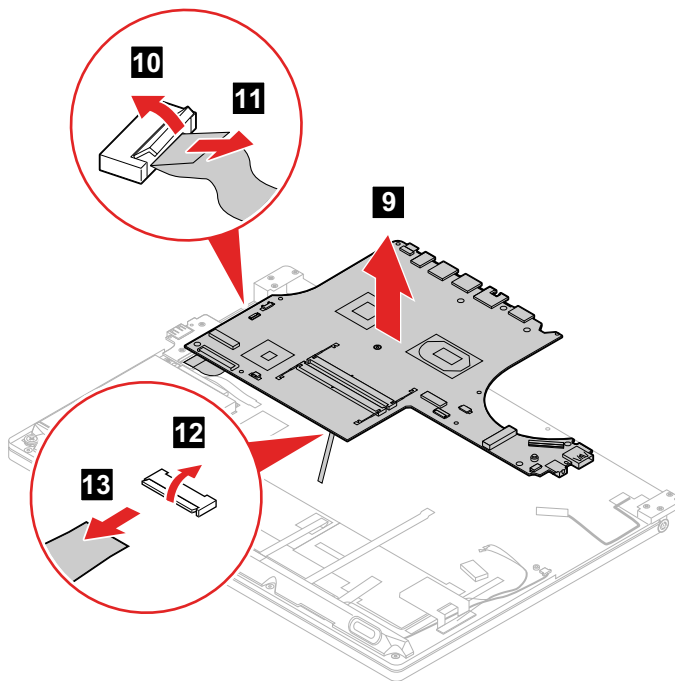
Figure 39. Remove the system board
