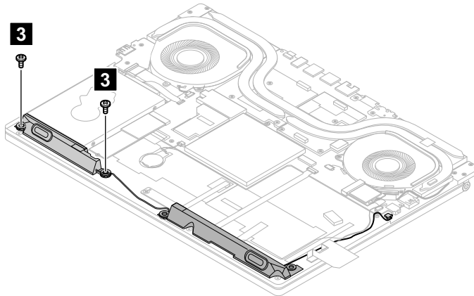
Figure 34. Remove the 2 screws
