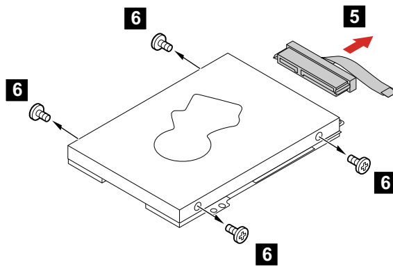
Figure 18. Remove the HDD cable and 4 screws
