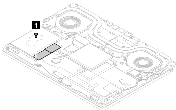
Figure 11. Remove 1 screw (for 2280)
