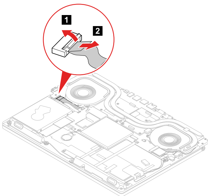
Figure 30. Detach the I/O board connector
