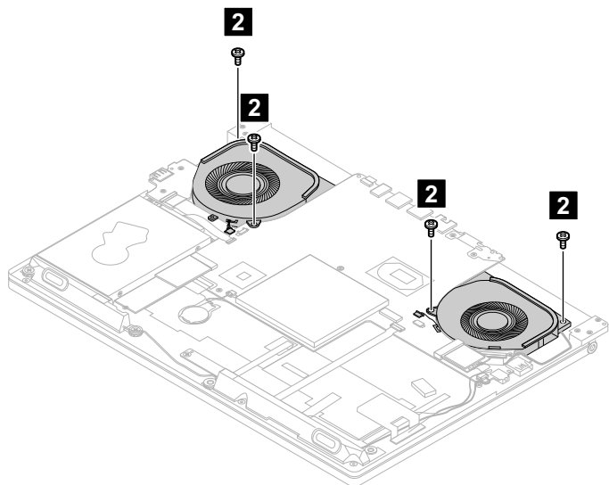
Figure 28. Remove the 4 screws
