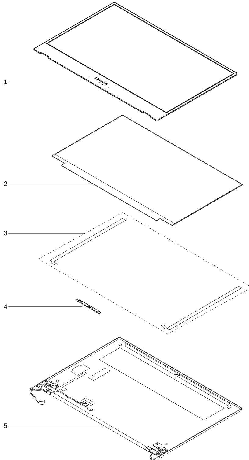
Figure 2. LCD module – exploded view
