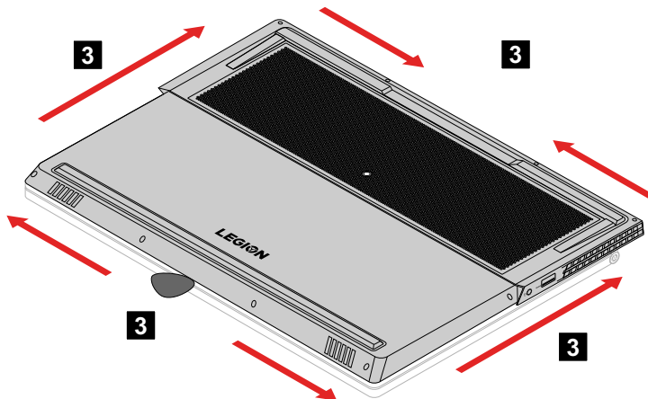
Figure 4. Separate the lower case from upper case
