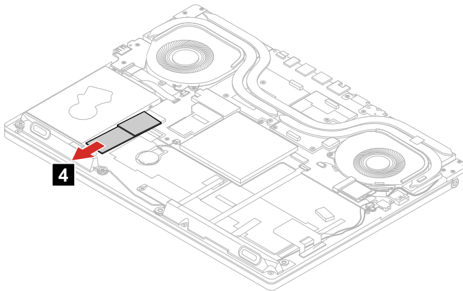
Figure 14. Remove the SSD
