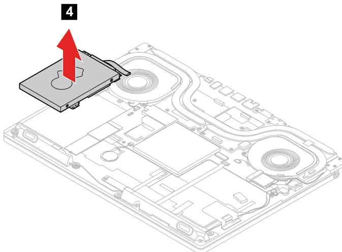
Figure 17. Remove the HDD assembly
