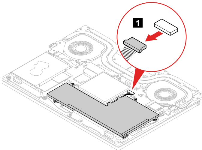
Figure 6. Detach the battery pack connector
