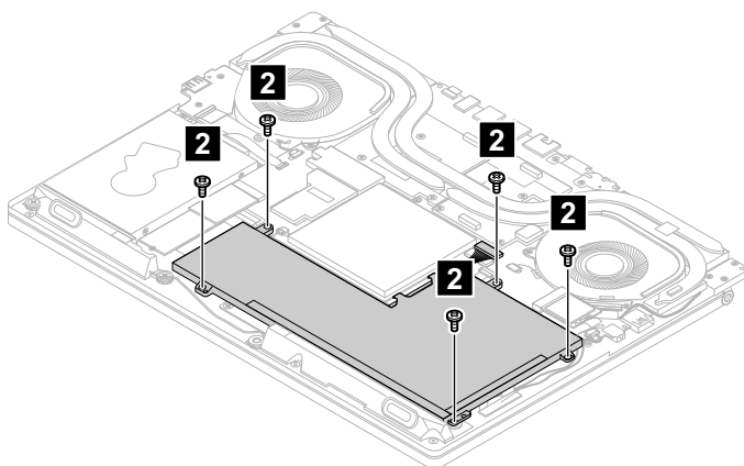
Figure 7. Remove the 5 screws
