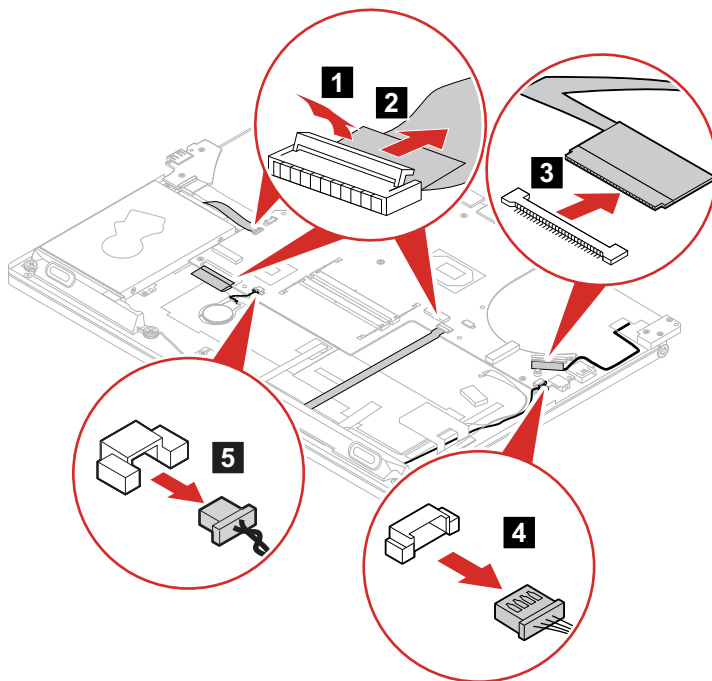
Figure 36. Detach the 6 connectors
