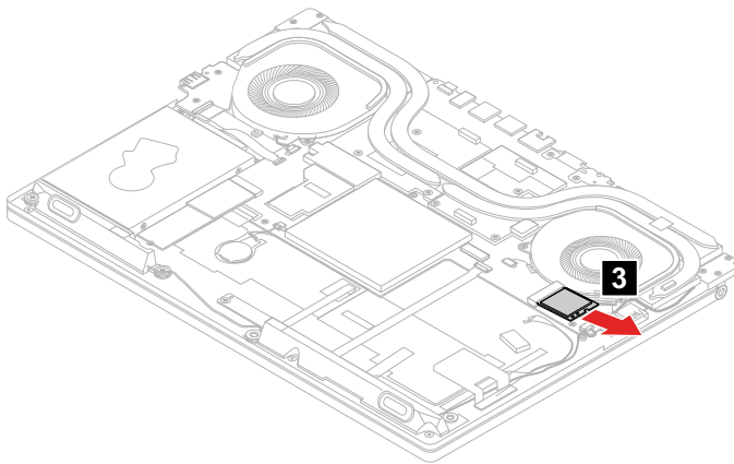
Figure 24. Remove the Wi-Fi card
