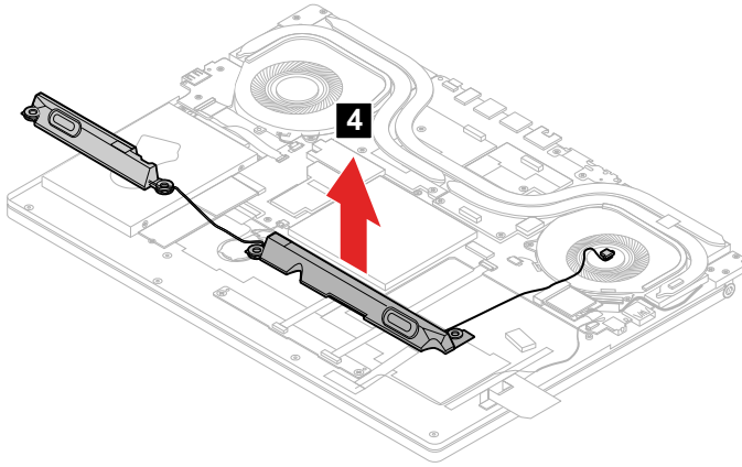
Figure 35. Remove the speakers
