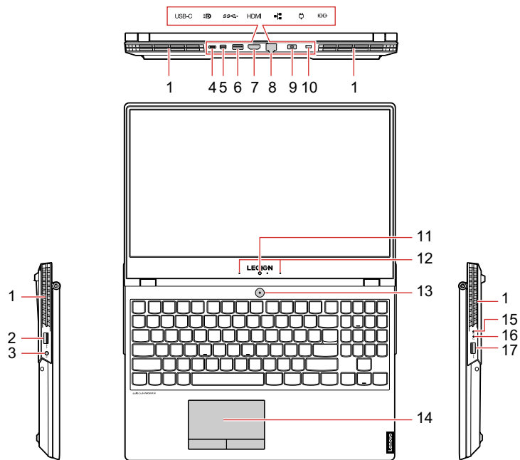
Figure 49. Features and connectors
