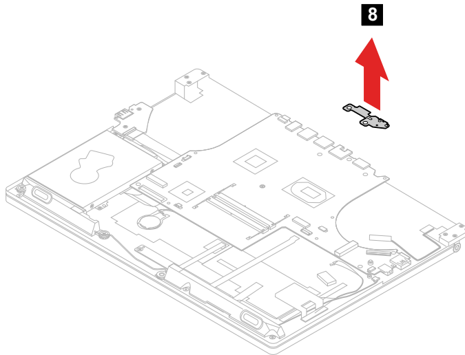
Figure 38. Remove the key-lock bracket
