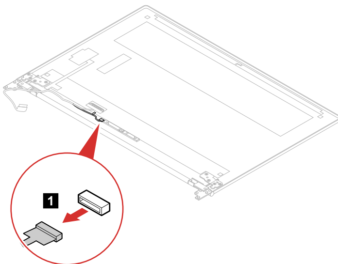
Figure 47. Detach the camera connector
