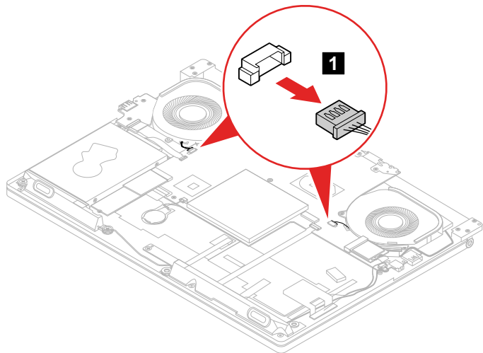
Figure 27. Detach the 2 connectors
