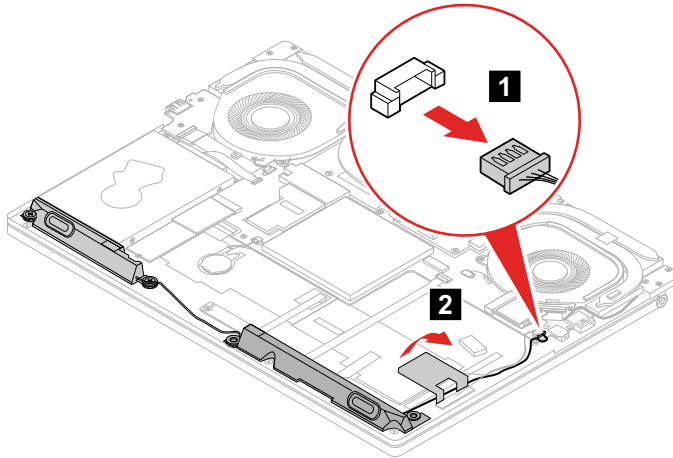
Figure 33. Detach the speaker connector and peel off the aluminum foil
