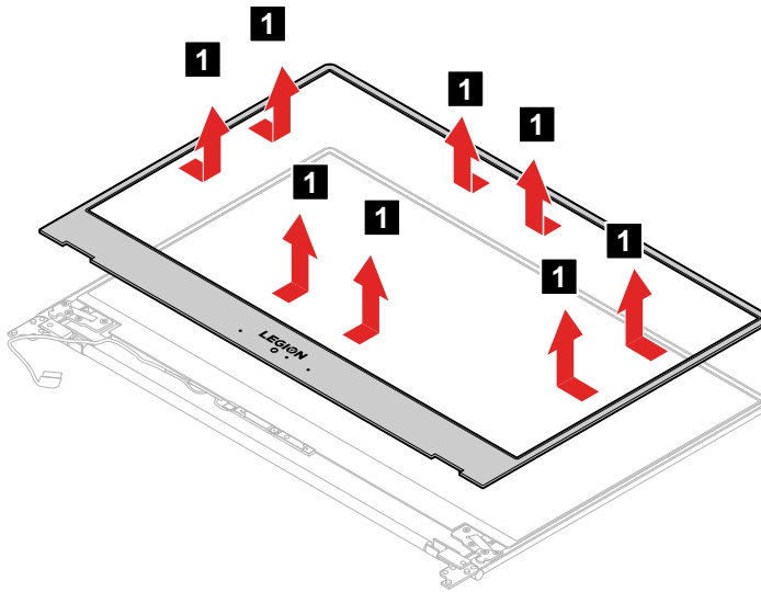
Figure 44. Pull the inner sides of the LCD bezel
