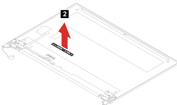
Figure 48. Remove the camera board
