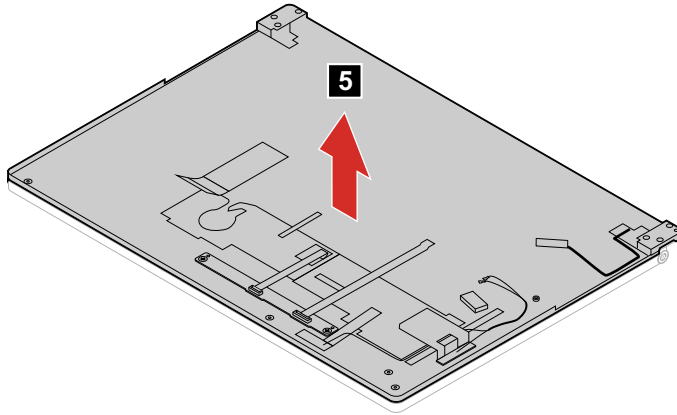
Figure 43. Remove the upper case
