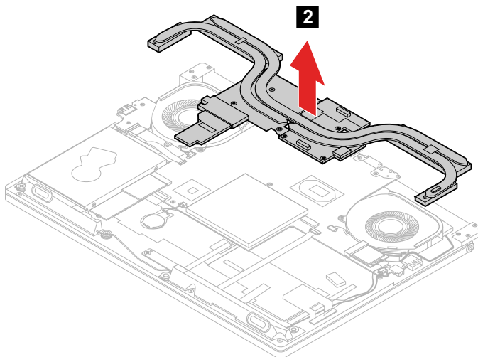
Figure 26. Remove the heat sink
