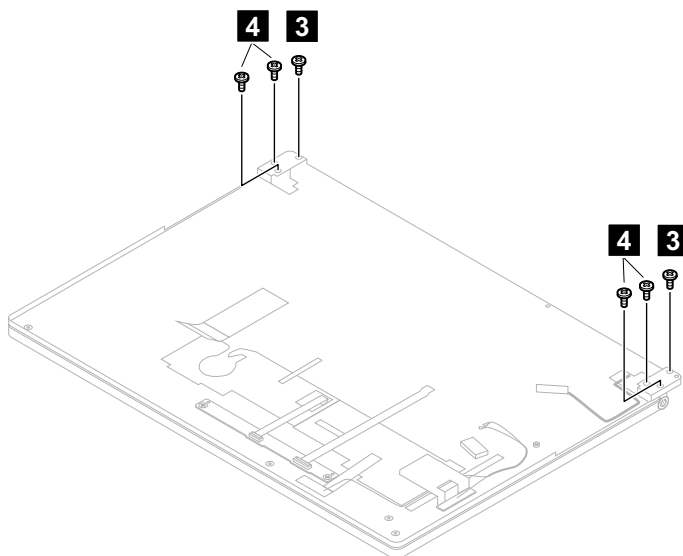
Figure 42. Remove the 6 screws
