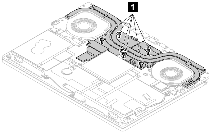
Figure 25. Loosen the 6 screws
