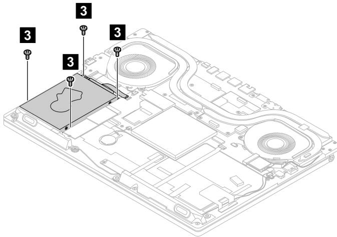
Figure 16. Remove the 4 screws
