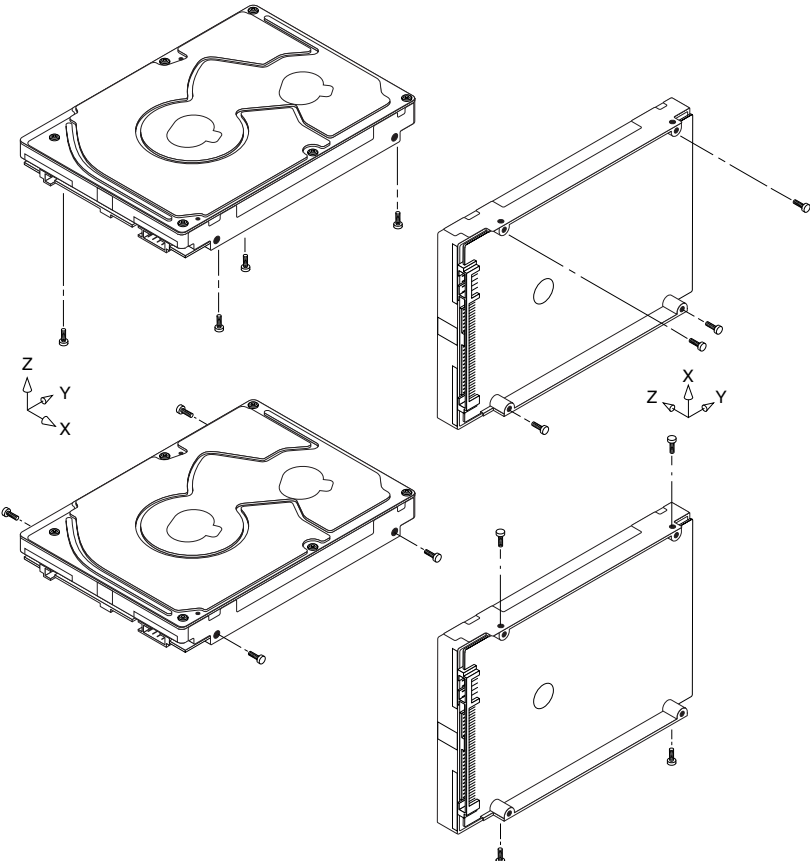
Figure 6. Recommended mounting
