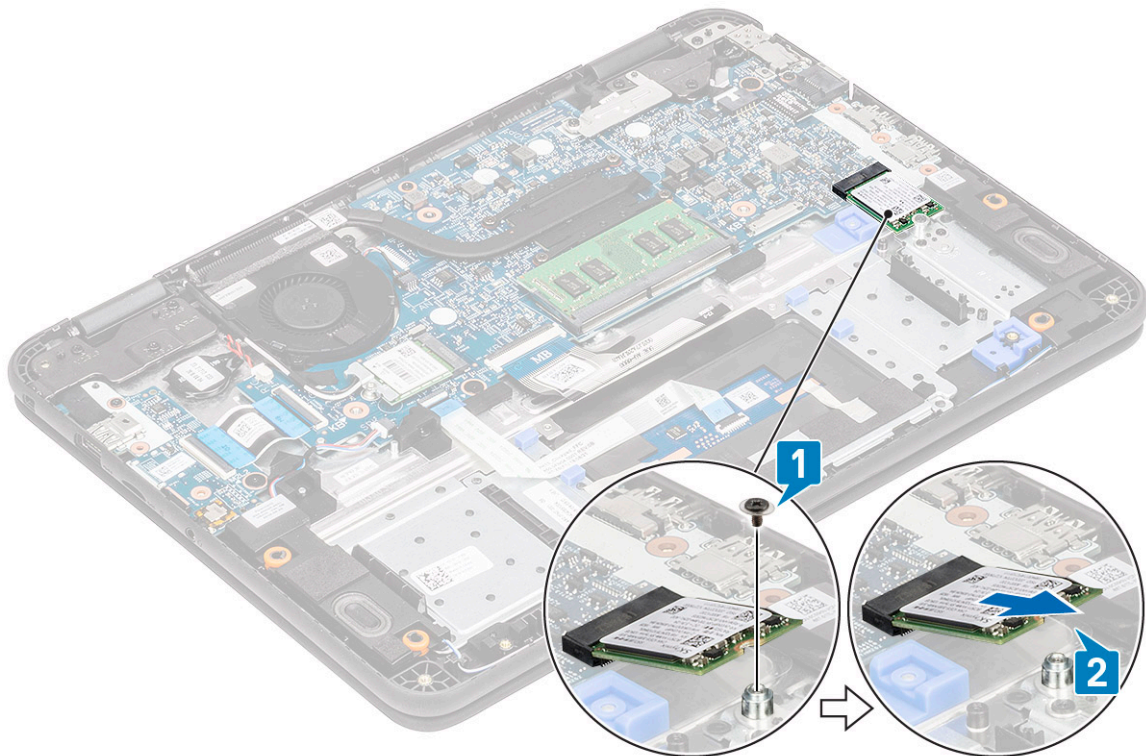
Figure 11. M.2 2230 SSD
