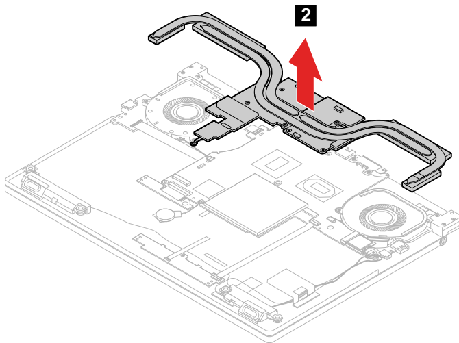
Figure 29. Remove the heat sink
