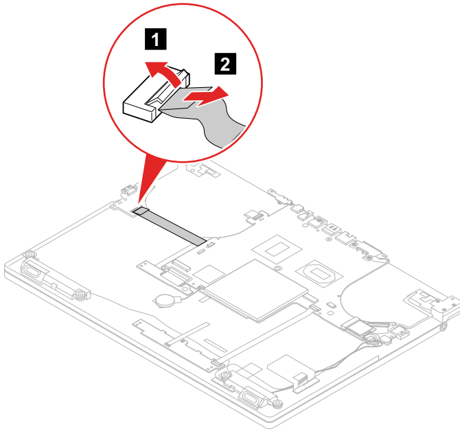
Figure 33. Detach the I/O board connector
