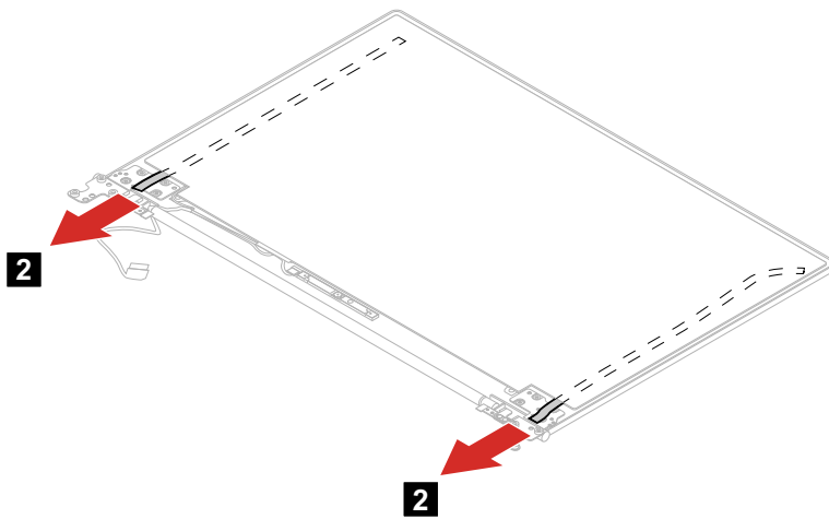
Figure 52. Remove the removable tapes
