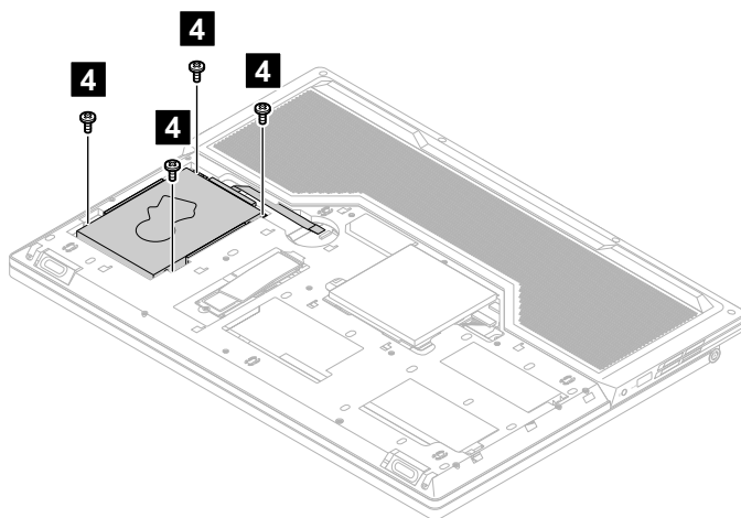
Figure 11. Remove the 4 screws
