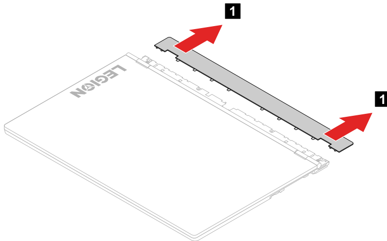
Figure 47. Remove the strip cover
