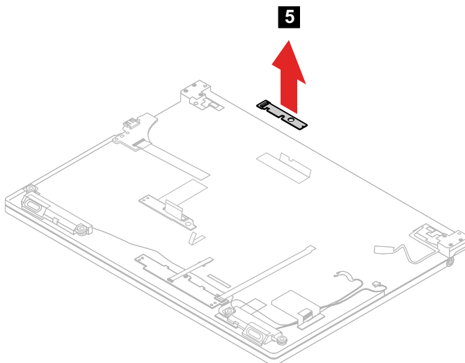
Figure 46. Remove the touchpad board
