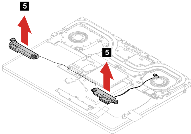
Figure 37. Remove the speakers
