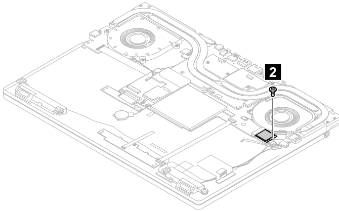
Figure 26. Remove 1 screw
