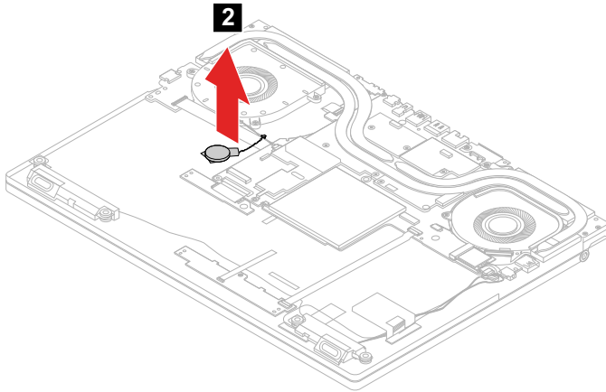
Figure 22. Remove the coin-cell battery
