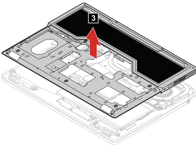
Figure 17. Remove the lower case
