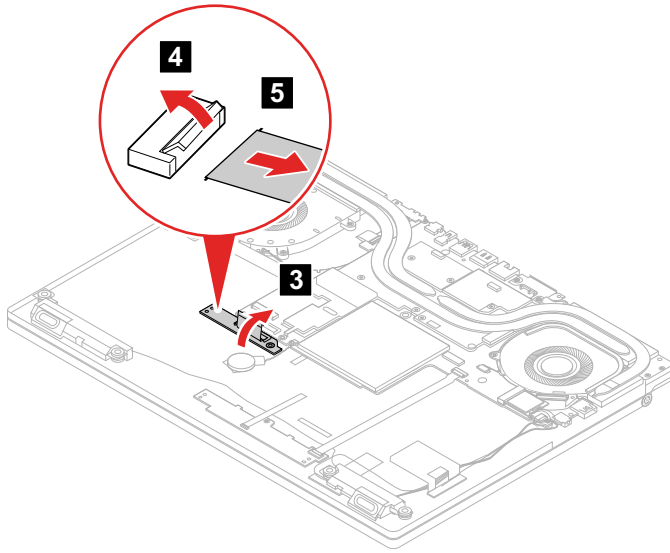
Figure 39. Remove the keyboard transfer board
