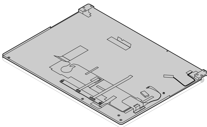
Figure 50. Remove the upper case
