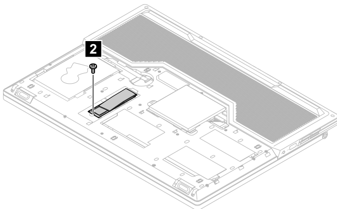
Figure 6. Remove 1 screw (for 2280)
