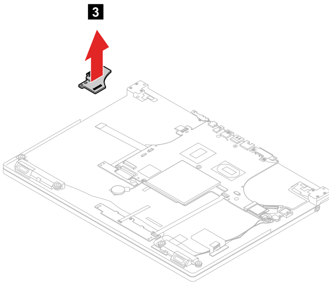
Figure 34. Remove the I/O board
