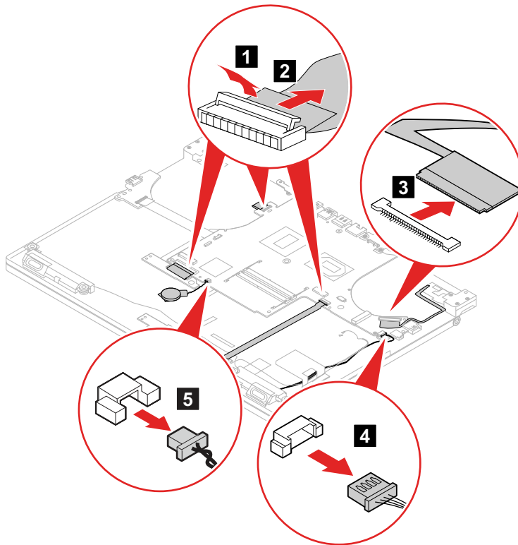
Figure 40. Detach the 6 connectors
