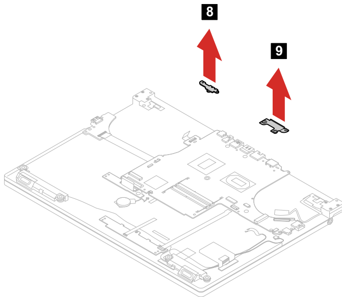
Figure 42. Remove the key-lock bracket and the DC-in bracket
