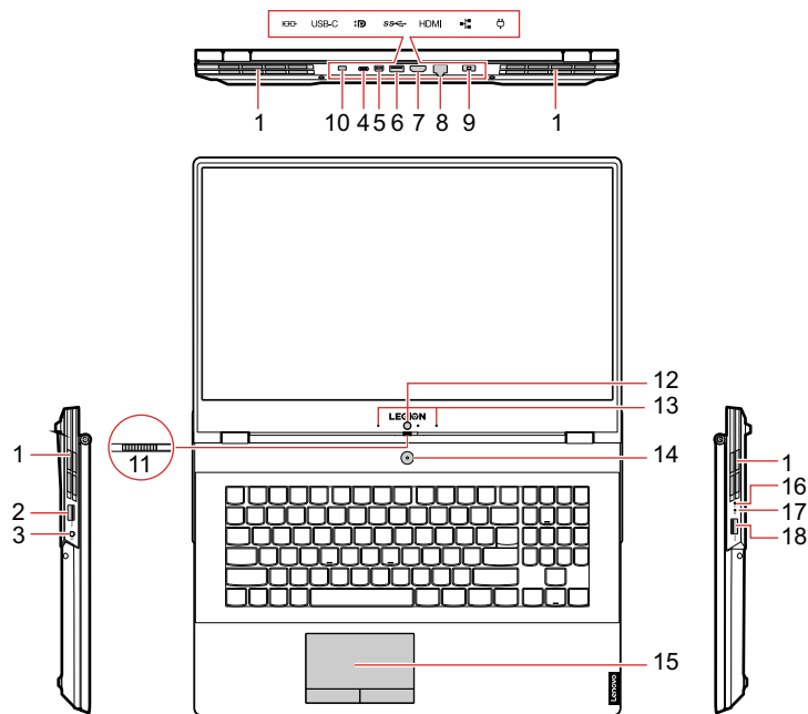
Figure 56. Features and connectors
