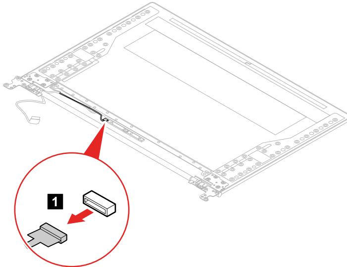
Figure 54. Detach the camera connector
