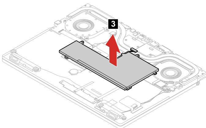
Figure 20. Remove the battery pack
