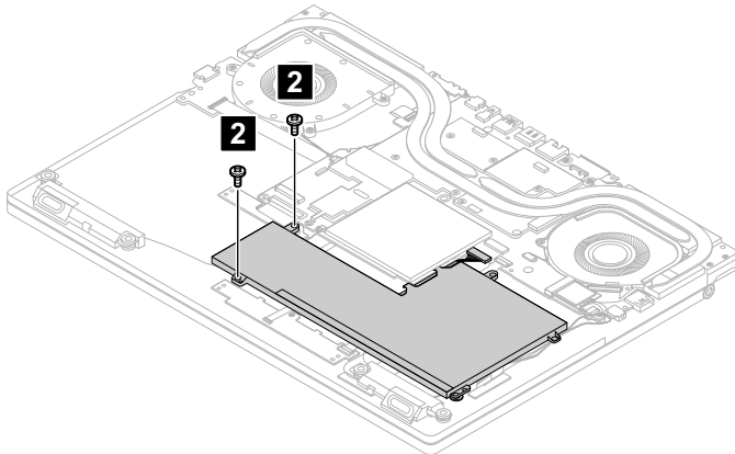
Figure 19. Remove the 2 screws
