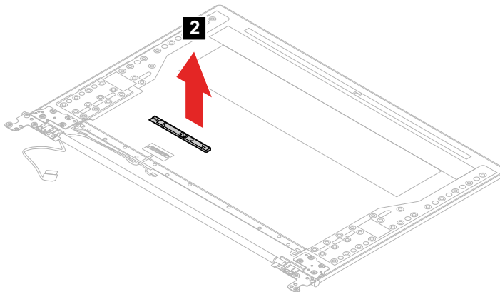
Figure 55. Remove the camera board
