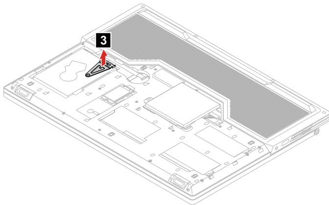
Figure 8. Remove the SSD bracket
