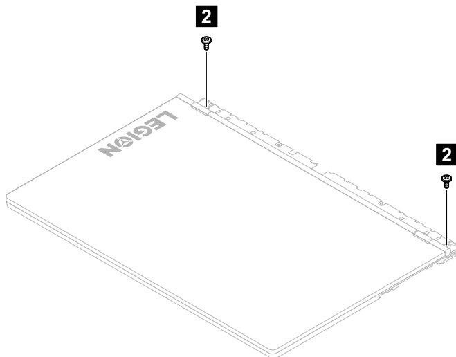
Figure 48. Remove the 2 screws
