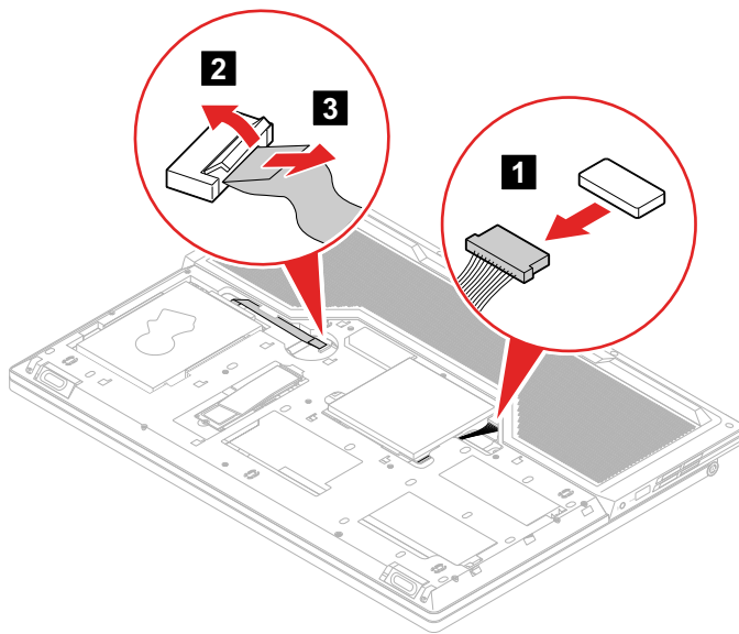
Figure 10. Detach the 2 connectors
