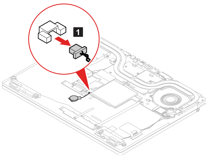
Figure 21. Detach the connector
