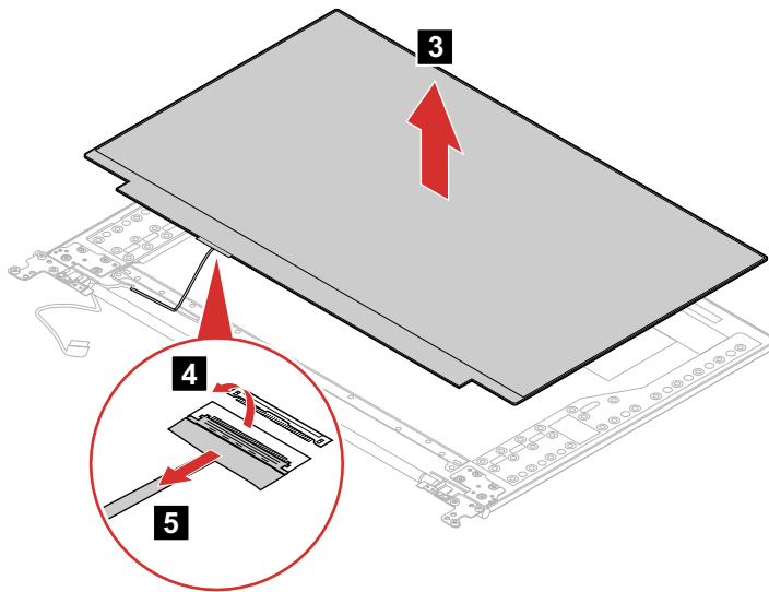
Figure 53. Detach EDP cable connector
