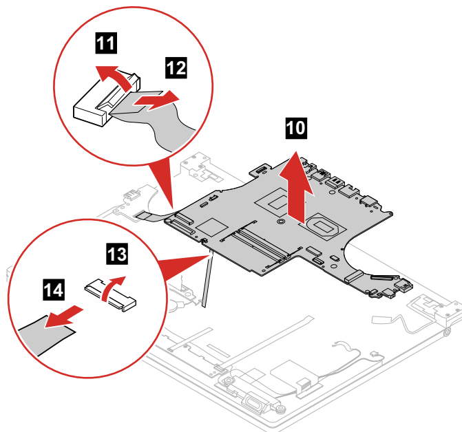
Figure 43. Remove the system board
