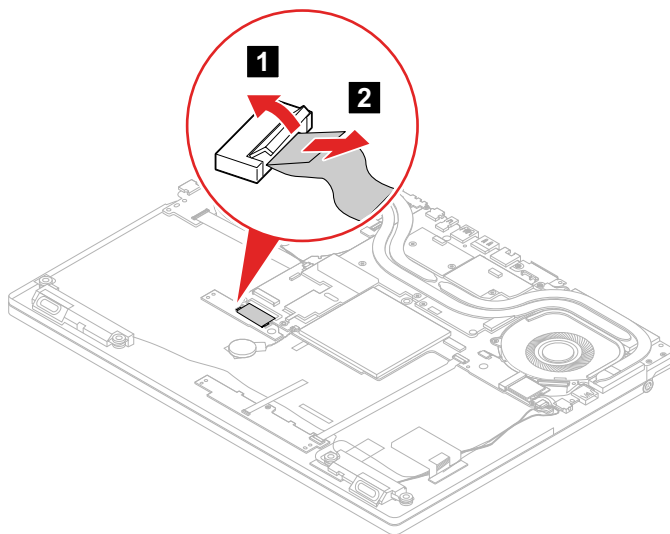
Figure 38. Detach 1 connector
