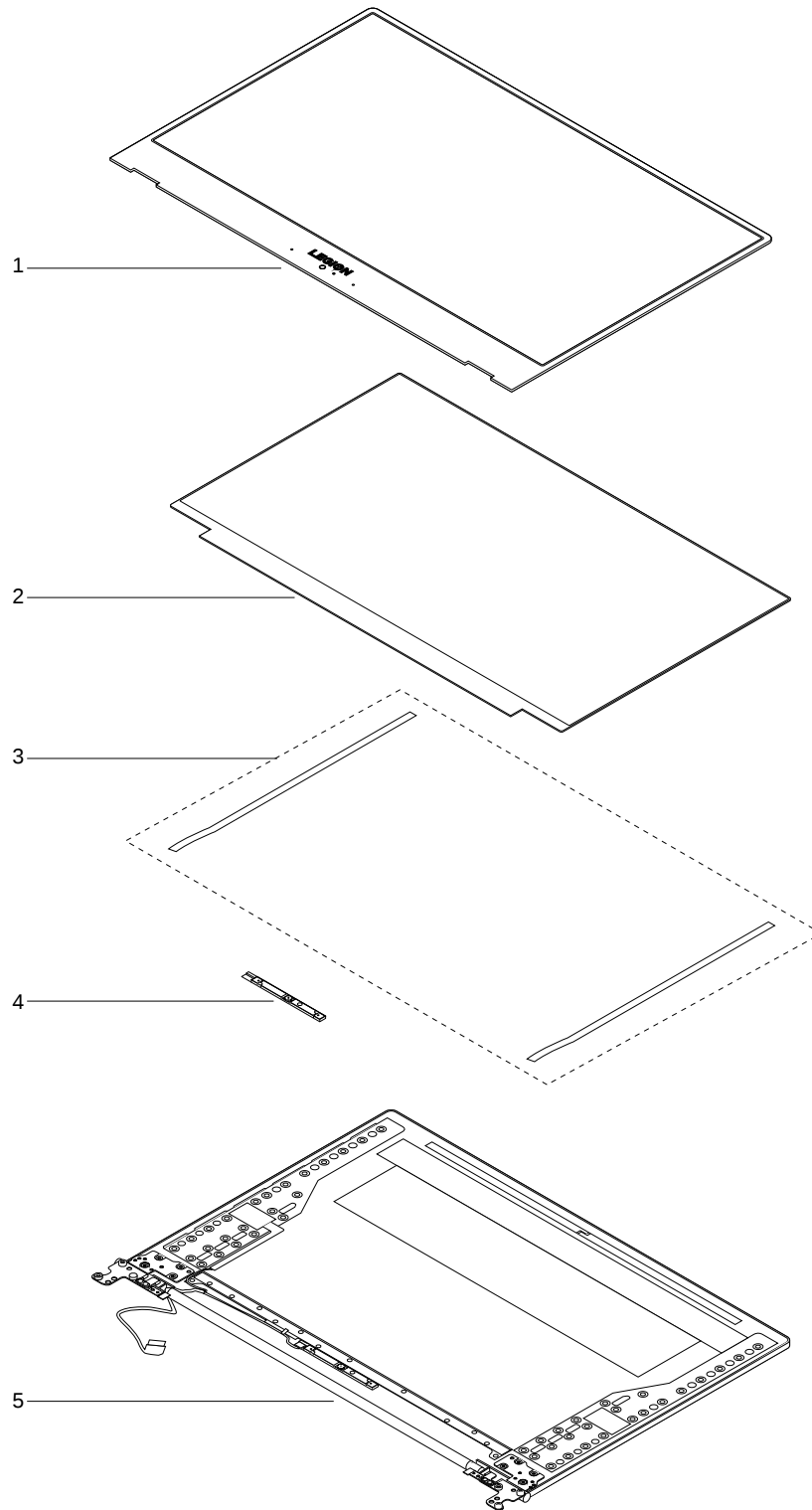
Figure 2. LCD module – exploded view
