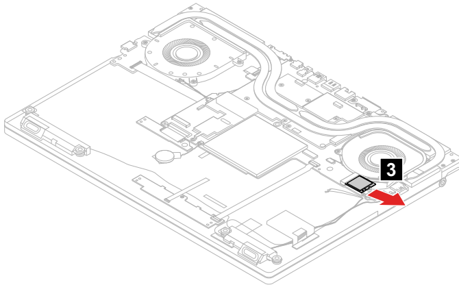
Figure 27. Remove the Wi-Fi card
