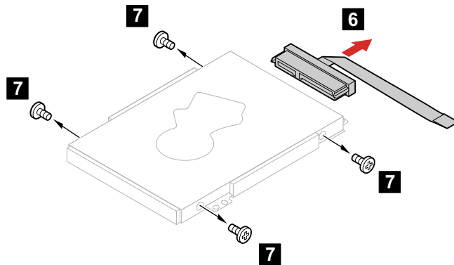
Figure 13. Remove the HDD cable and the 4 screws
