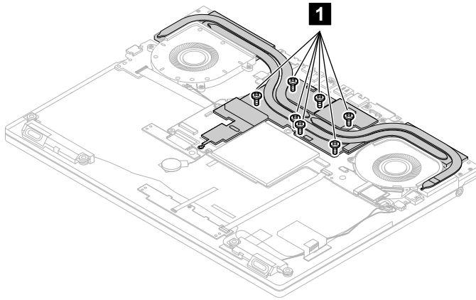
Figure 28. Loosen the 7 screws
