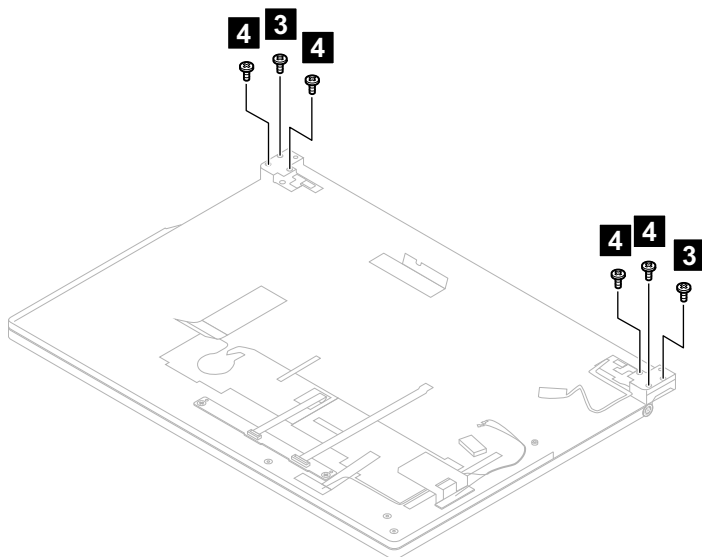
Figure 49. Remove the 6 screws
