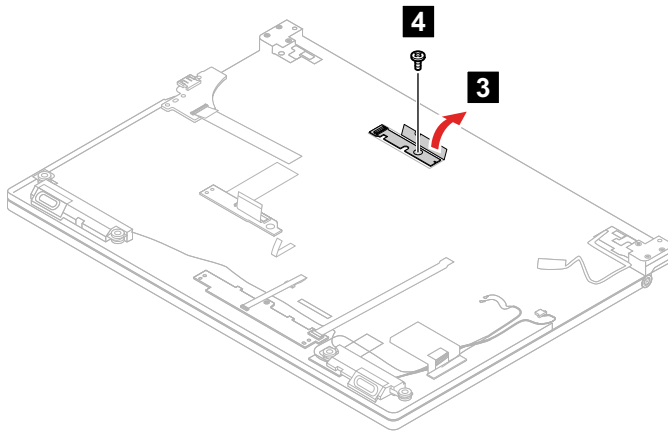
Figure 45. Remove 1 screw
