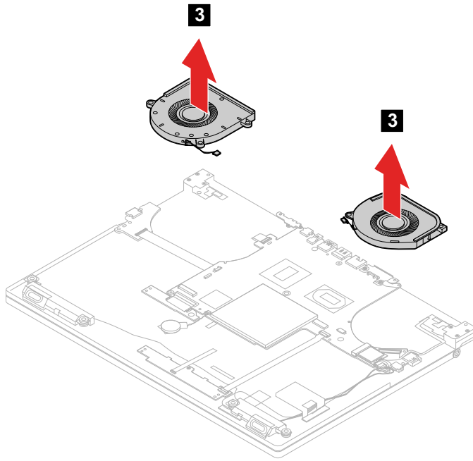
Figure 32. Remove the 2 fans
