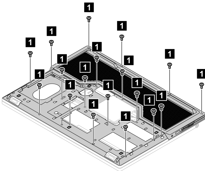
Figure 15. Remove the 18 screws
