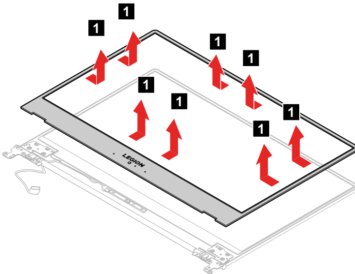
Figure 51. Pull the inner sides of the LCD bezel
