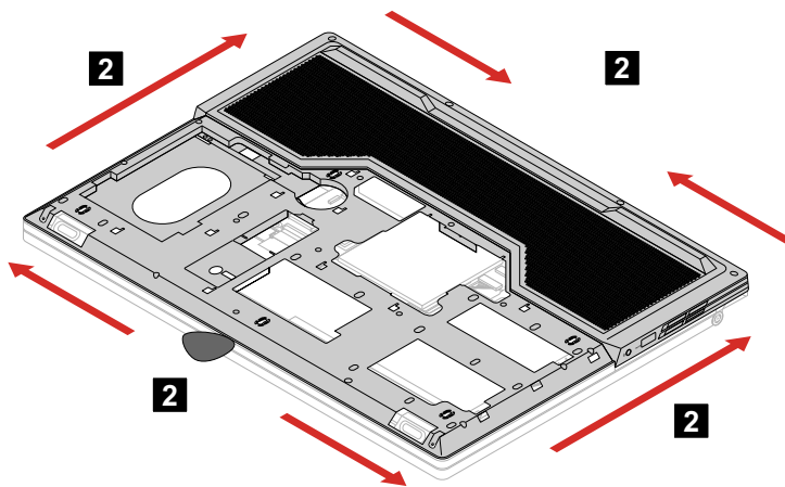
Figure 16. Separate the lower case from upper case
