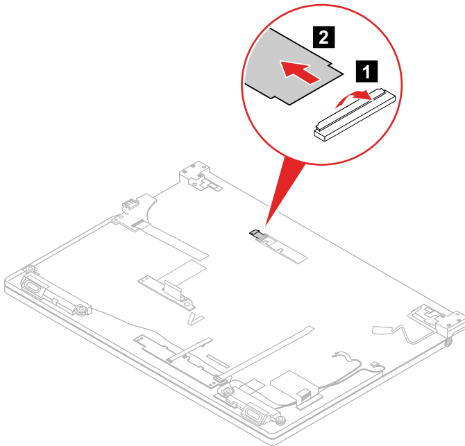
Figure 44. Detach the connector
