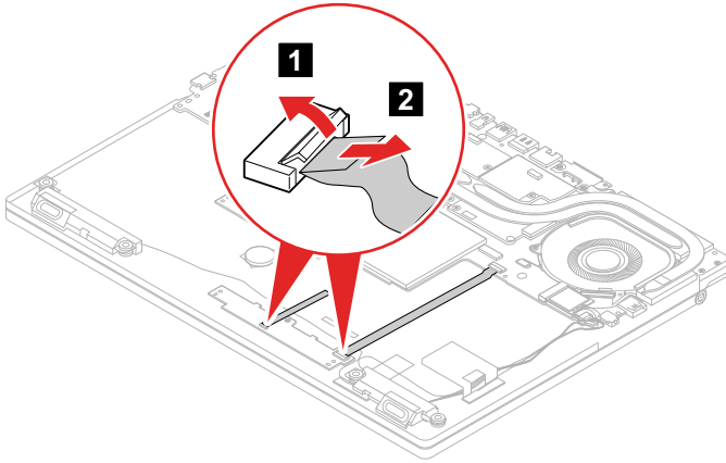
Figure 35. Detach the 2 connectors
