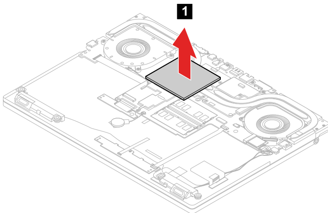
Figure 23. Remove the memory module shielding
