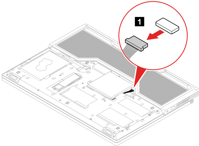
Figure 5. Detach the battery cable connector
