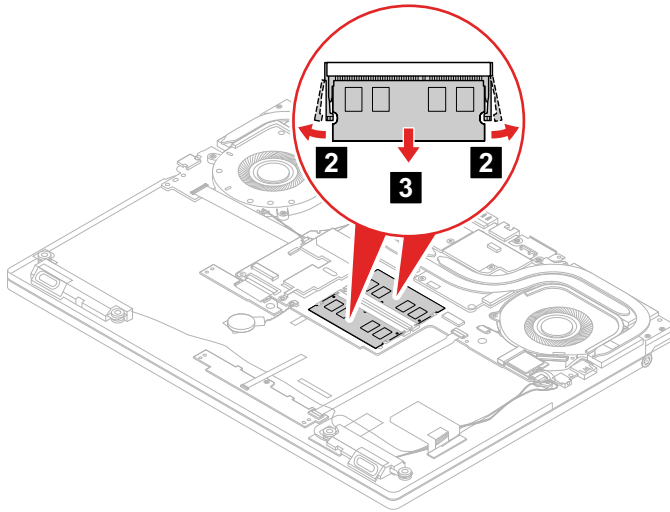
Figure 24. Remove the memory modules
