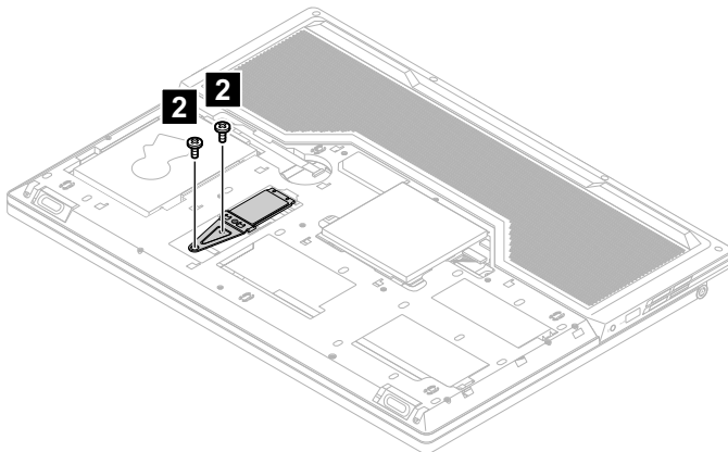
Figure 7. Remove the 2 screws (for 2242)
