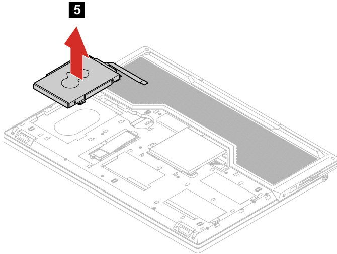
Figure 12. Remove the HDD assembly
