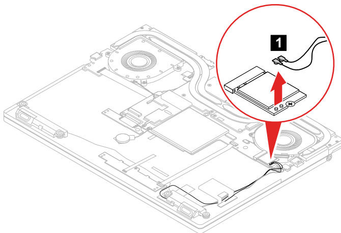
Figure 25. Detach the 2 connectors
