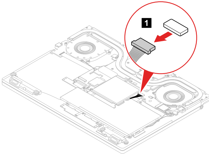
Figure 18. Detach the battery pack connector
