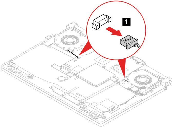
Figure 30. Detach the 2 fan connectors
