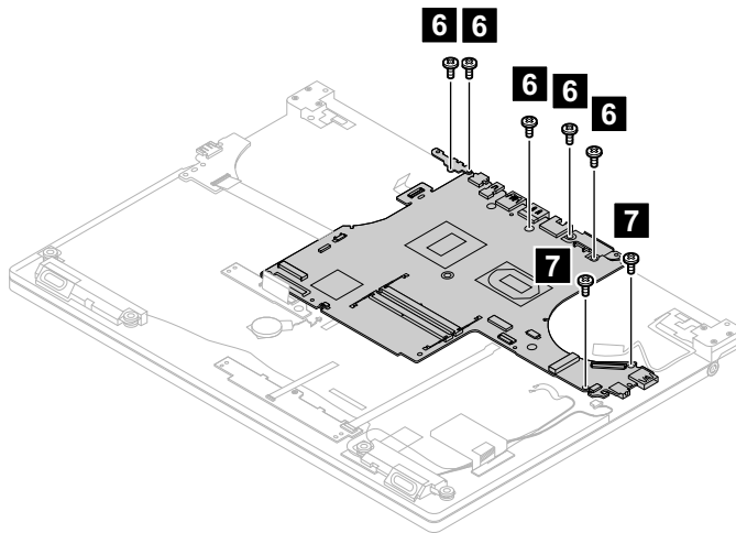
Figure 41. Remove the 7 screws
