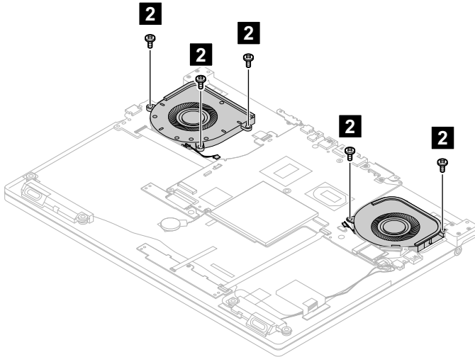
Figure 31. Remove the 5 screws
