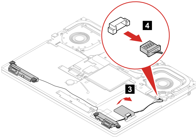
Figure 36. Peel off the aluminum foil and detach the speaker connector
