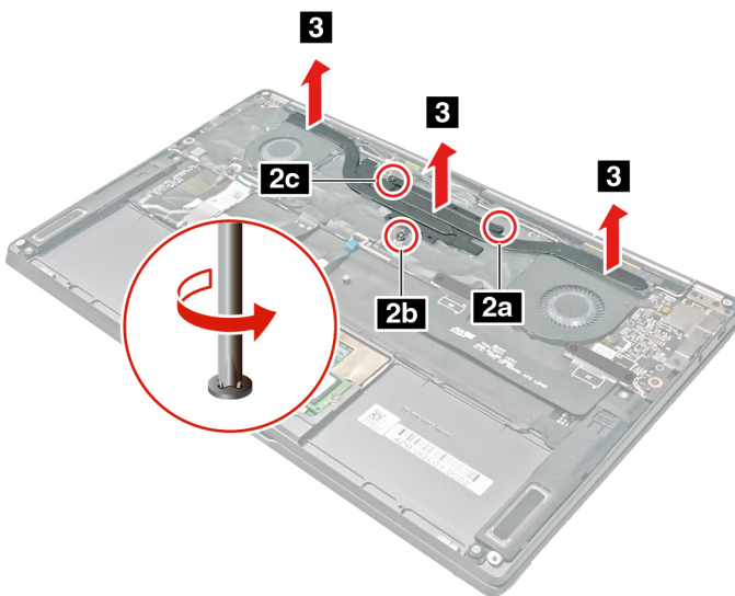
Figure 13. Loosen three screws and remove the heat sink
