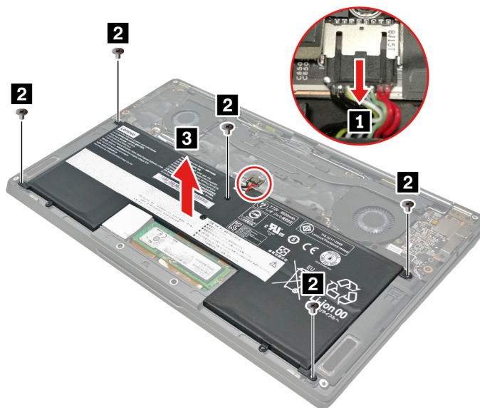
Figure 4. Remove the battery pack
