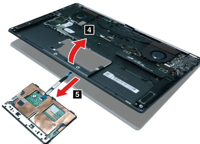
Figure 9. Remove the touch pad with cable
