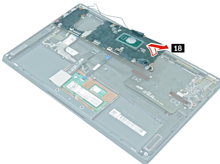
Figure 23. Remove the system board
