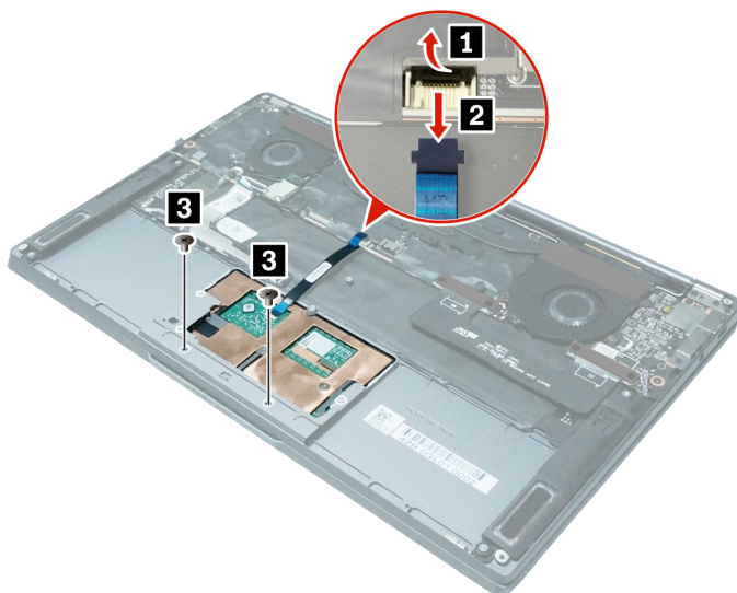
Figure 8. Disconnect the touch pad cable and remove screws
