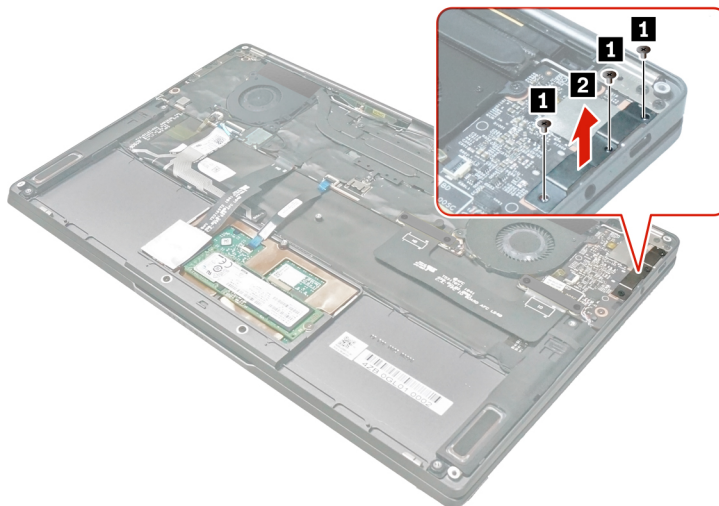
Figure 18. Remove the right I/O board bracket
