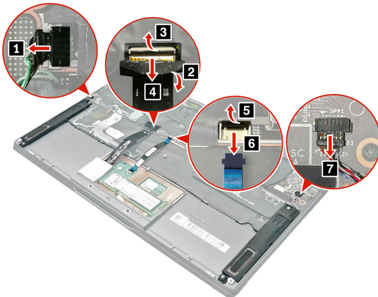
Figure 10. Disconnect cables
