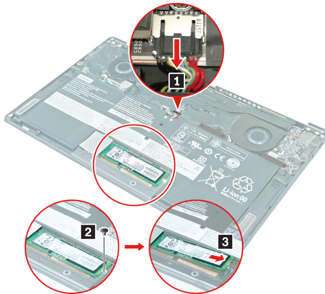
Figure 5. Remove the solid-state drive
