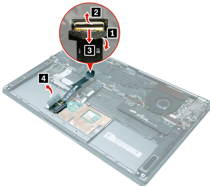
Figure 6. Disconnect the cable of the solid-state drive board
