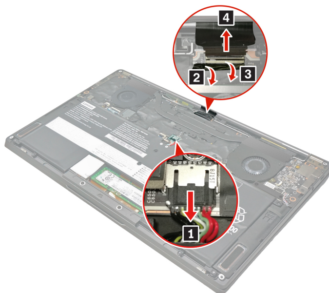
Figure 24. Disconnect the battery pack cable and LCD cable from the system board
