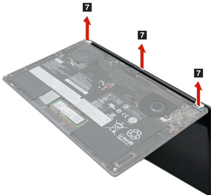
Figure 26. Remove the LCD module
