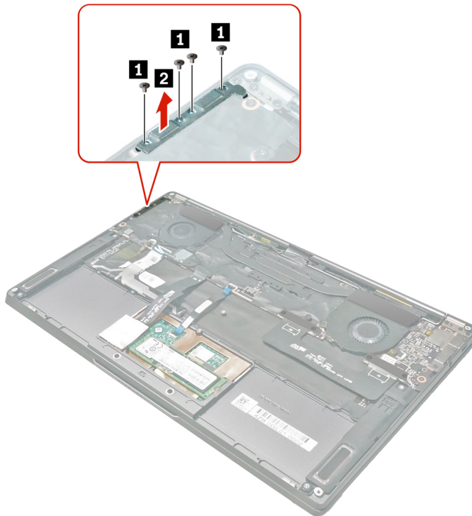
Figure 17. Remove the left I/O board bracket
