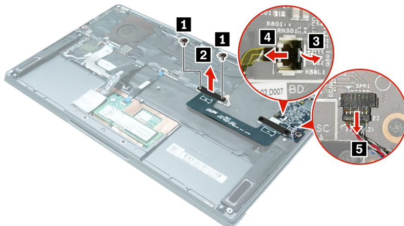
Figure 19. Remove two screws and disconnect cables
