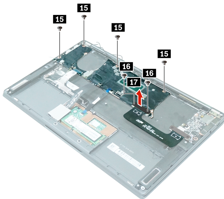
Figure 22. Remove six screws
