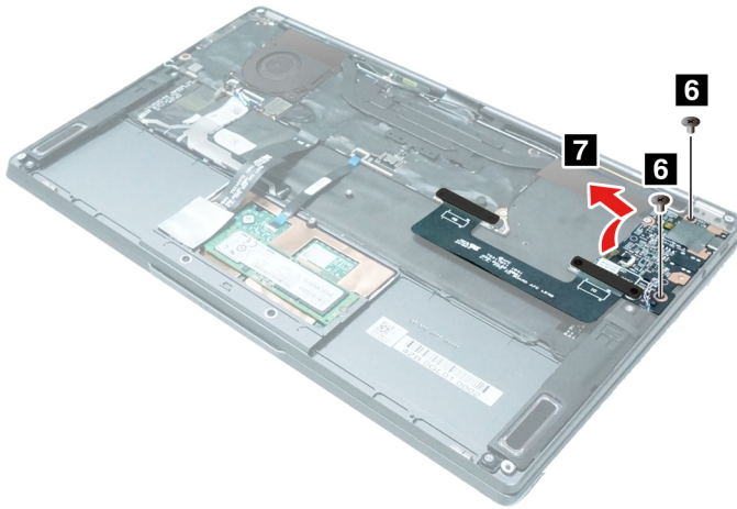
Figure 20. Remove two screws and remove the I/O board with cable
