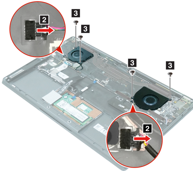
Figure 15. Disconnect the fan cables and remove four screws
