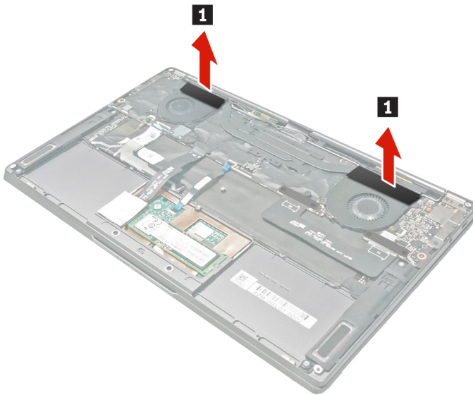
Figure 12. Peel off the acetate tapes
