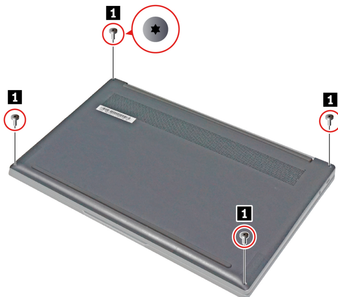
Figure 2. Remove four screws
