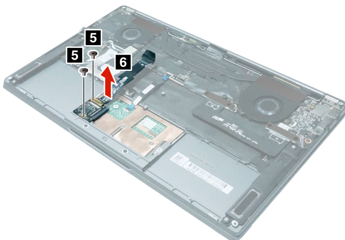
Figure 7. Remove the solid-state drive board with cable
