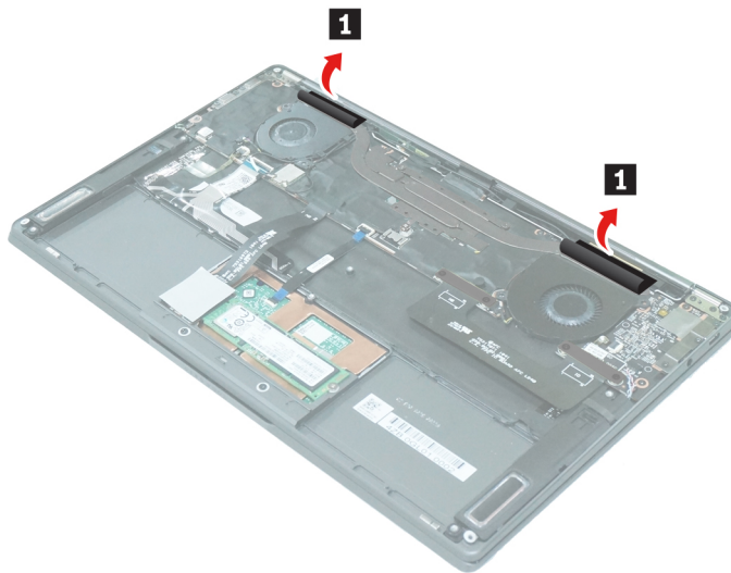
Figure 14. Peel off half of each acetate tape that covers the fan
