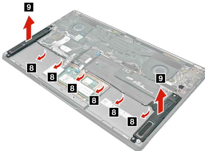
Figure 11. Remove speakers
