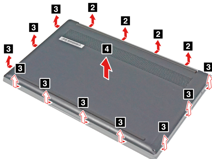
Figure 3. Pry up the latches and remove the lower case
