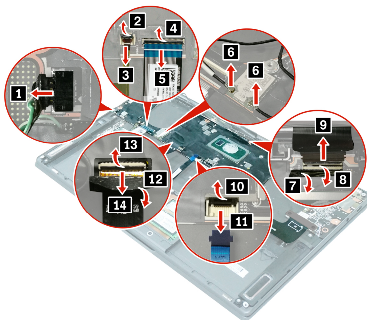
Figure 21. Disconnect cables
