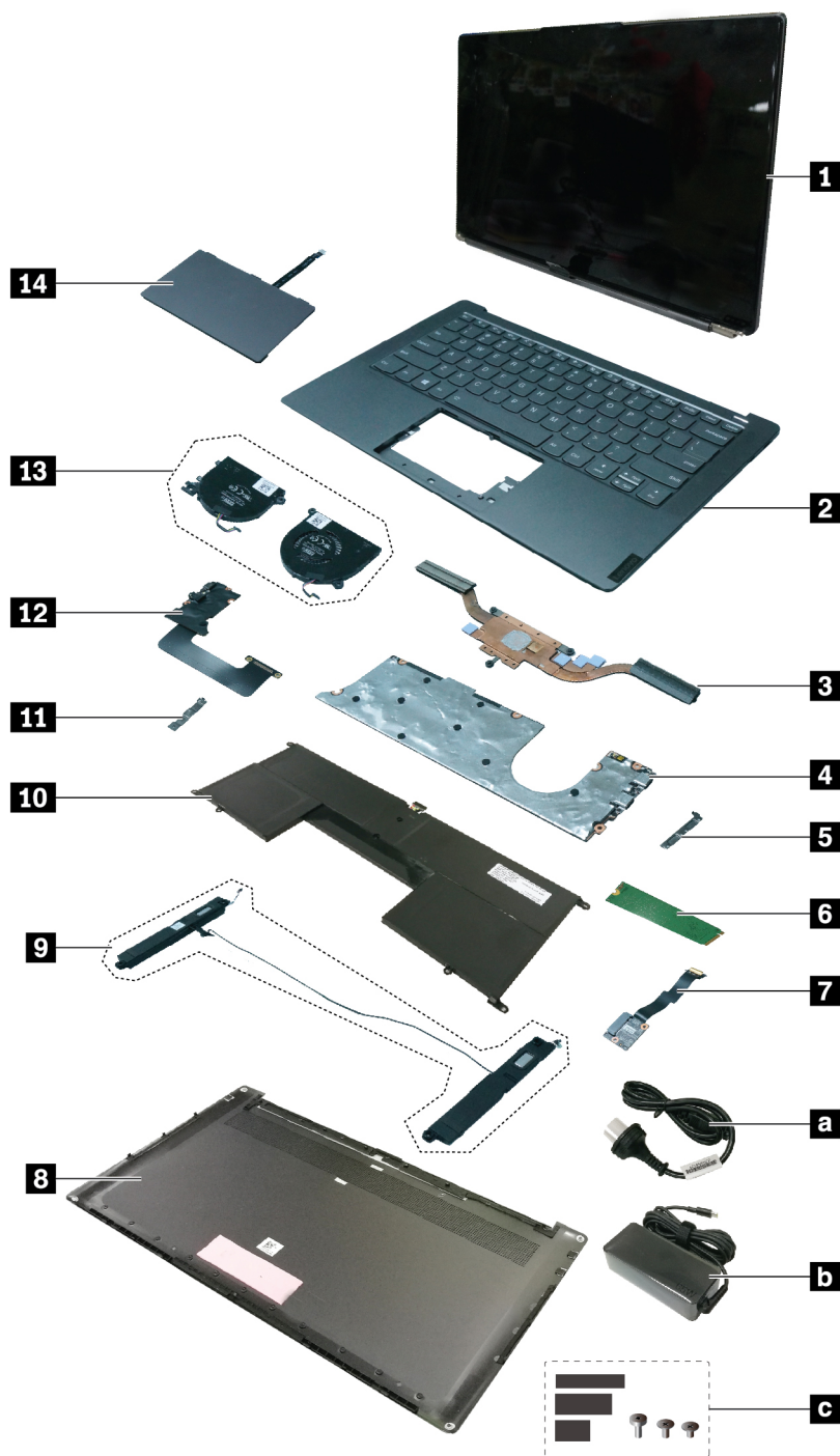
Figure 1. Lenovo IdeaPad S940-14IWL/Lenovo Yoga S940-14IWL exploded view
