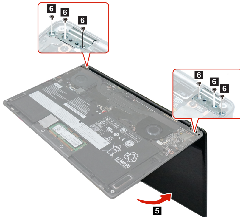
Figure 25. Rotate the LCD module and remove six screws
