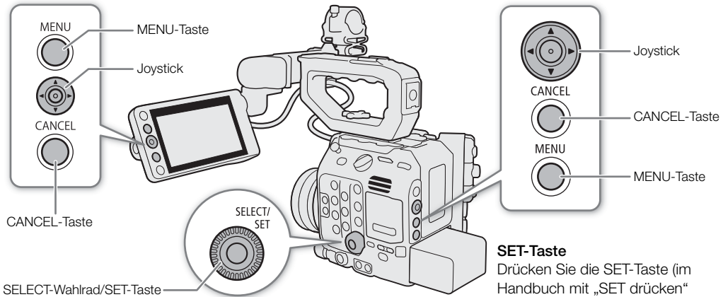
SELECT-Wahrrad/SET-Taste
