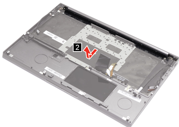
Figure 33. Remove upper case.
