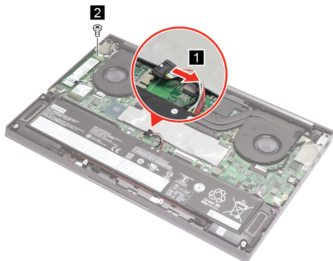
Figure 13. Remove one screw
