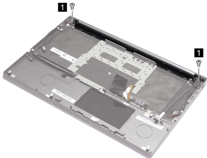
Figure 32. Remove two screws
