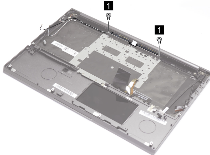
Figure 28. Remove two screws
