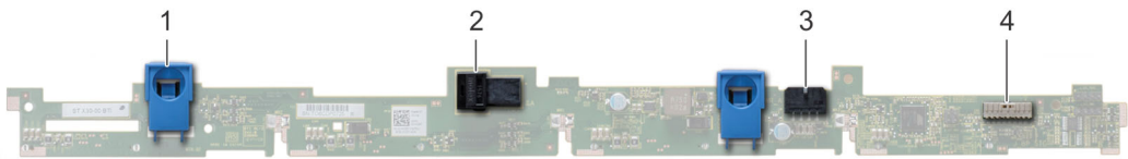
Figure 82. Backplane 4 x 3,5
