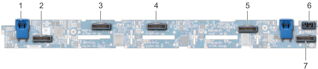
Figure 84. Backplane 10 x 2,5
