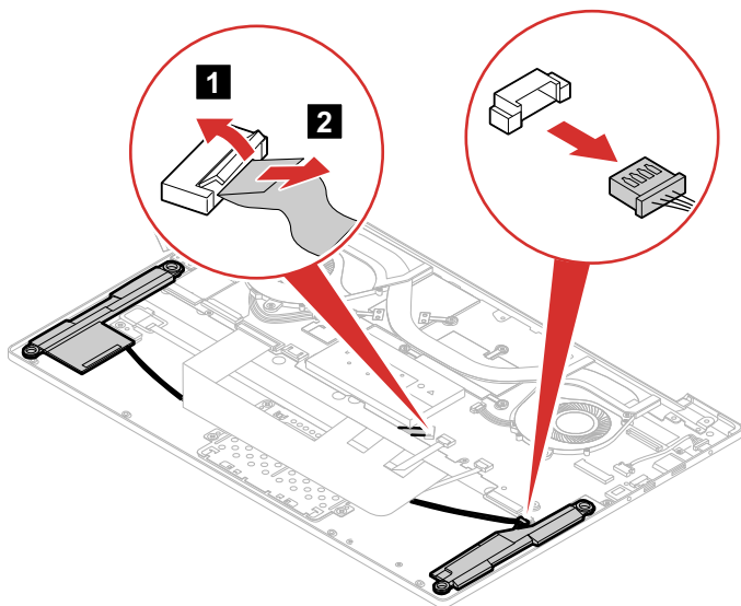
Figure 20. Disconnect 2 cables
