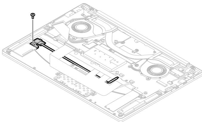
Figure 23. Remove 1 screw
