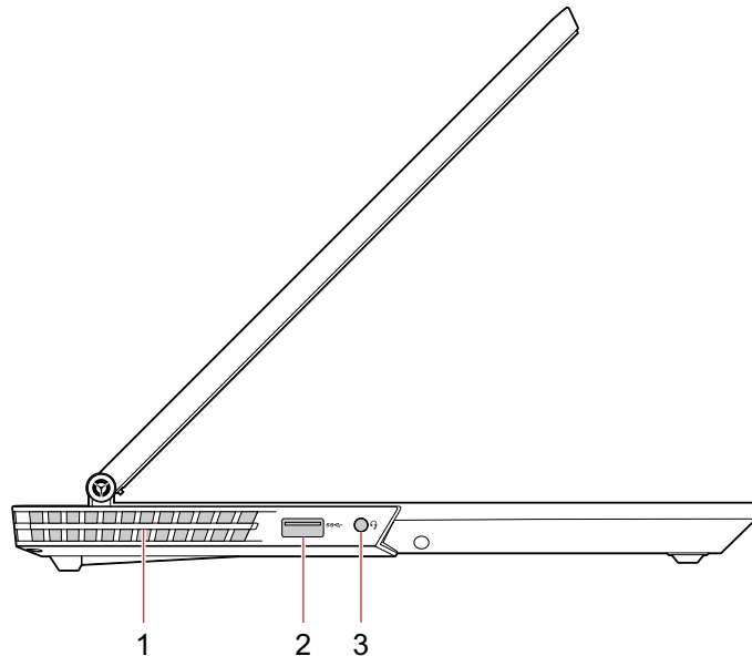
Figure 2. Legion Y7000 2019 Series - left view
