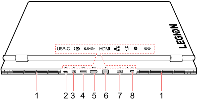
Figure 4. Legion Y7000 2019 Series - rear view
