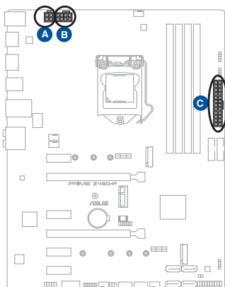
A EATX12V_2
