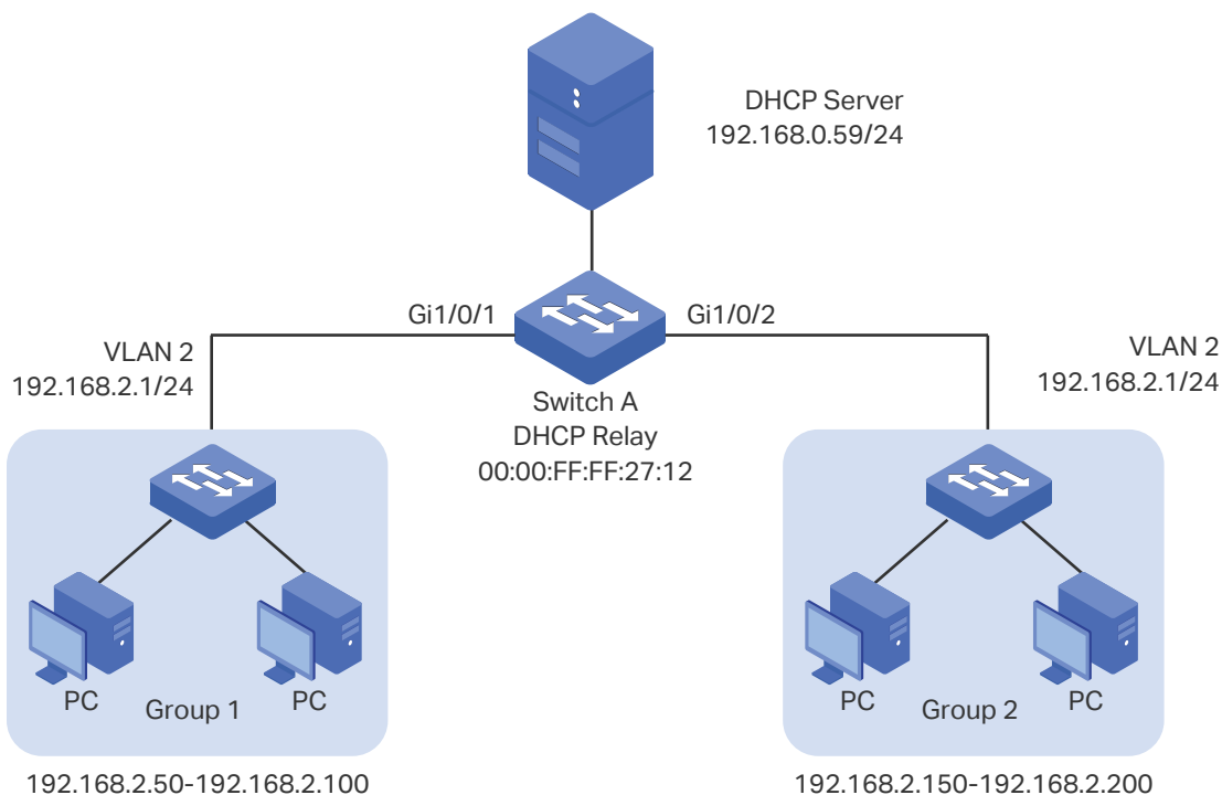
Figure 5-28 Network Topology for Option 82 in DHCP Relay
