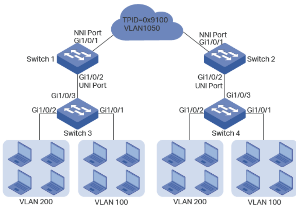
Figure 4-10 Network Topology
