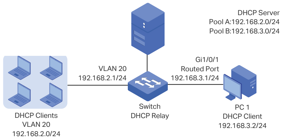
Figure 1-2 Application Scenario of DHCP Interface Relay
