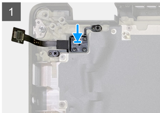
2x M2x2.5
