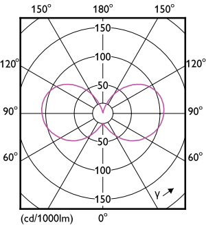
Light Distribution Diagram - LEDClassic SSW 40W B35 E14 WW CLND 1SRT4
