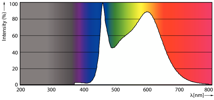
Spectral Power Distribution Colour - LED classic 100W A60 CW FR ND RFRFSRT4
