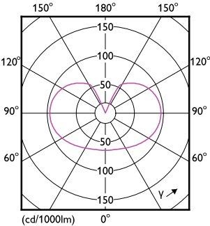
Light Distribution Diagram - LED classic 100W A60 CW FR ND RFRFSRT4
