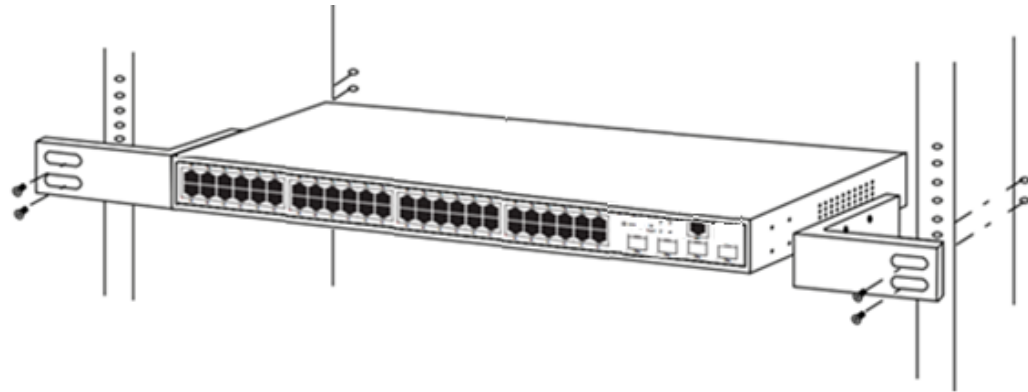
Figure 6 - Rack Installation
