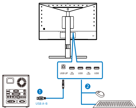
USB hub
