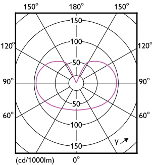
Light Distribution Diagram - LED classic 100W A60 E27 CW FR ND 2SRT6
