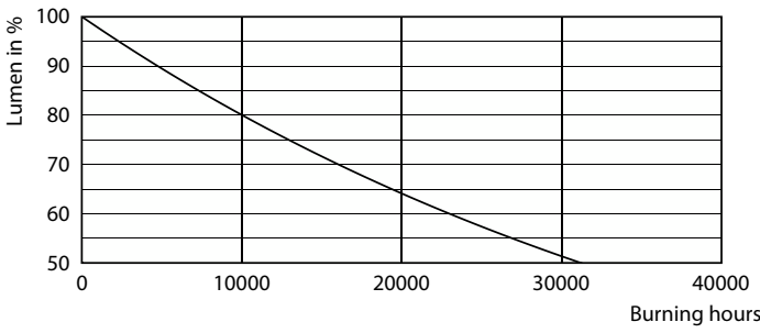
Lumen Maintenance Diagram - LED classic 100W A60 E27 CW FR ND 2SRT6
