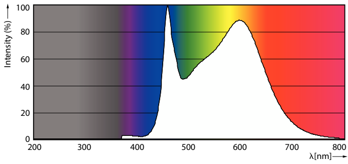
Spectral Power Distribution Colour - LED classic 100W A60 E27 CW FR ND 2SRT6
