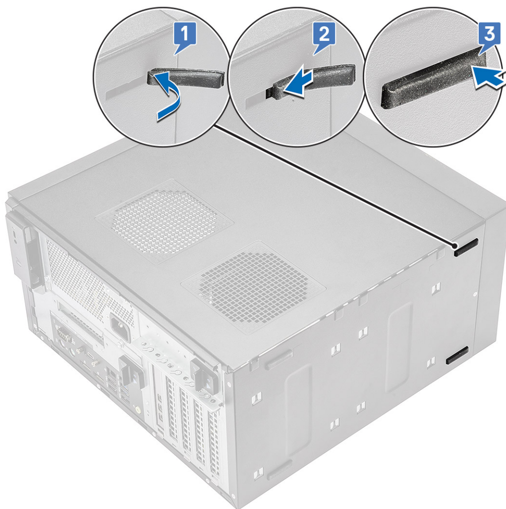
Figure 14. Front rubber feet installation
