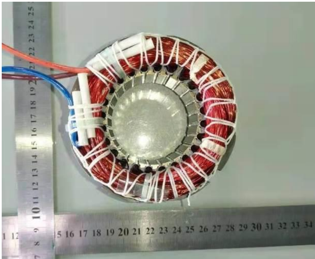
Motor stator for P3117
