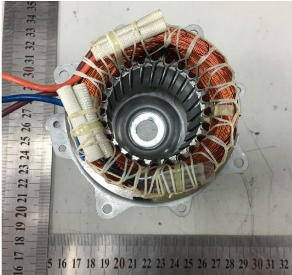
Motor stator for P3115
