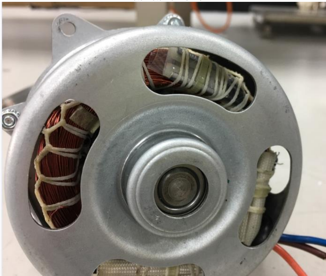
Motor rotor for P3119
