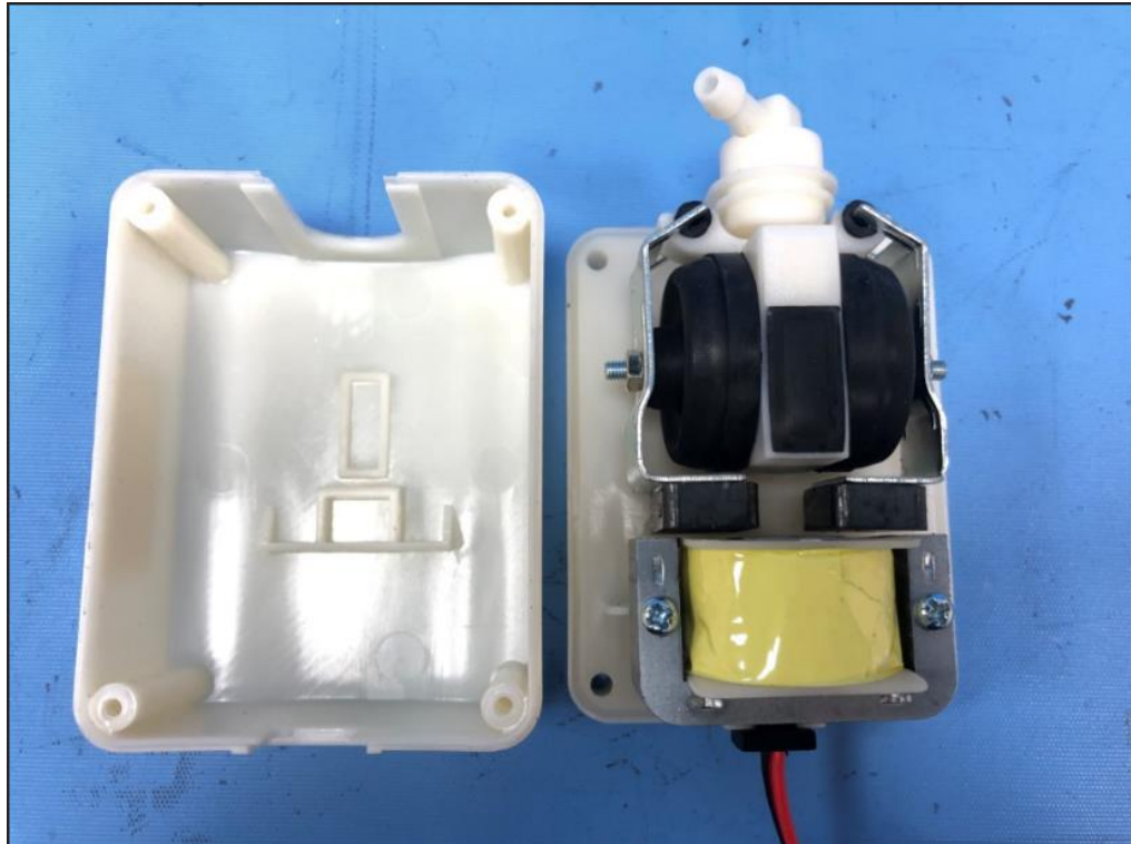
Filling pump view
