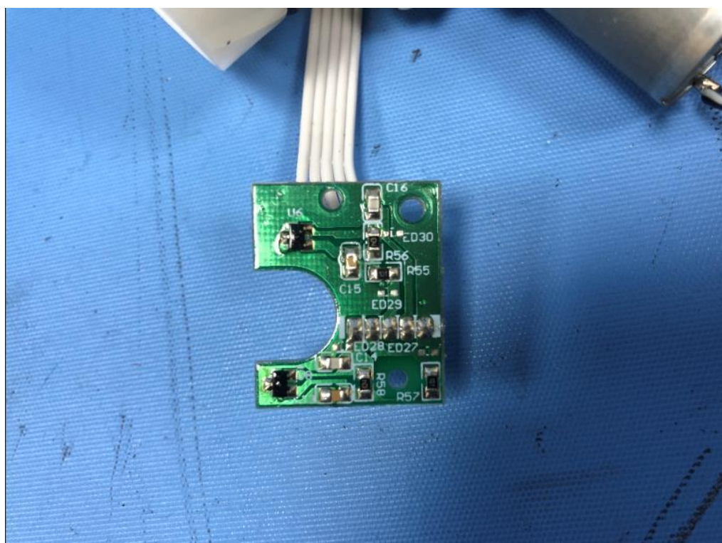
Valve PCB
