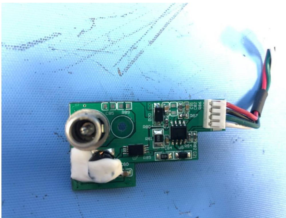
PCB view
