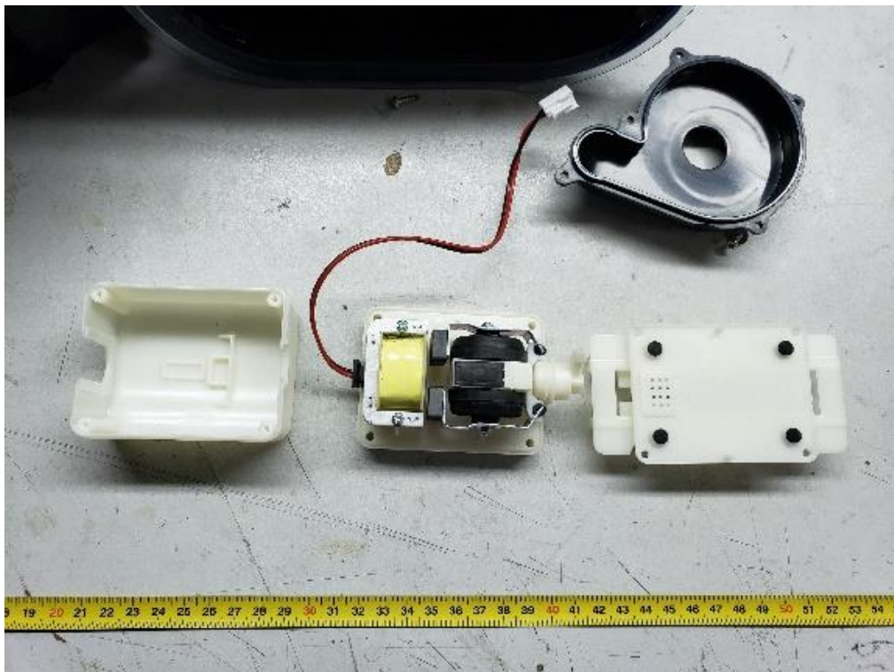
Filling pump view
