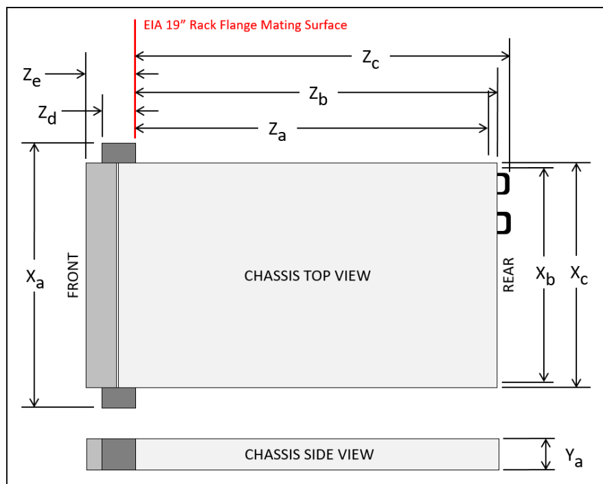
Figure 8. Server dimensions
