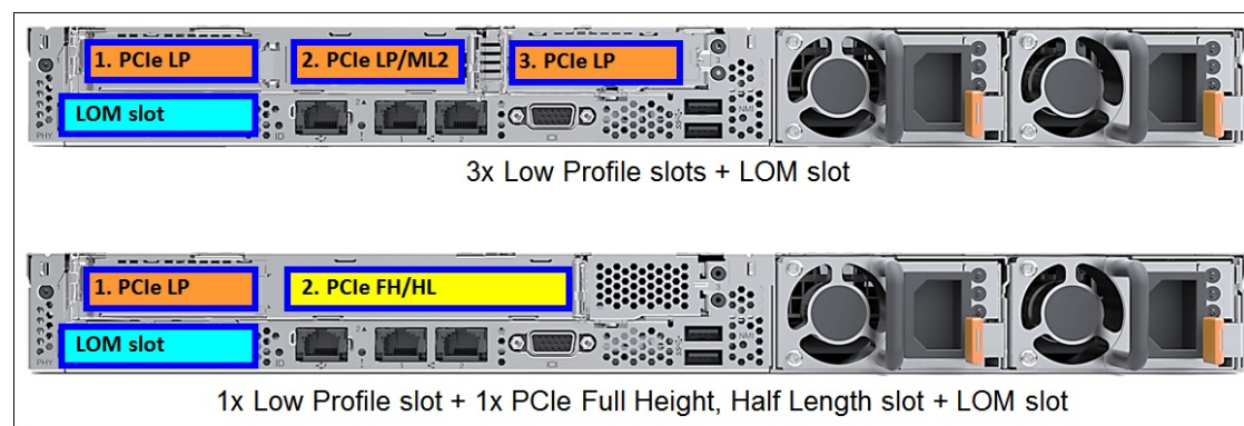
Figure 7. Slot locations
