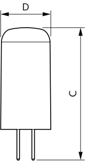
GY6.35 1.9W-20W 200lm 2700K Non-Dim
