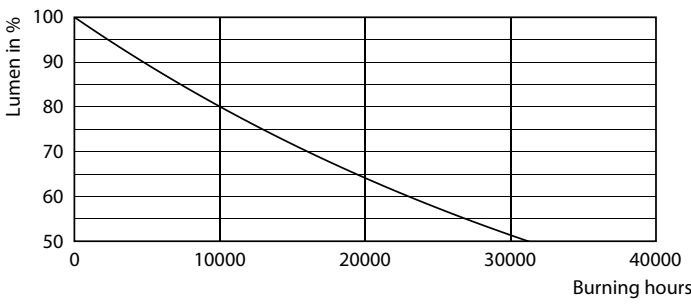
Lumen Maintenance Diagram - LEDBulb 6W B22 965 230V 2PF/3 AU
