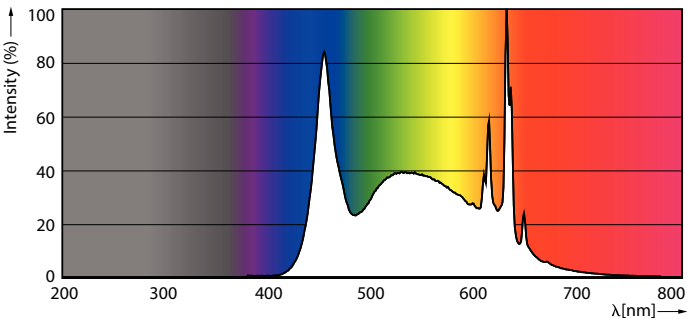
Spectral Power Distribution Colour - LEDBulb 6W B22 965 230V 2PF/3 AU
