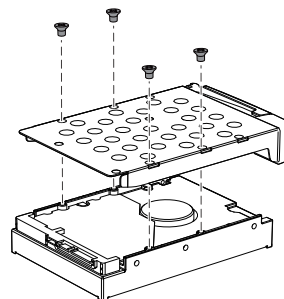
3.5-inch HDD
