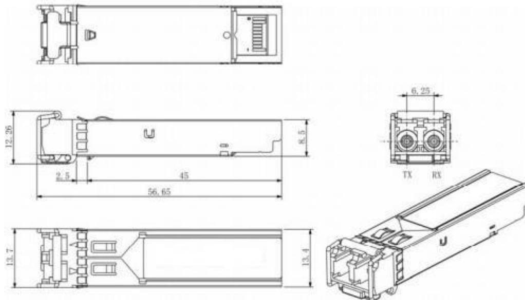
Mechanical Drawing
