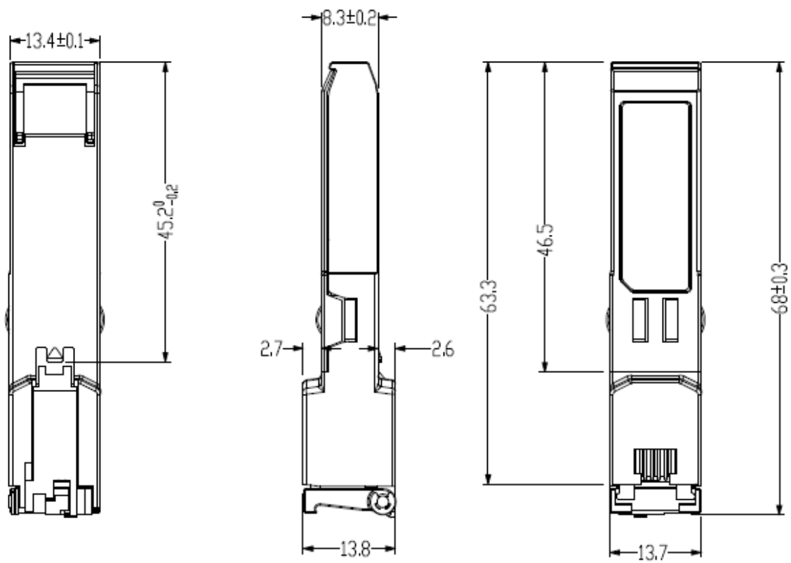
Mechanical Drawing
