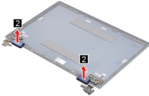
Figure 25. Remove the hinge
