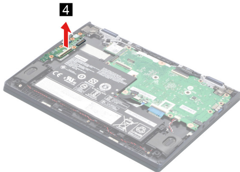
Figure 8. Remove the I/O board
