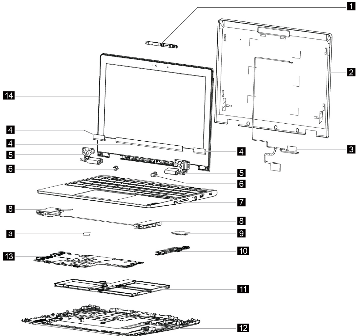
Figure 1. IdeaPad Flex 3 Chromebook (11", 05) exploded view
