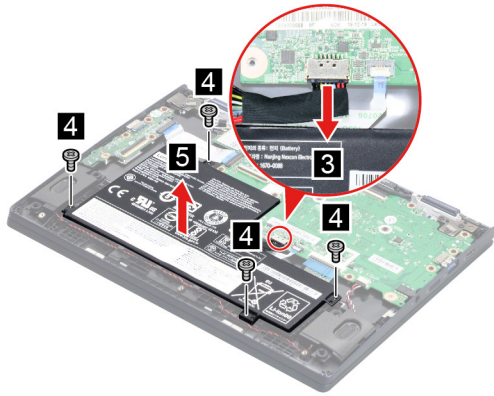
Figure 5. Remove the battery pack
