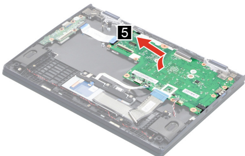
Figure 13. Remove the system board
