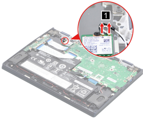
Figure 9. Detach the main and auxiliary antenna cable connectors.
