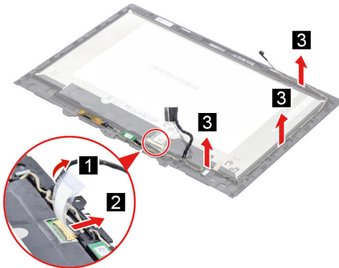
Figure 26. Remove the LVDS cable
