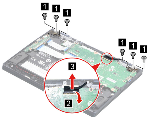
Figure 17. Remove six screws
