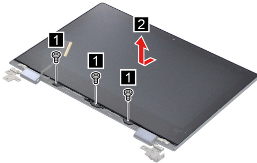
Figure 21. Remove the LCD module
