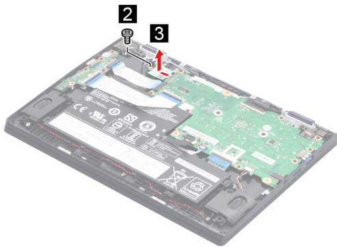
Figure 10. Remove one screw and remove the WLAN card
