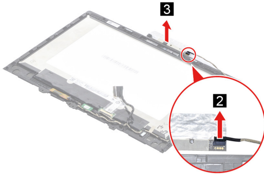
Figure 23. Remove the camera
