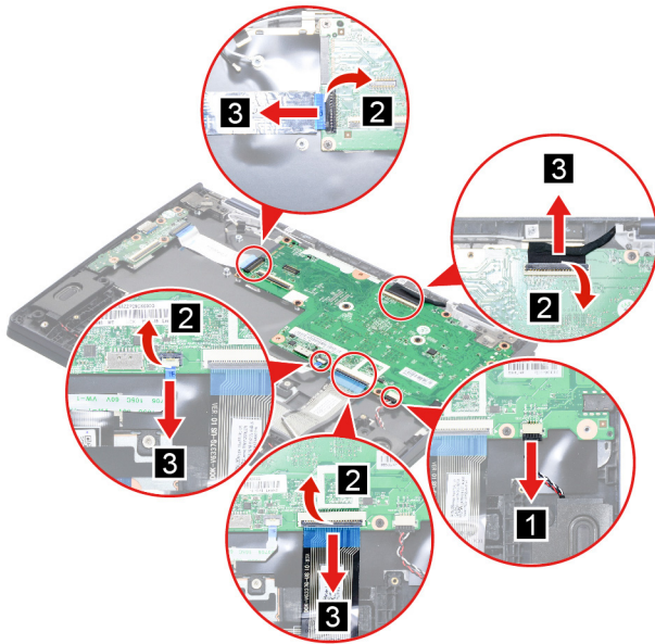
Figure 11. Disconnect cables connected to the system board
