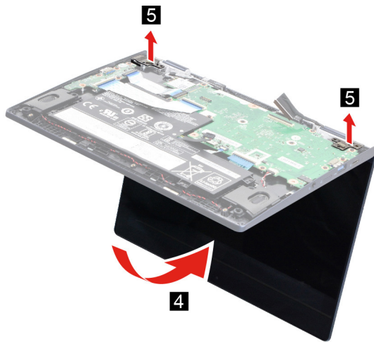
Figure 18. Remove the LCD unit
