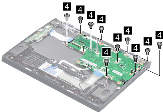
Figure 12. Remove ten screws
