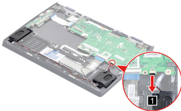
Figure 14. Disconnect the speaker cable from the system board
