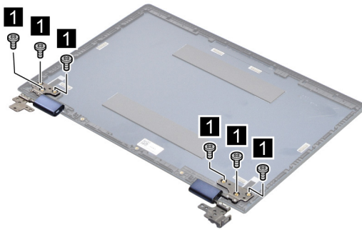
Figure 24. Remove six screws
