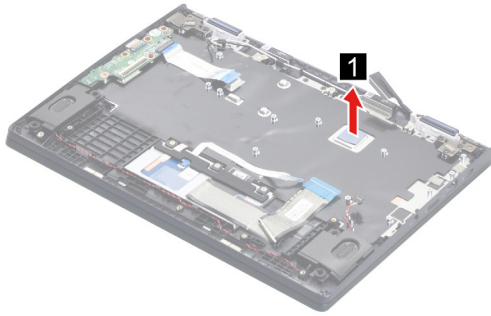
Figure 16. Remove the thermal pad
