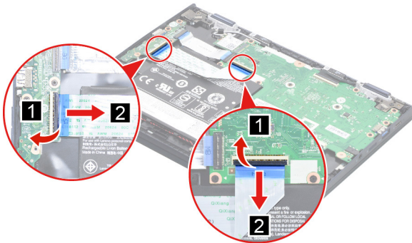
Figure 4. Remove the I/O board cable
