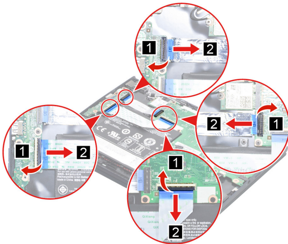
Figure 6. Disconnect the cable of the I/O board
