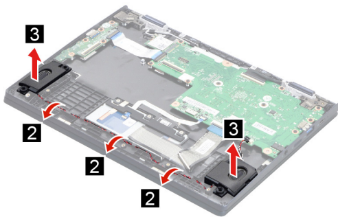
Figure 15. Remove the speakers
