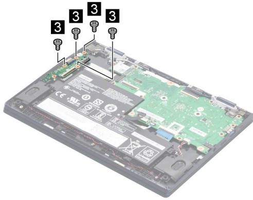
Figure 7. Remove four screws
