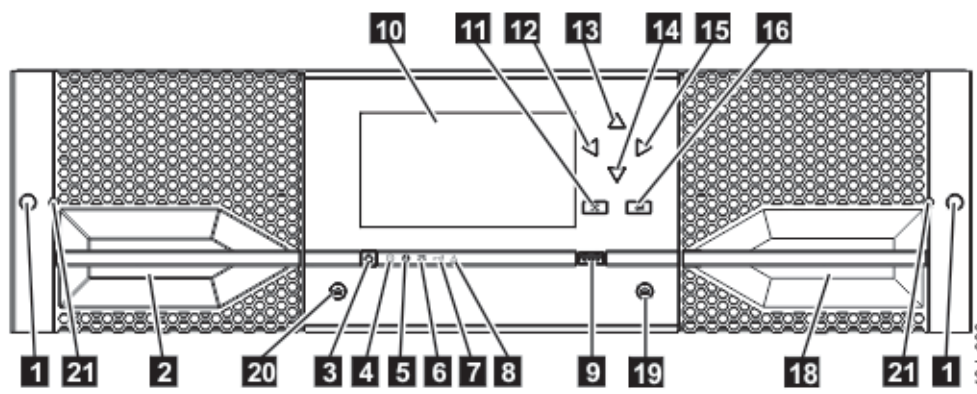
Figura 7. Panel frontal
