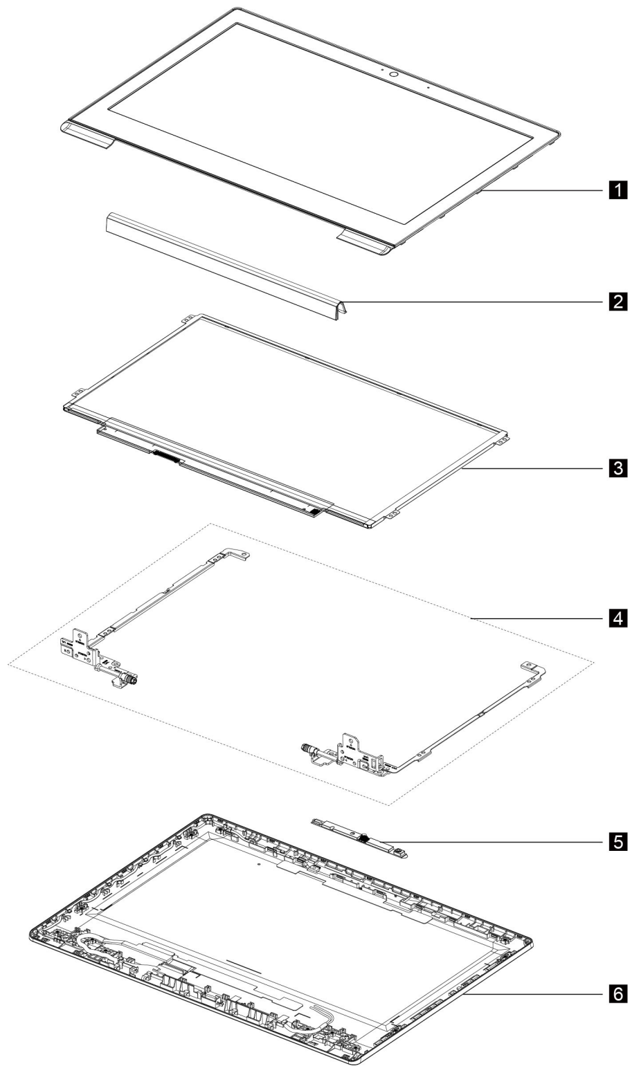
Figure 2. LCD module - exploded view - IdeaPad 3 CB 11IGL05 and IdeaPad 3 CB 11AST5
