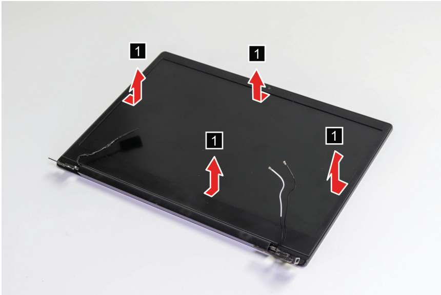
Figure 45. Remove the LCD bezel
