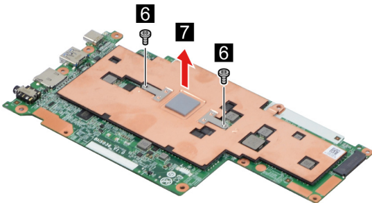
Figure 16. Remove two screws and remove the heat sink
