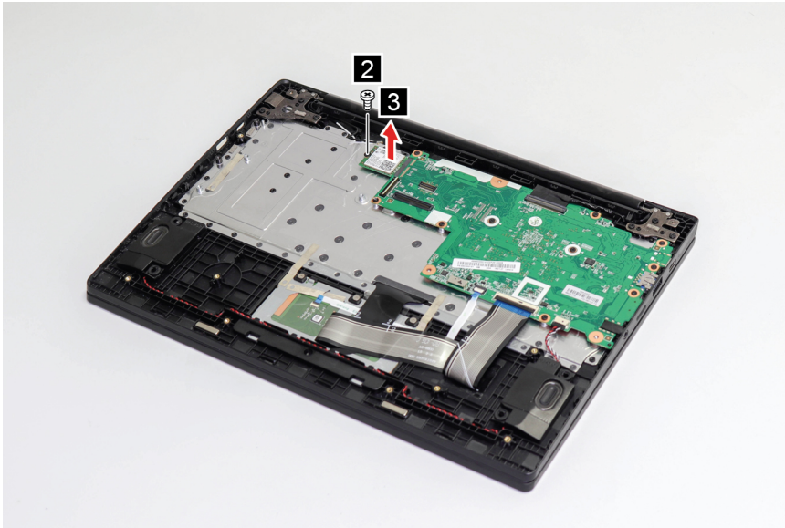
Figure 36. Remove one screw and remove the WLAN card
