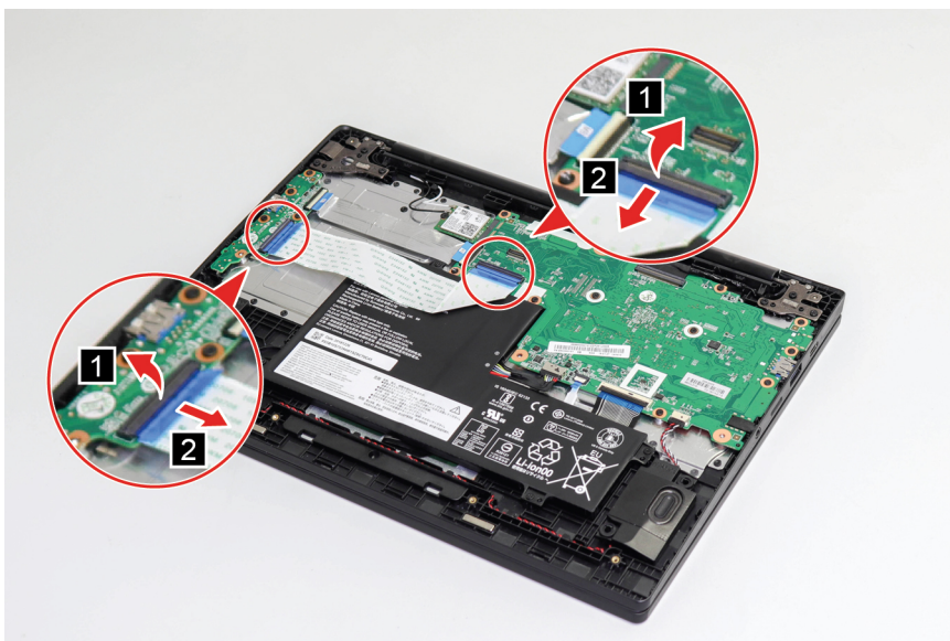
Figure 30. Remove the I/O board cable
