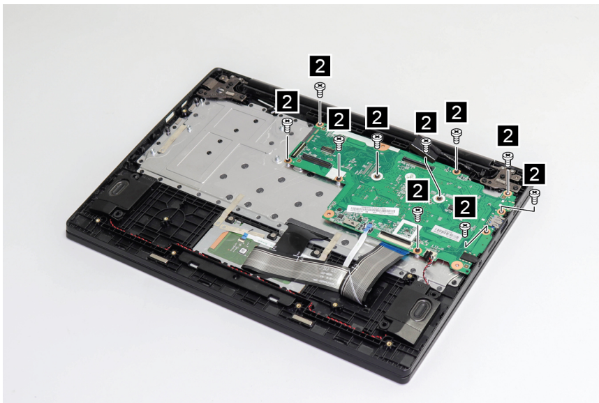
Figure 38. Remove ten screws
