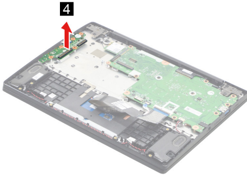
Figure 10. Remove the I/O board
