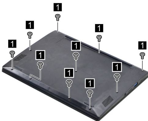
Figure 5. Remove ten screws
