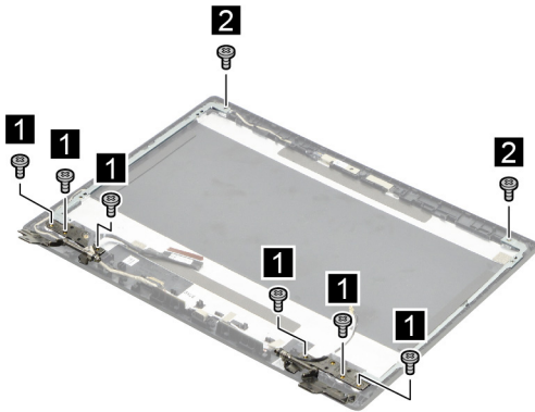
Figure 24. Remove eight screws
