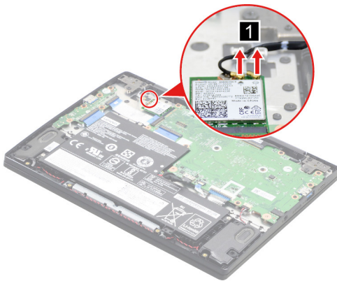
Figure 11. Detach the main and auxiliary antenna cable connectors
