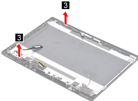
Figure 27. Remove the EDP cable
