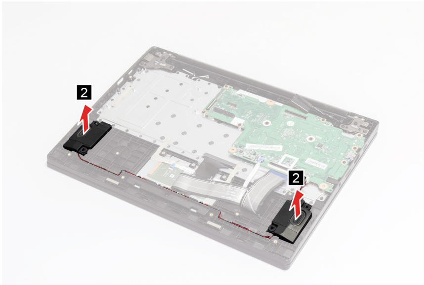
Figure 41. Remove the speakers
