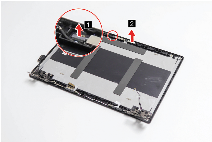
Figure 49. Remove the camera
