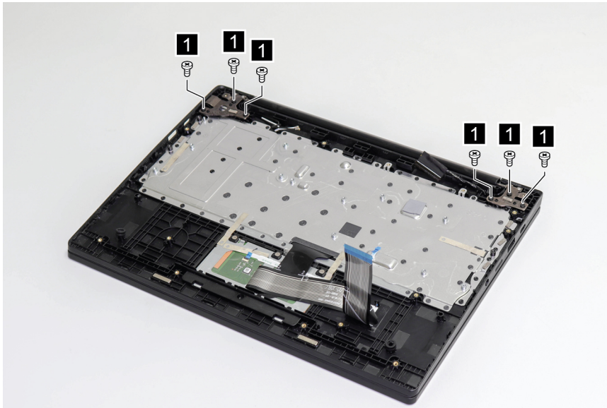
Figure 43. Remove six screws
