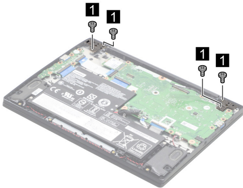
Figure 17. Remove four screws
