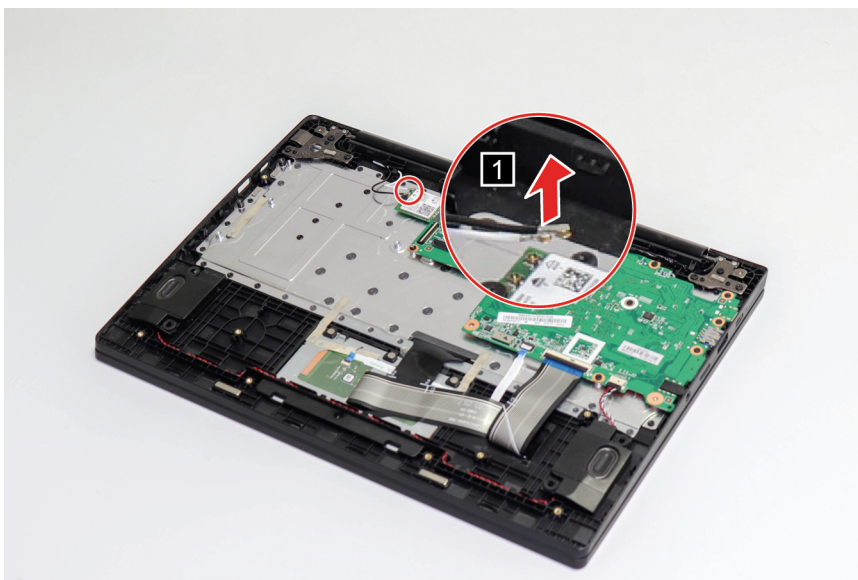
Figure 35. Disconnect the antenna cables
