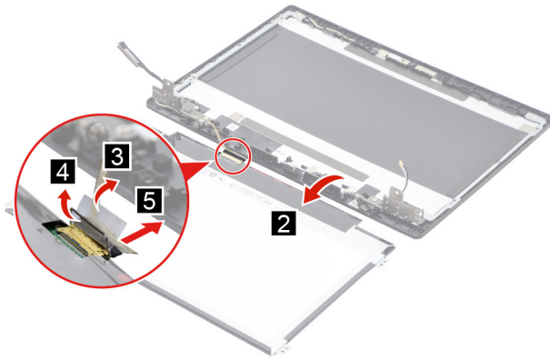
Figure 22. Remove the LCD panel
