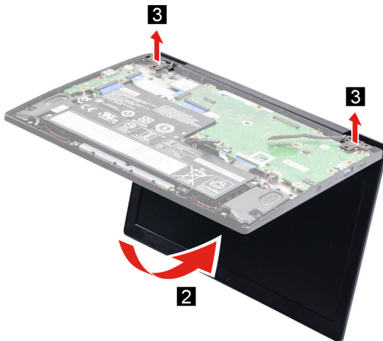
Figure 18. Remove the LCD module
