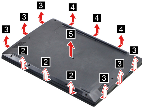
Figure 6. Pry up the latches and remove the lower case
