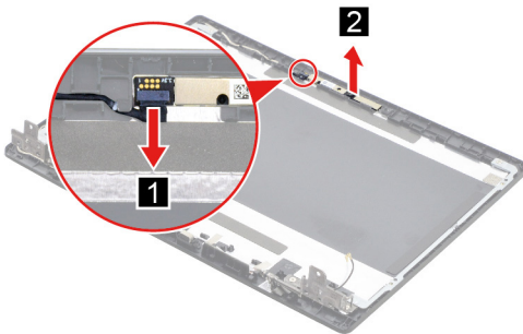
Figure 23. Remove the camera
