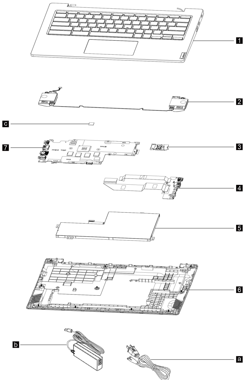
Figure 3. exploded view - IdeaPad 3 CB 14IGL05
