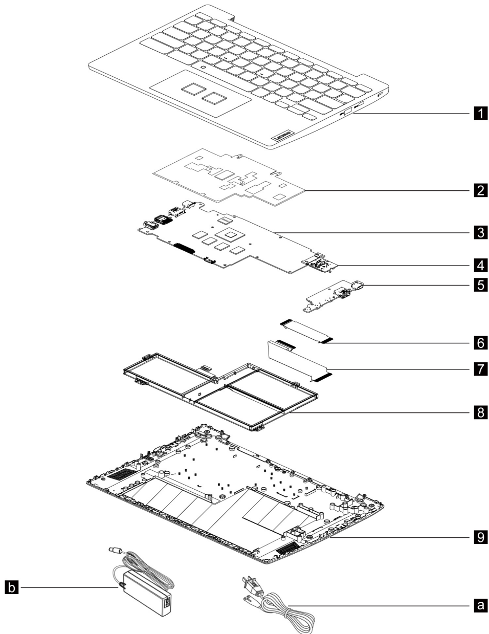
Figure 1. exploded view - IdeaPad 3 CB 11IGL05 and IdeaPad 3 CB 11AST5
