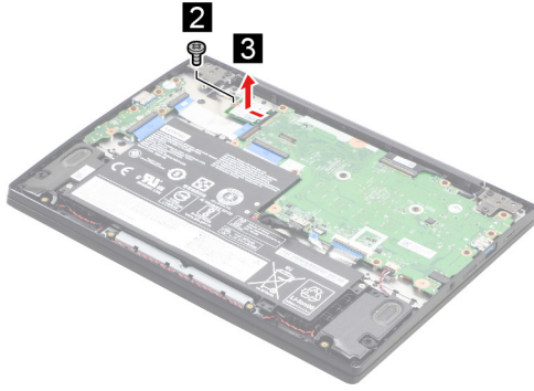
Figure 12. Remove one screw and remove the WLAN card
