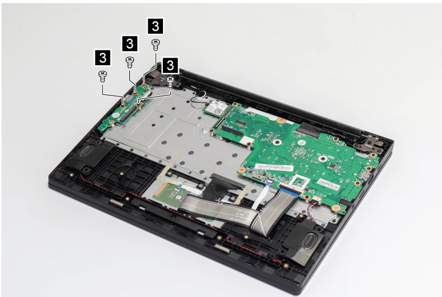
Figure 33. Remove four screws
