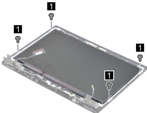
Figure 21. Remove four screws
