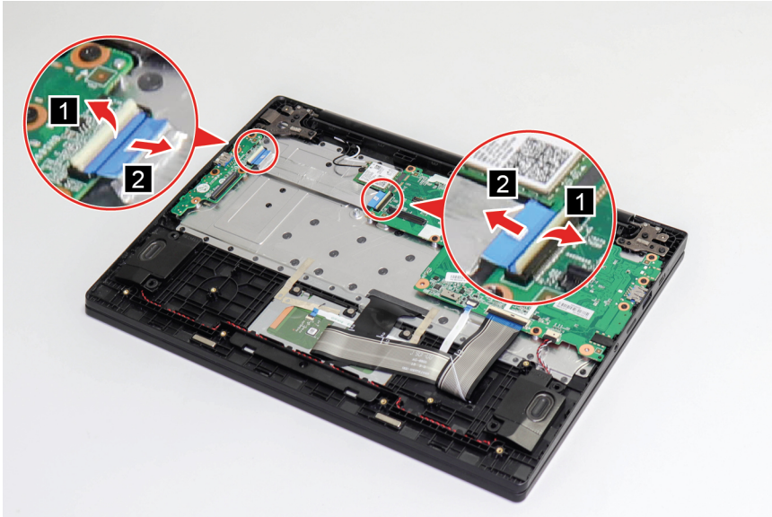
Figure 32. Disconnect the cable of the I/O board
