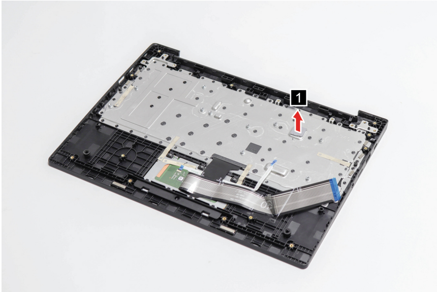
Figure 42. Remove the thermal pad
