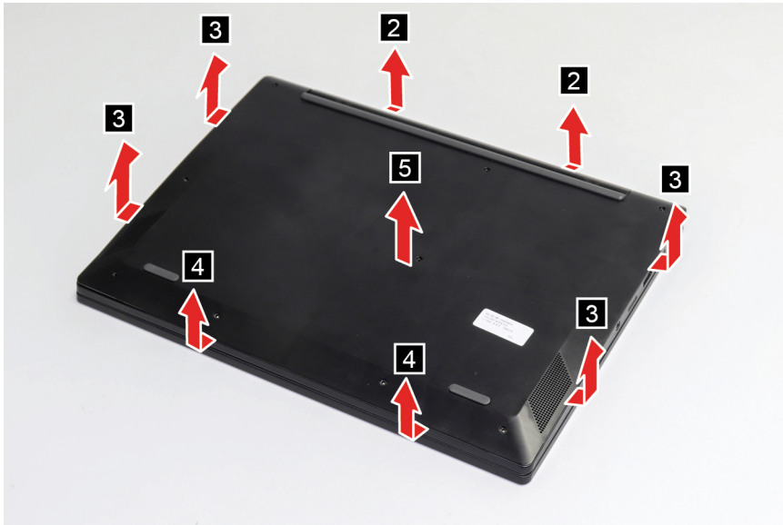
Figure 29. Pry up the latches and remove the lower case
