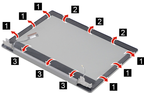
Figure 19. Remove the LCD bezel
