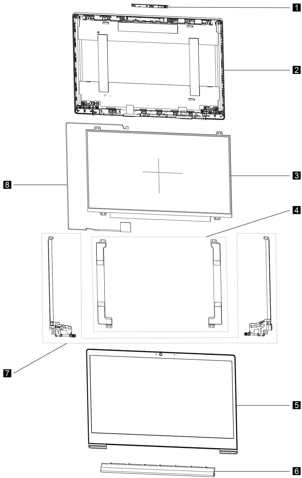
Figure 4. LCD module - exploded view - IdeaPad 3 CB 14IGL05
