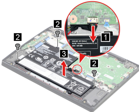
Figure 7. Remove three screws and remove the battery pack
