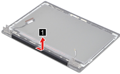
Figure 20. Remove the strip cover
