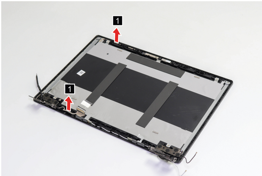
Figure 52. Remove the LVDS cable
