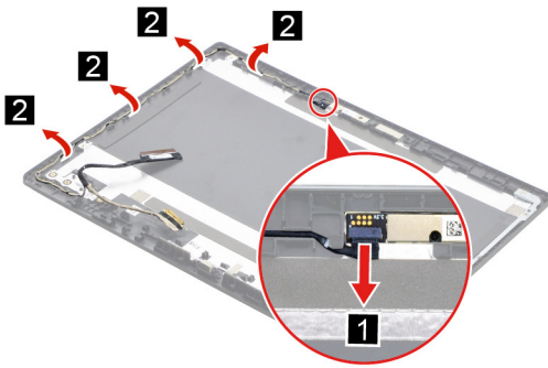
Figure 26. Disconnect the EDP cable from the camera and release the EDP cable from the cable guide
