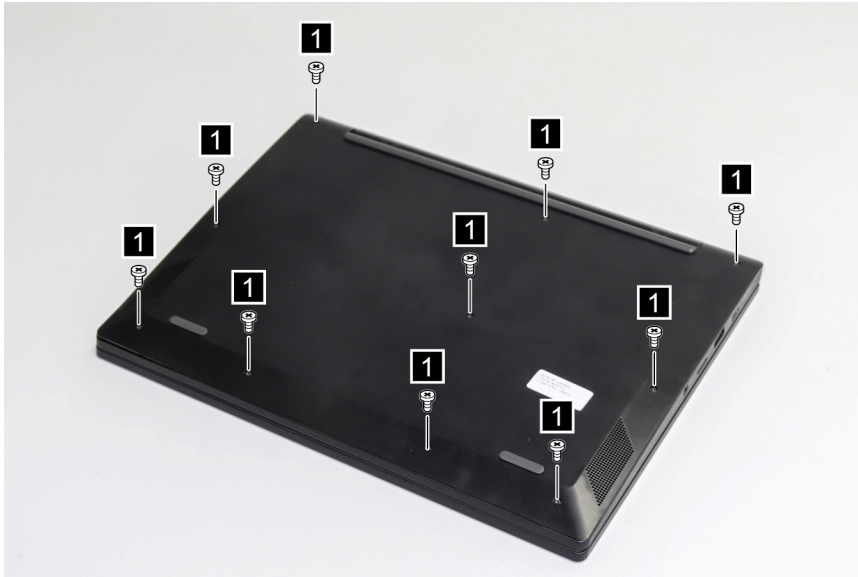
Figure 28. Remove ten screws
