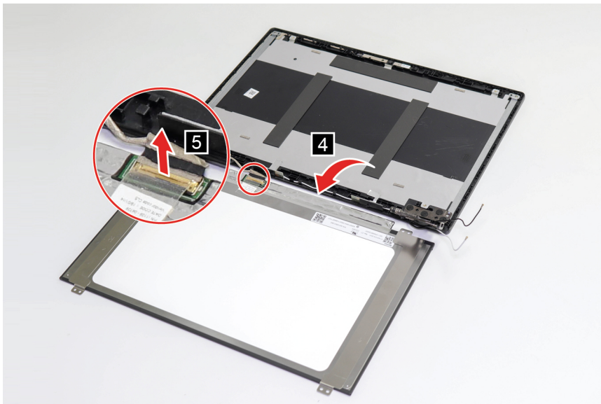
Figure 48. Remove the LCD panel
