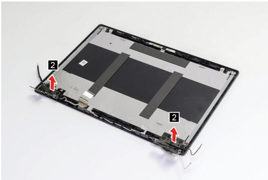
Figure 51. Remove the hinges
