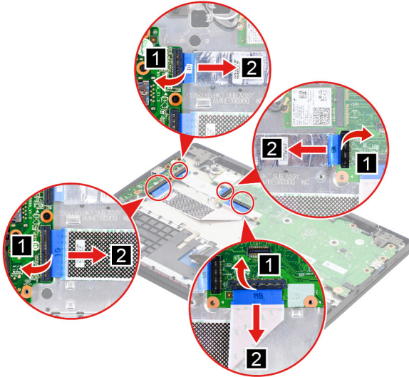
Figure 8. Remove the I/O board cables
