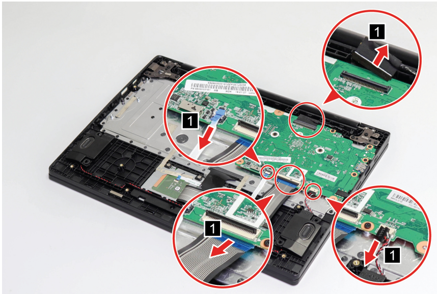
Figure 37. Disconnect cables
