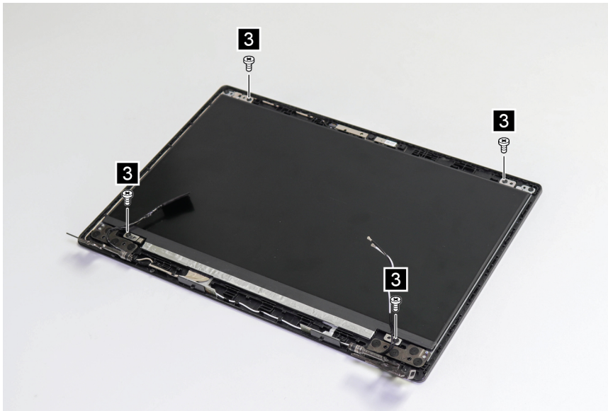
Figure 47. Remove four screws
