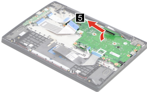
Figure 15. Remove the system board
