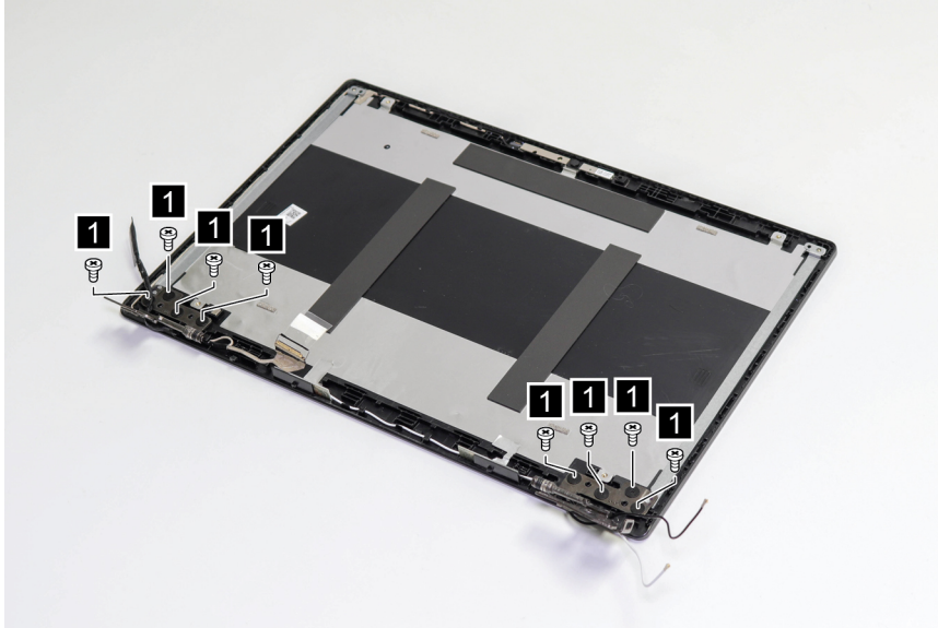
Figure 50. Remove eight screws
