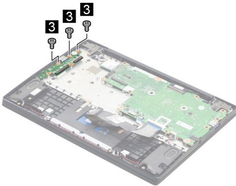
Figure 9. Remove three screws
