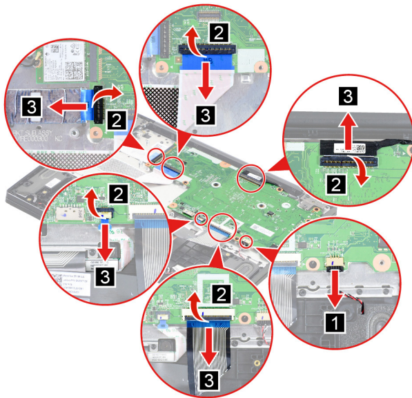
Figure 13. Disconnect cables connected to the system board
