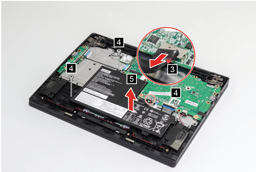
Figure 31. Remove the battery pack
