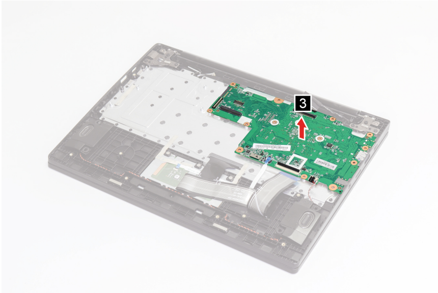
Figure 39. Remove the system board
