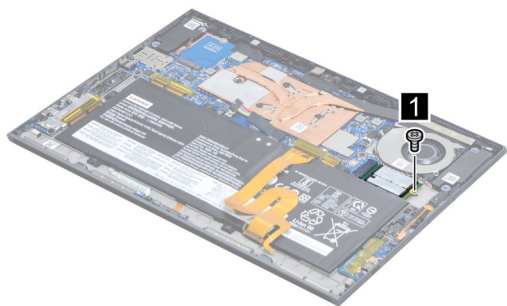
Figure 9. Remove one screw
