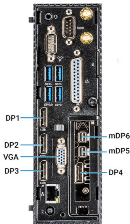
Figure 36. Ports on Wyse 5070 Extended thin client
