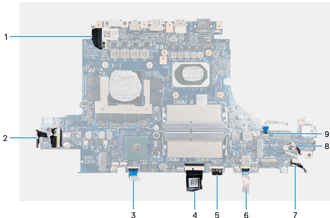
Figure 1. System-board cables
