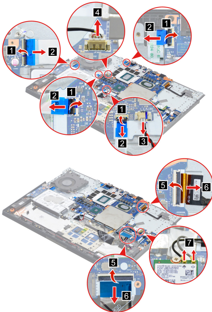
Figure 23. Disconnect cables connected to the system board and detach the antenna cable connectors
