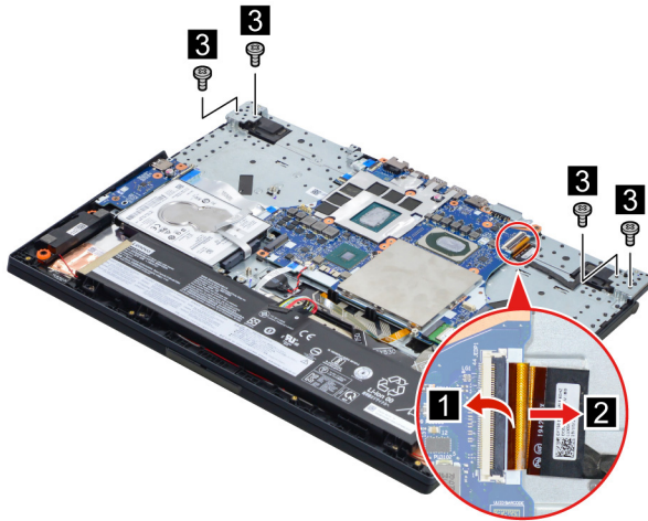
Figure 32. Disconnect the EDP cable from the system board and remove four screws
