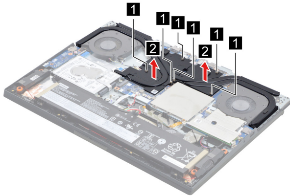
Figure 14. Loosen six screws and remove the heat sink
