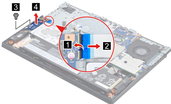
Figure 17. Remove the I/O board
