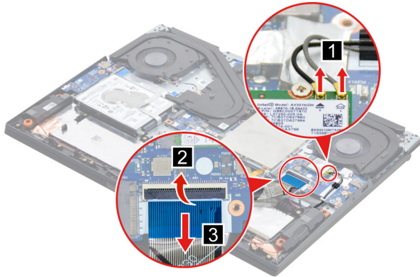
Figure 21. Detach the cables
