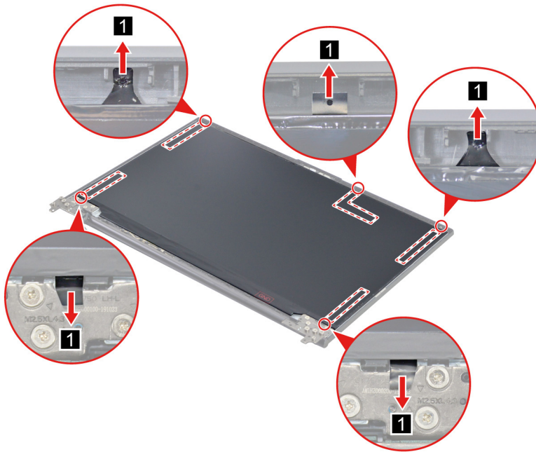
Figure 36. Pull out the pieces of adhesive tape with tweezers
