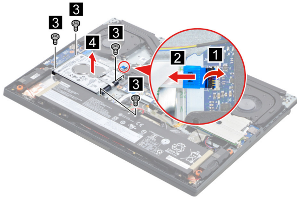
Figure 10. Remove the HDD module
