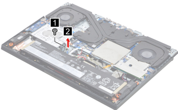
Figure 8. Remove the SSD stand off (for 2242 SSD only)
