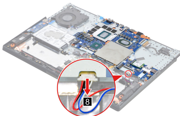
Figure 24. Disconnect the speaker cable from the system board
