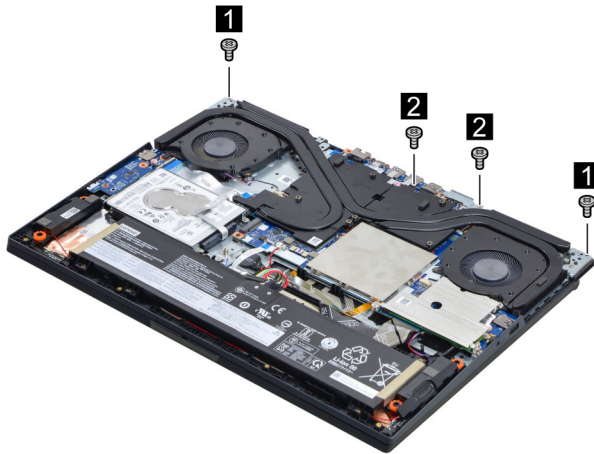
Figure 30. Remove four screws
