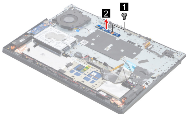
Figure 28. Remove the power board
