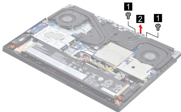
Figure 19. Remove the DC-in bracket
