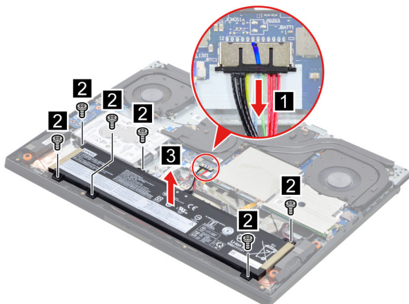
Figure 5. Remove the battery pack
