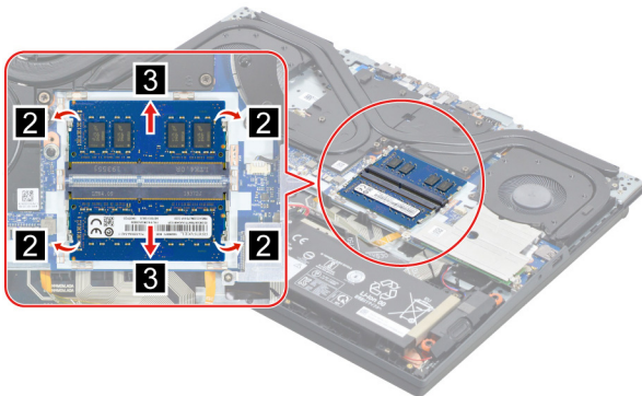
Figure 13. Remove the memory
