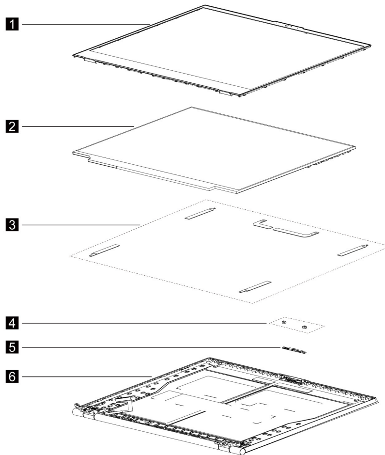
Figure 2. Lenovo Legion 5 (17", 05) LCD module — exploded view
