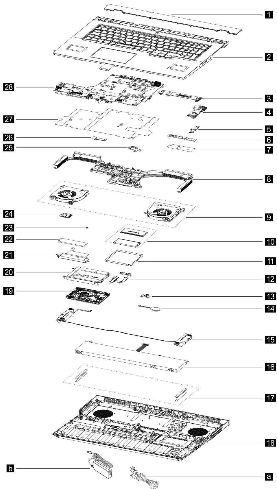
Figure 1. Lenovo Legion 5 (17", 05) exploded view
