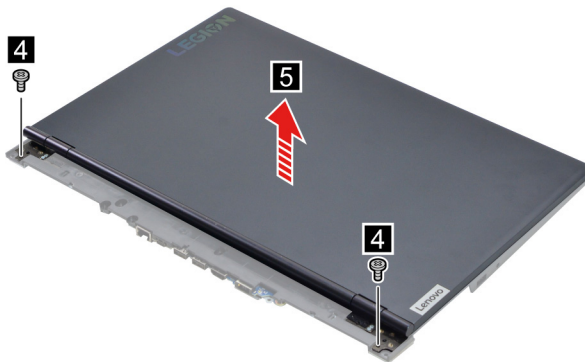
Figure 33. Remove two screws and lift the LCD module
