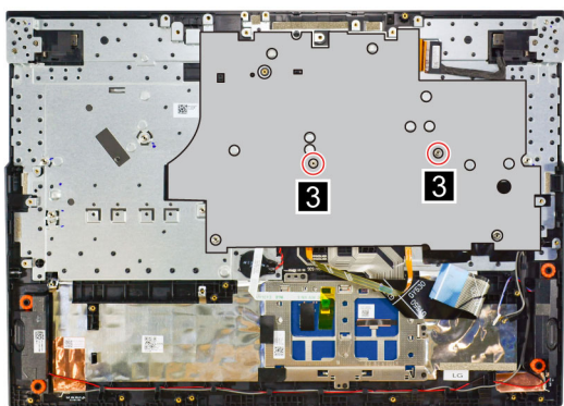
Figure 41. Attach the keyboard bracket mylar
