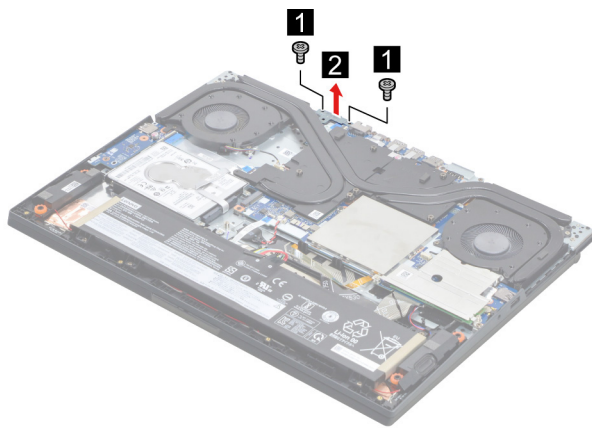
Figure 18. Remove the Kensington lock bracket
