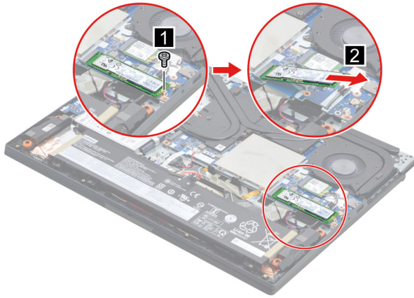
Figure 7. Remove the SSD
