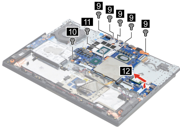
Figure 25. Remove seven screws and lift the system board
