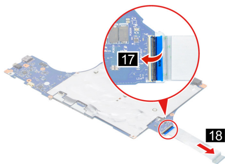
Figure 27. Remove the I/O board cable
