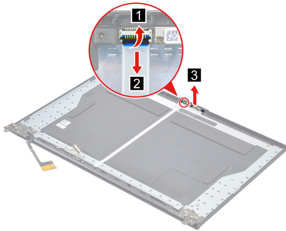
Figure 38. Remove the camera
