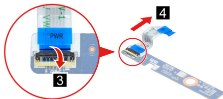
Figure 29. Remove the power board cable
