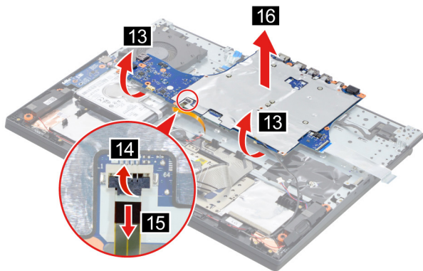
Figure 26. Remove the system board
