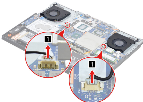
Figure 15. Disconnect the fan cables from the system board
