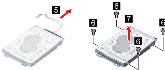
Figure 11. Separate the HDD cable, HDD and the HDD bracket
