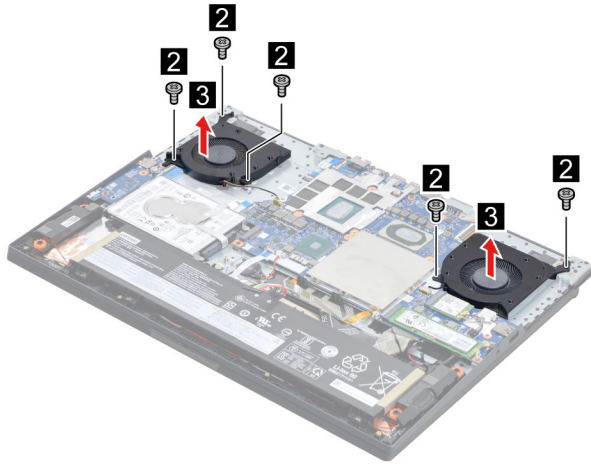
Figure 16. Remove five screws and remove the fan
