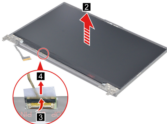
Figure 37. Remove the LCD panel
