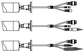
Figure 18: Wrapping the Power Connector and Reset Button
