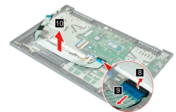
Figure 21. Disconnect and remove the USB board cable
