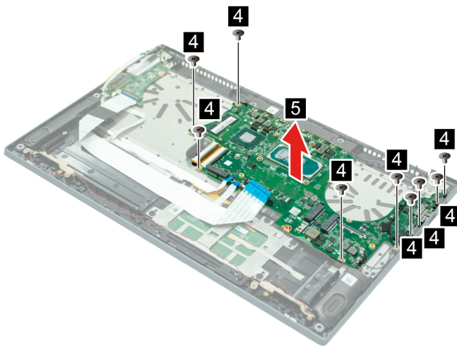
Figure 25. Remove the system board
