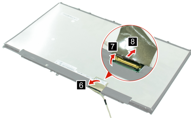
Figure 33. Disconnect the EDP cable
