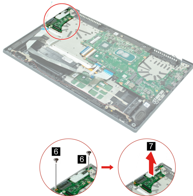
Figure 20. Remove the USB board
