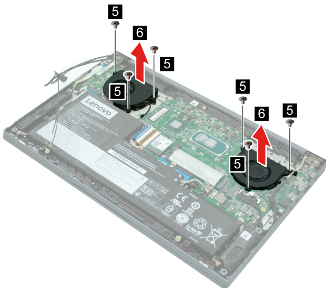
Figure 16. Remove the fans
