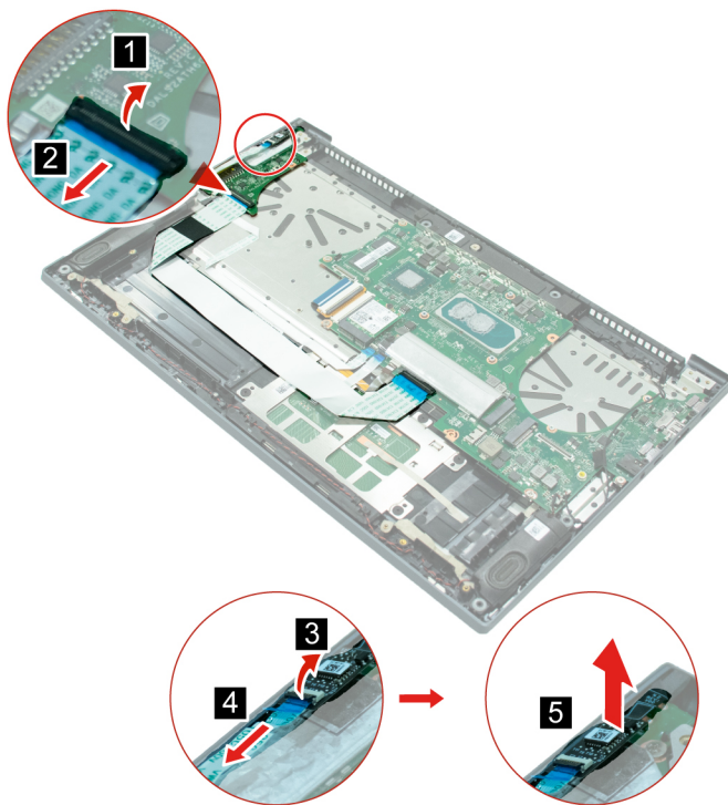
Figure 19. Disconnect cables and FP board
