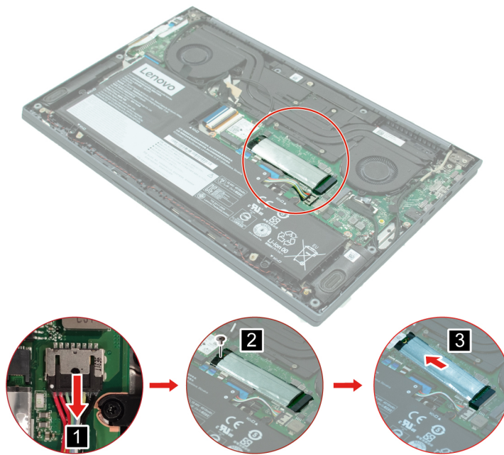
Figure 8. Remove the solid-state drive
