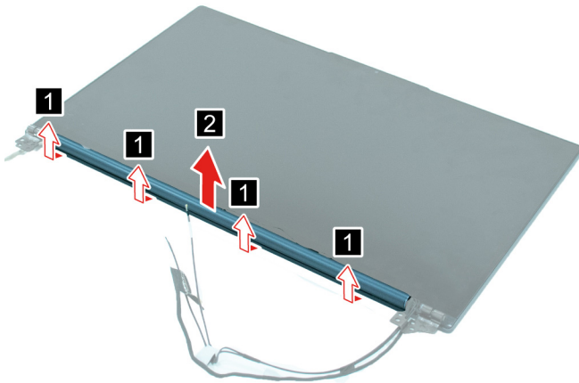
Figure 27. Remove the hinge cover
