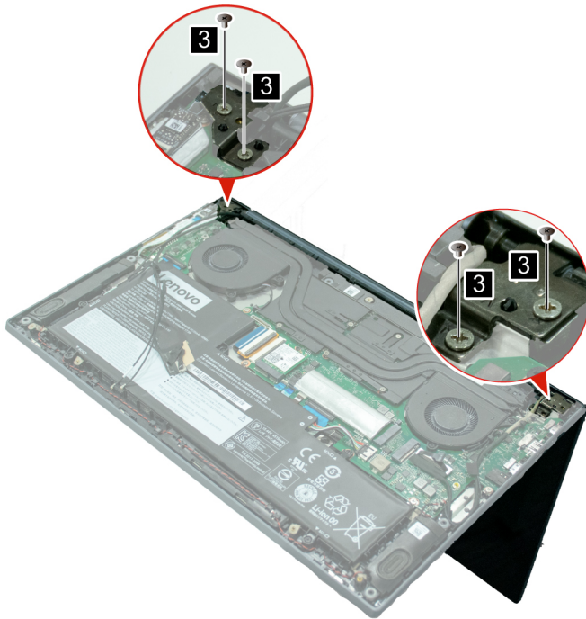
Figure 12. Rotate the LCD module and remove the four screws
