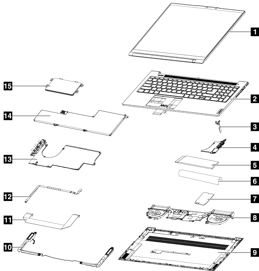
Figure 2. Exploded view 15-inch
