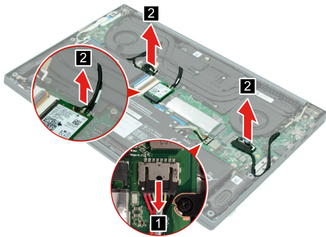
Figure 11. Disconnect the cables from the system board
