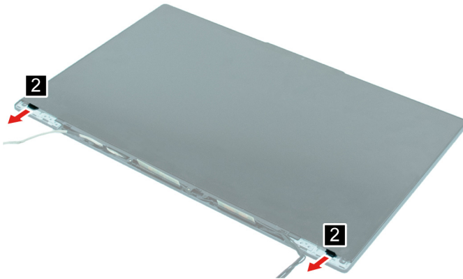
Figure 31. Remove adhesive strips
