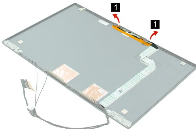
Figure 34. Disconnect the two camera cables
