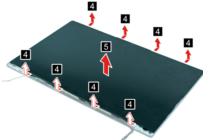
Figure 32. Remove bezel and panel
