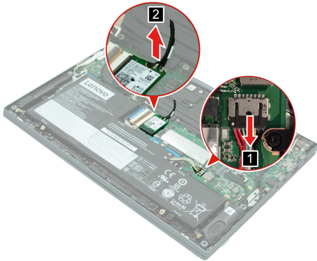
Figure 9. Disconnect the antennas
