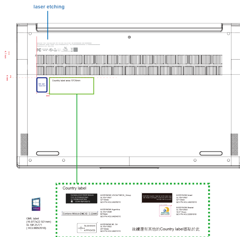
Figure 37. Label layout on the back side of the back cover 15"
