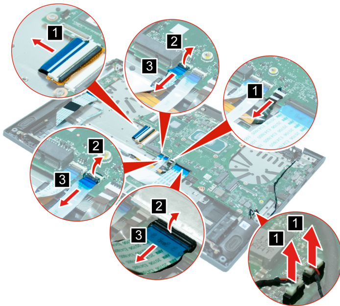
Figure 24. Disconnect cables
