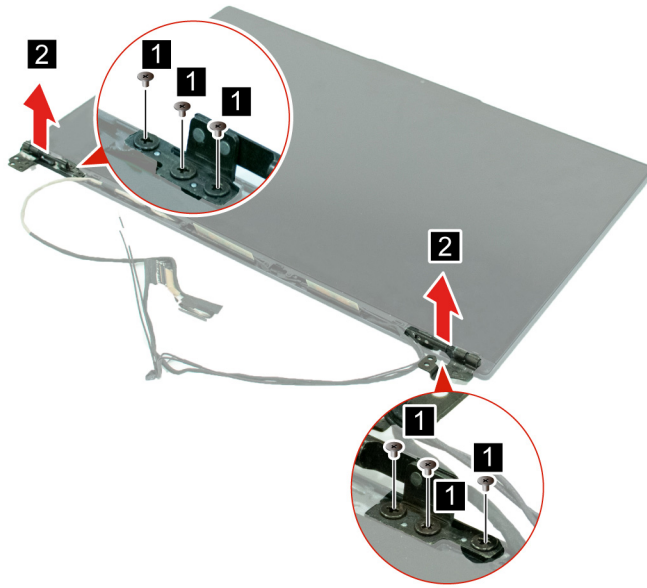
Figure 28. Remove the hinges
