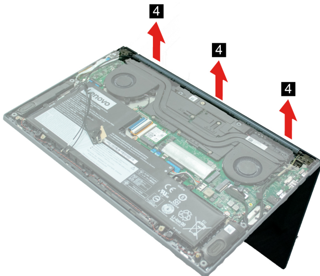
Figure 13. Remove the LCD module
