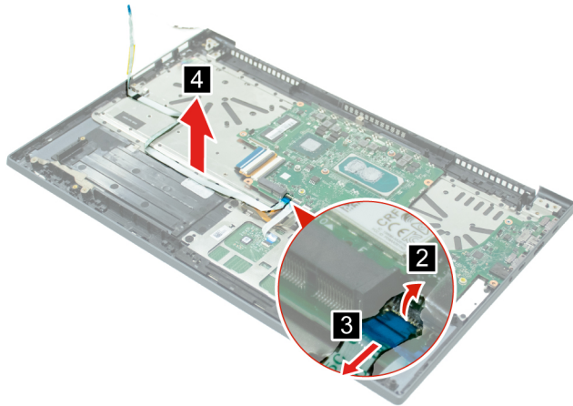
Figure 23. Disconnect the FP board cable and remove the cable.
