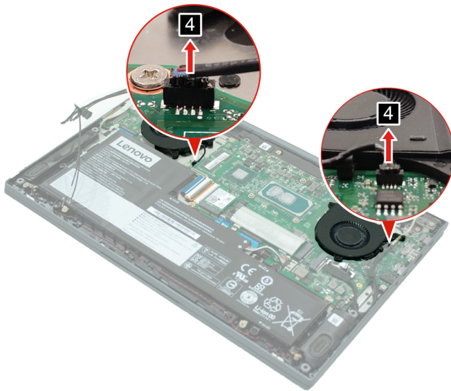
Figure 15. Disconnect the fan power cables
