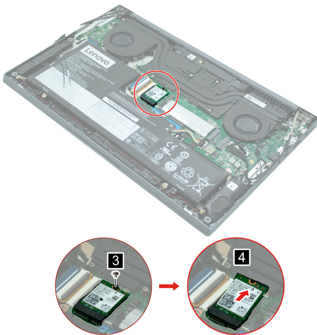
Figure 10. Remove the WLAN
