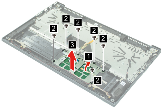
Figure 26. Remove the touchpad
