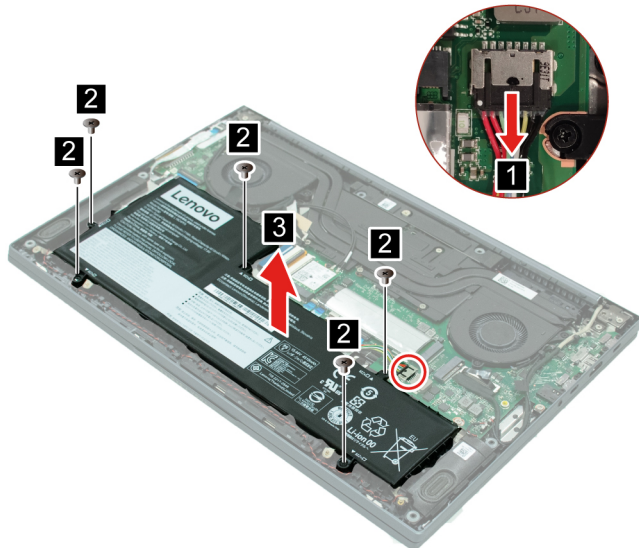
Figure 7. Remove the battery
