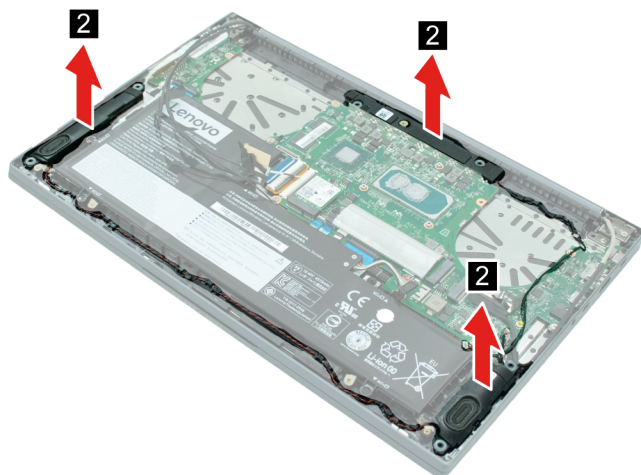
Figure 18. Remove speakers (and subwoofer)
