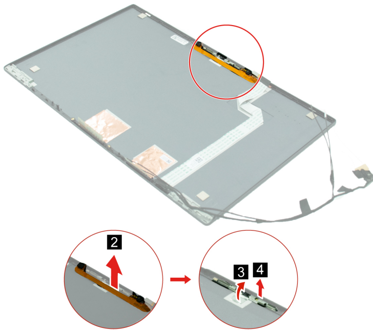
Figure 35. Remove the camera cable and camera
