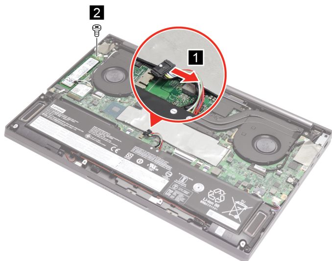
Figure 13. Remove one screw
