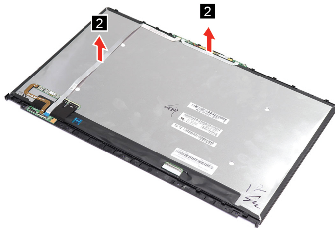
Figure 42. Remove the microphone and camera module
