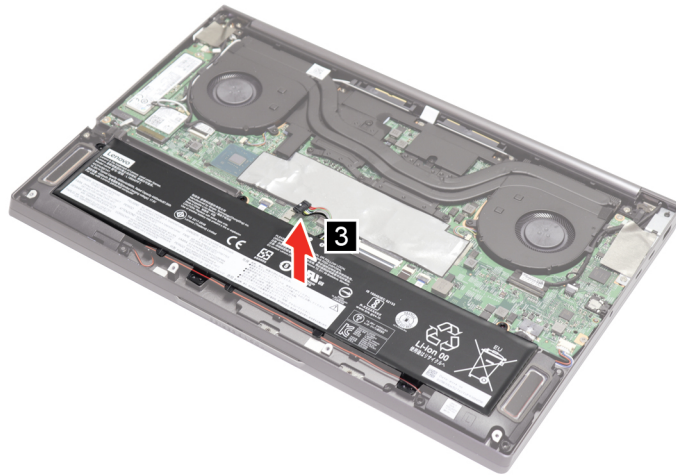
Figure 7. Remove the battery pack
