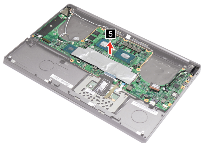
Figure 25. Remove main board
