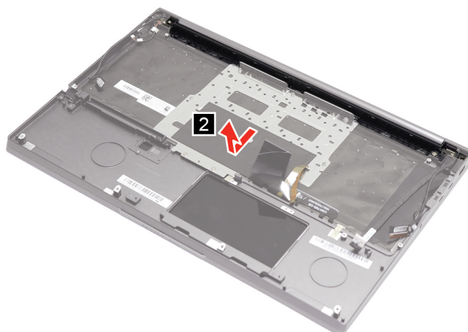
Figure 33. Remove upper case.
