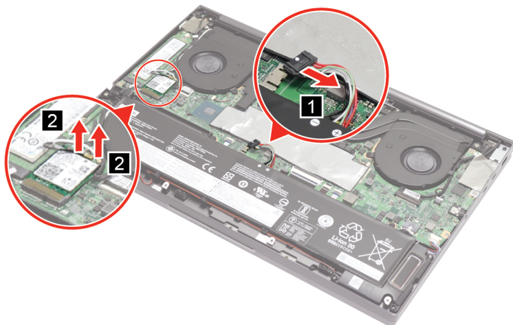
Figure 10. Disconnect the cables
