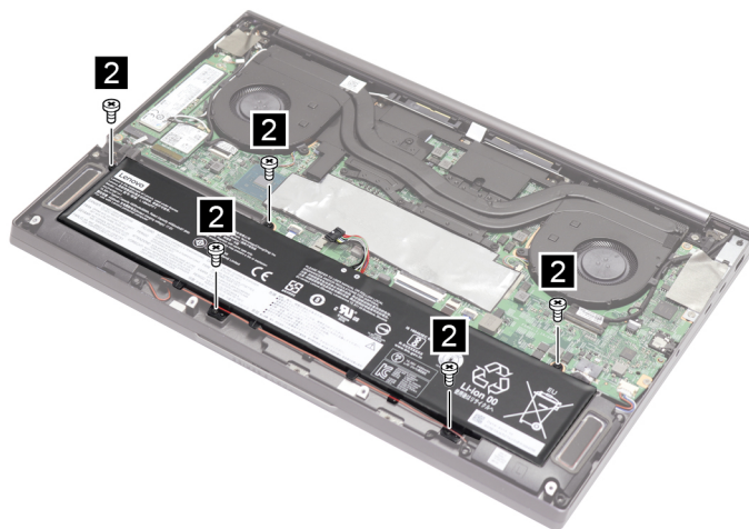
Figure 6. Remove five screws
