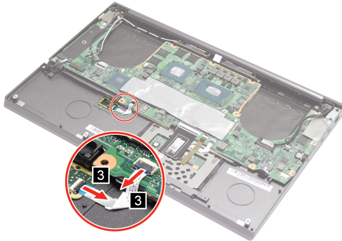
Figure 20. Disconnect the fingerprint sensor cable
