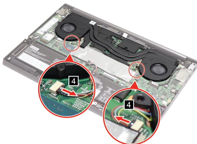
Figure 16. Disconnect fan cables
