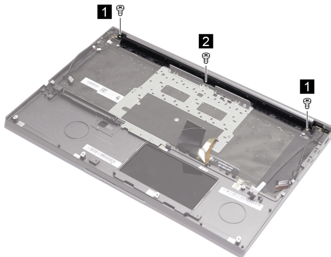
Figure 30. Remove three screws
