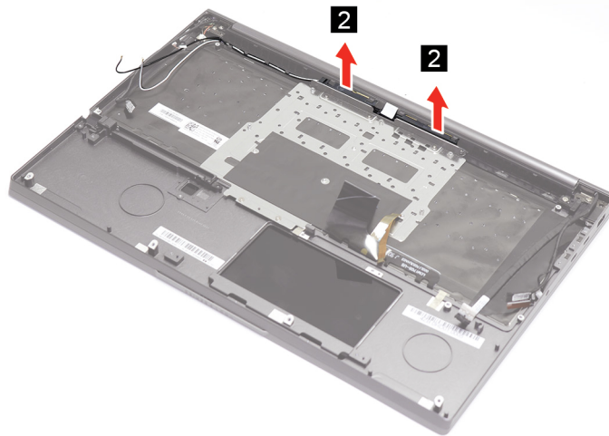
Figure 29. Disconnect the cables.
