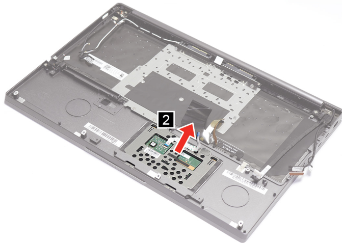
Figure 27. Remove touch pad
