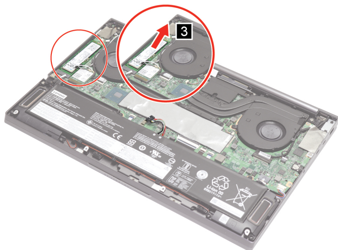
Figure 14. Slide the M.2 solid-state drive out of the slot
