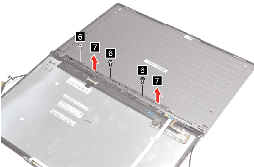
Figure 37. Remove three screws and remove the panel frame
