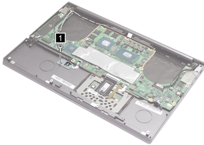
Figure 18. Remove one screw
