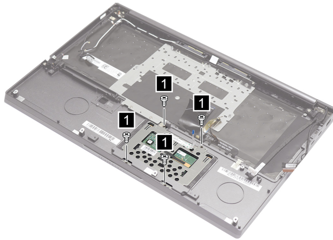
Figure 26. Remove four screws
