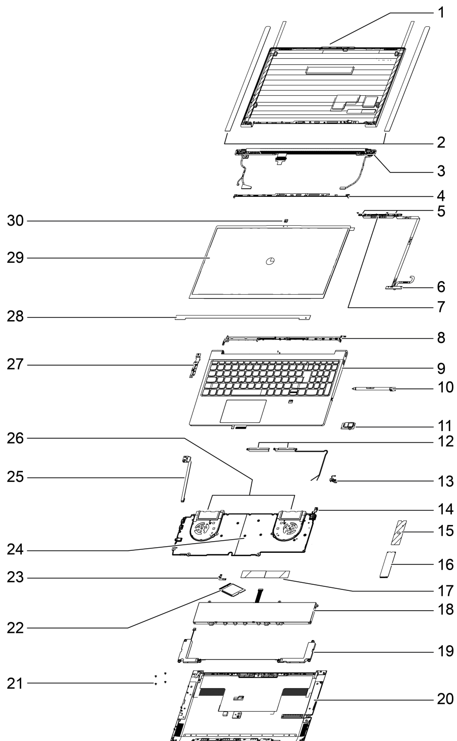
Figure 1. Lenovo Yoga 9 15IMH5 exploded view
