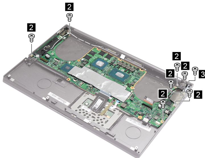
Figure 23. Remove eight screws
