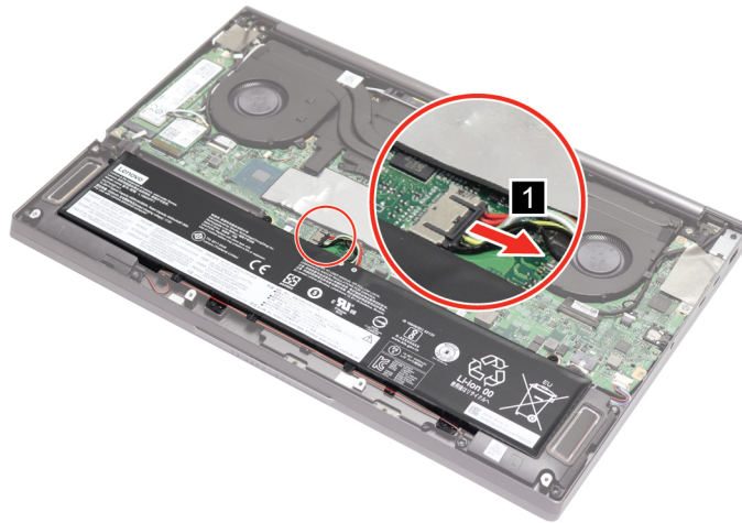
Figure 5. Disconnect the cable
