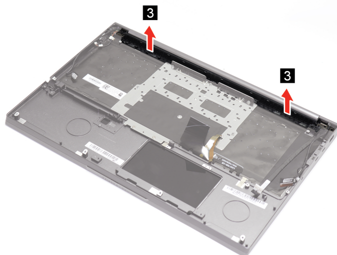
Figure 31. Remove the thermal cover
