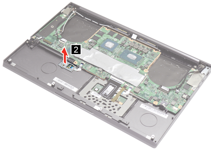
Figure 19. Remove the fingerprint sensor cover
