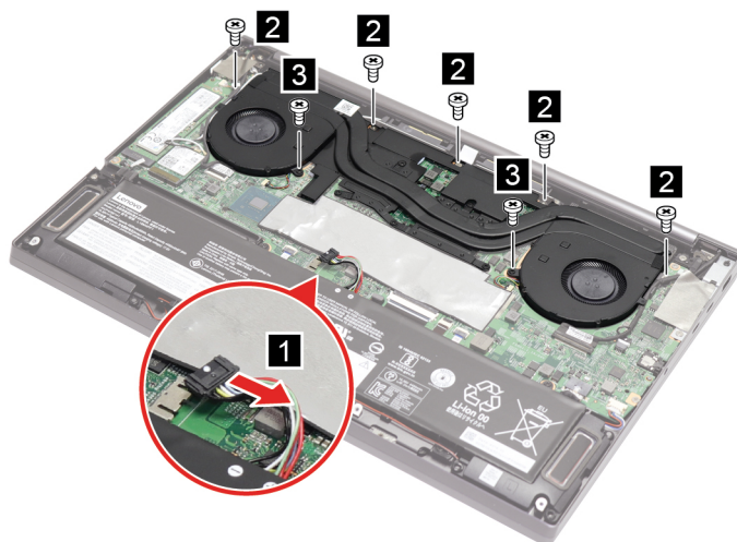
Figure 15. Remove seven screws
