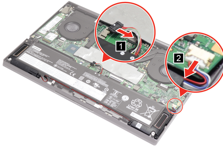
Figure 8. Disconnect the cables
