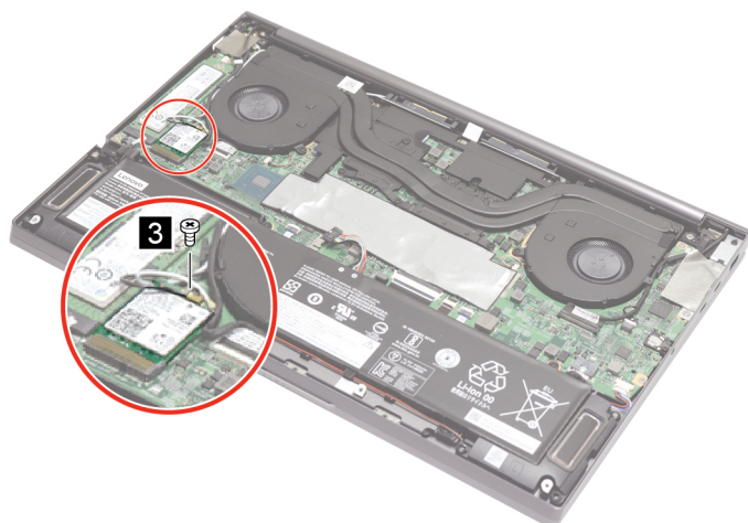
Figure 11. Remove one screw
