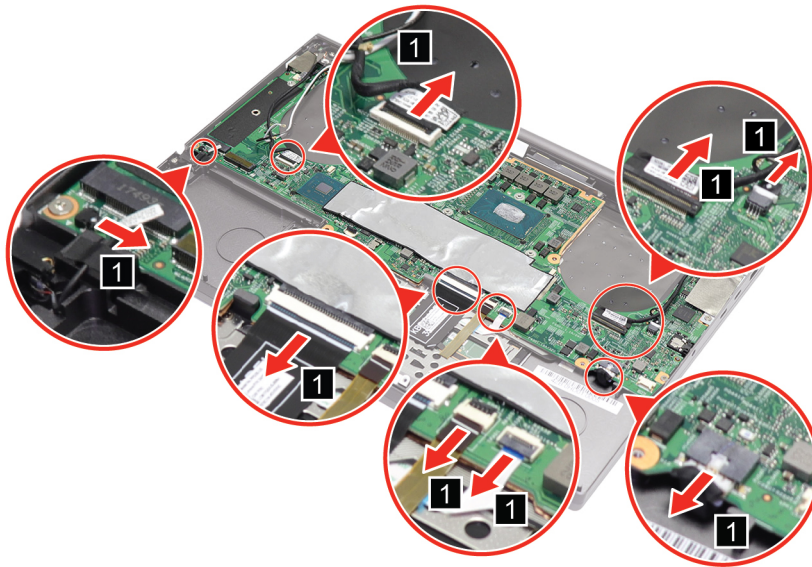
Figure 22. Disconnect cables
