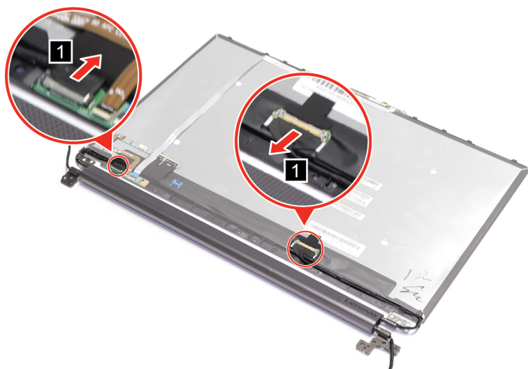
Figure 39. Disconnect the cables
