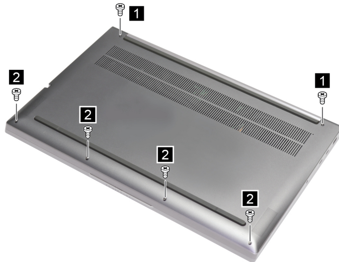
Figure 3. Remove six screws
