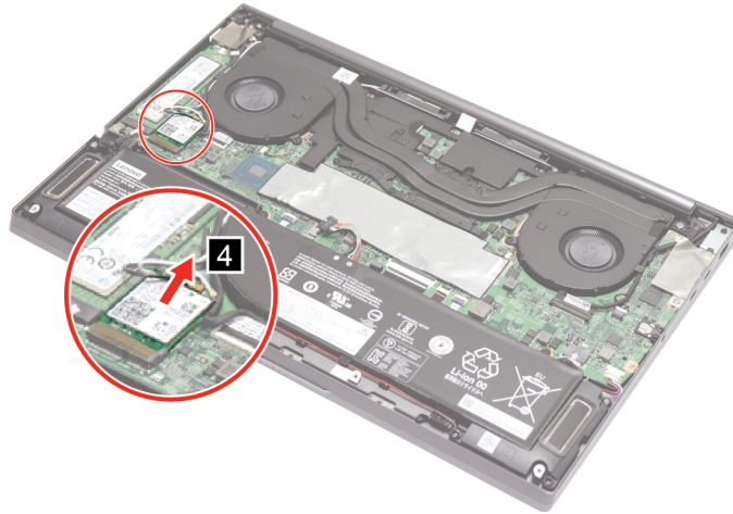
Figure 12. Slide the WLAN card out of the slot
