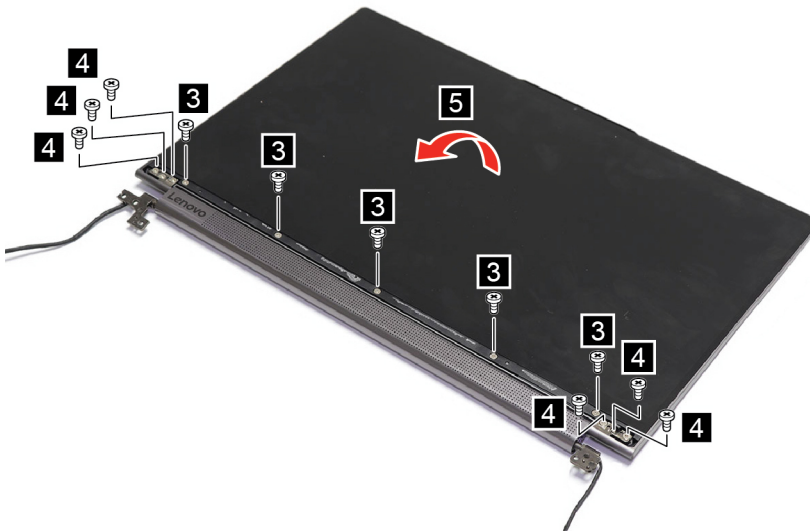
Figure 36. Remove eleven screws and turn the LCD panel
