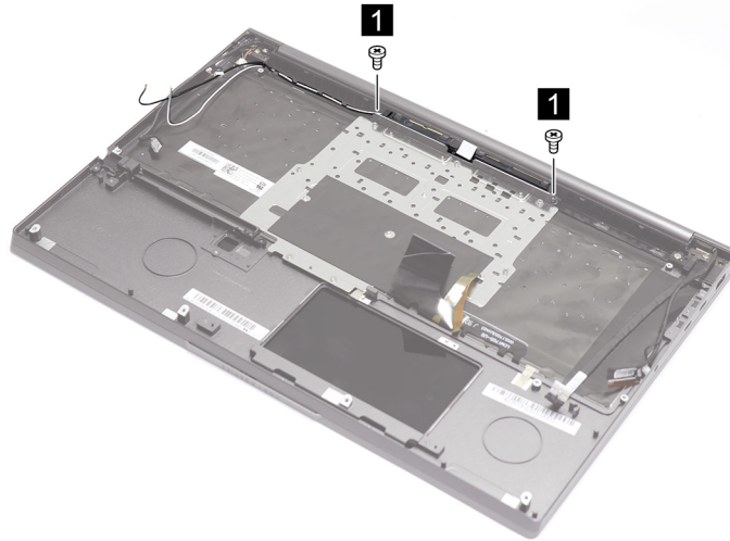
Figure 28. Remove two screws
