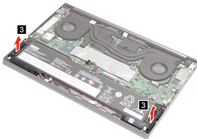
Figure 9. Remove the speakers
