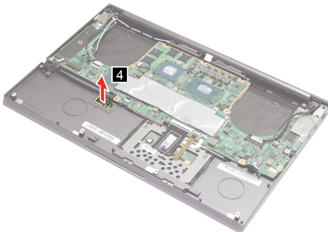
Figure 21. Remove the fingerprint sensor
