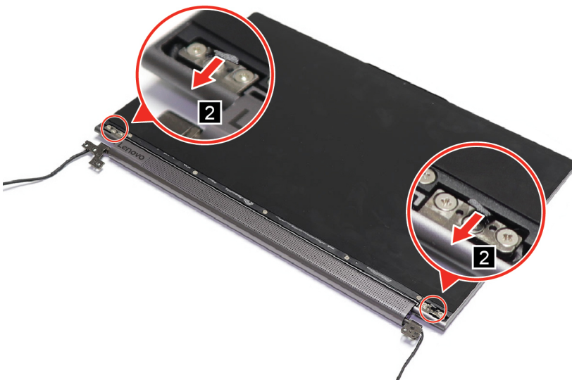
Figure 35. Pull out adhesive tapes
