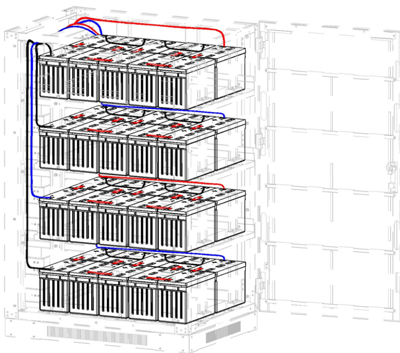
Figure 5-43: Model BP240V100L-NIB
