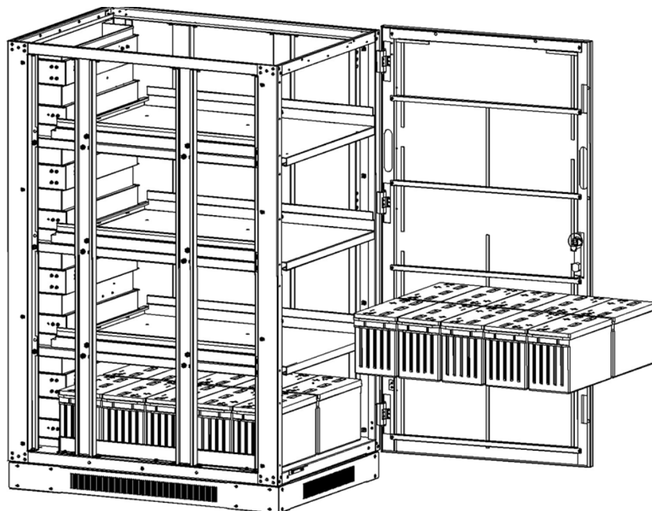
Figure 5-34: Model BP240V100L-NIB
