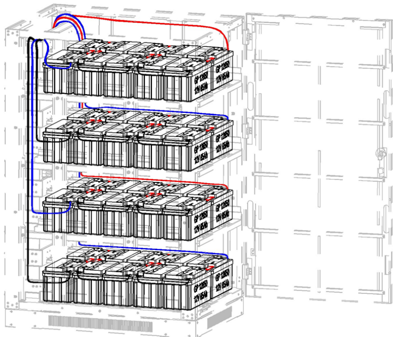
Figure 5-42: Model BP240V65L-NIB
