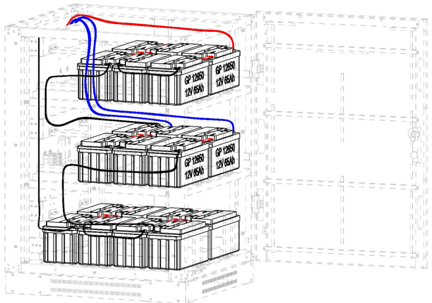
Figure 5-19: Model BP240V65-NIB
