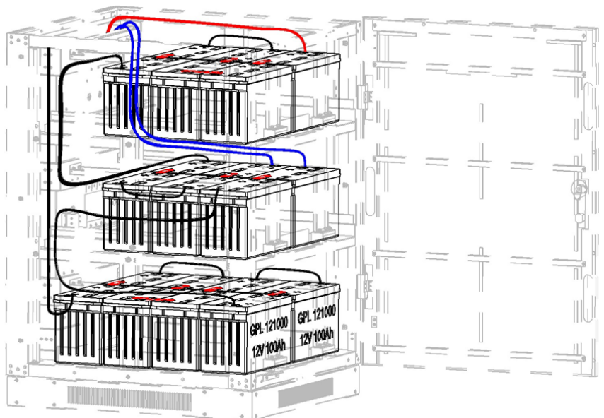
Figure 5-20: Model BP240V100-NIB
