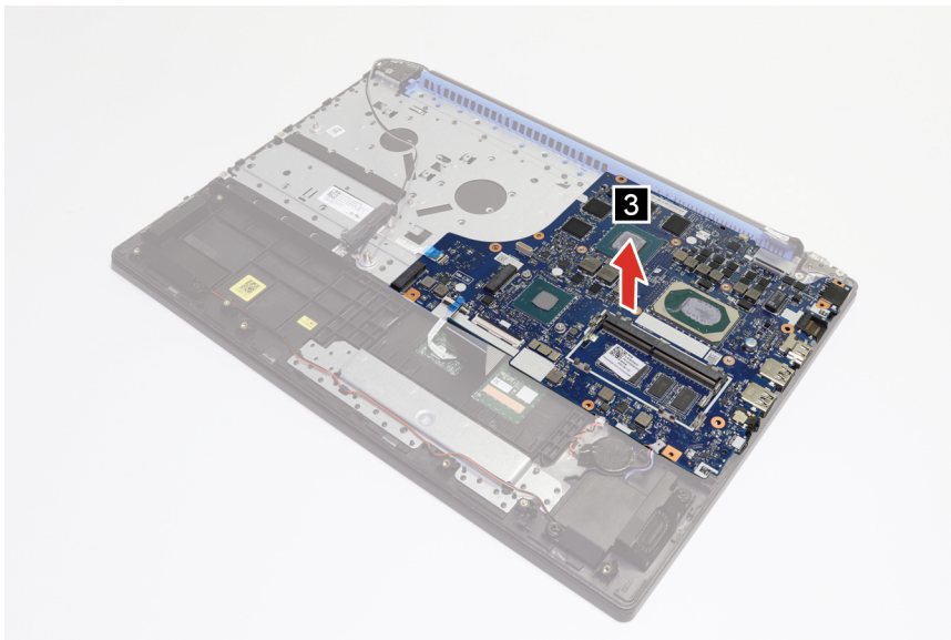
Figure 17. Remove the system board
