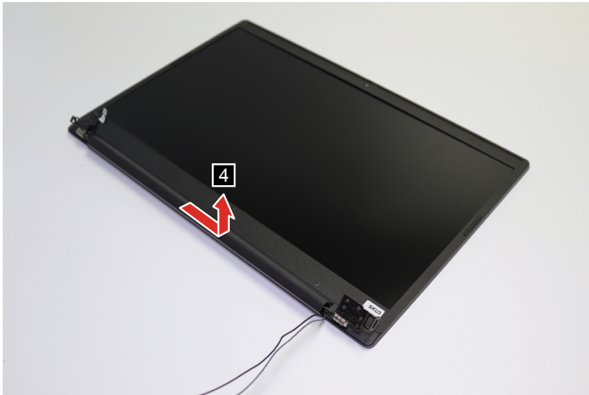
Figure 24. Remove the hinge cap
