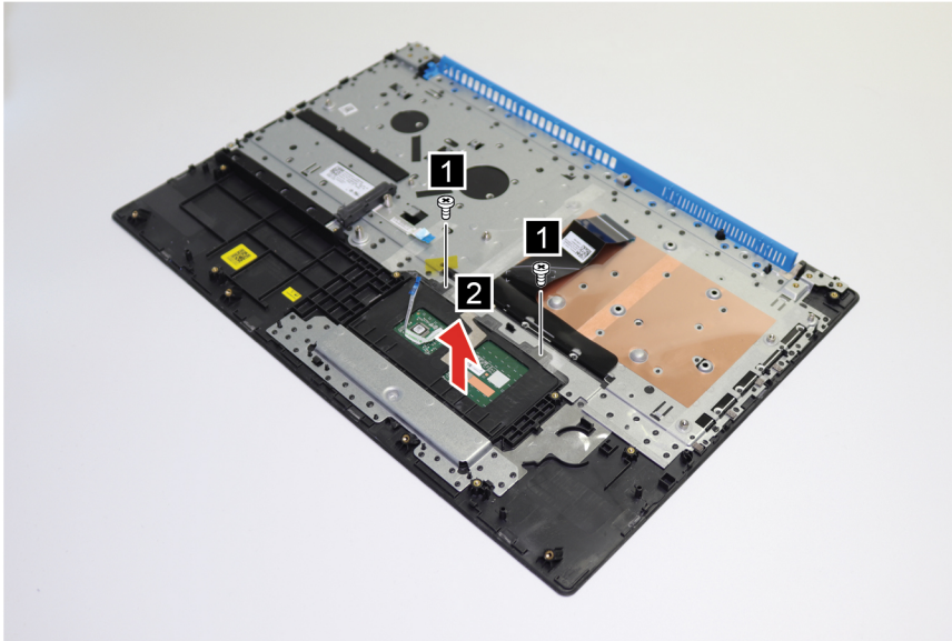
Figure 20. Remove the screws and detach the touchpad
