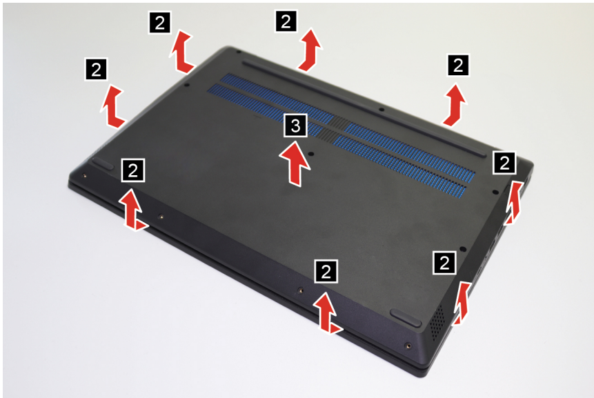
Figure 3. Remove the lower case
