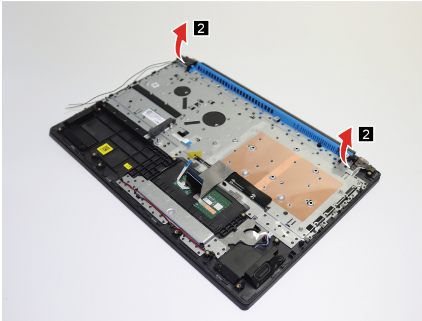
Figure 22. Open the hinges
