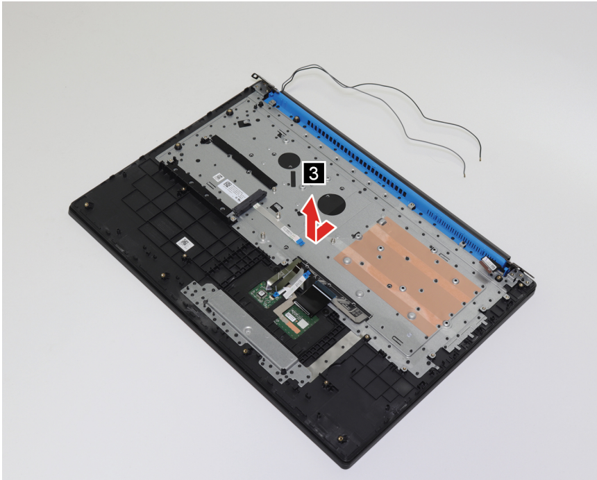
Figure 32. Remove the upper case
