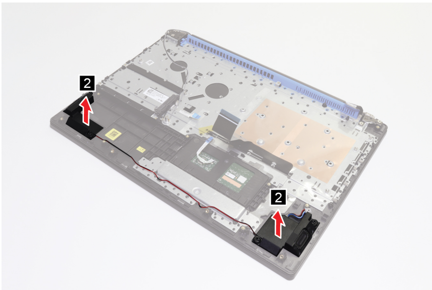
Figure 19. Remove the speakers
