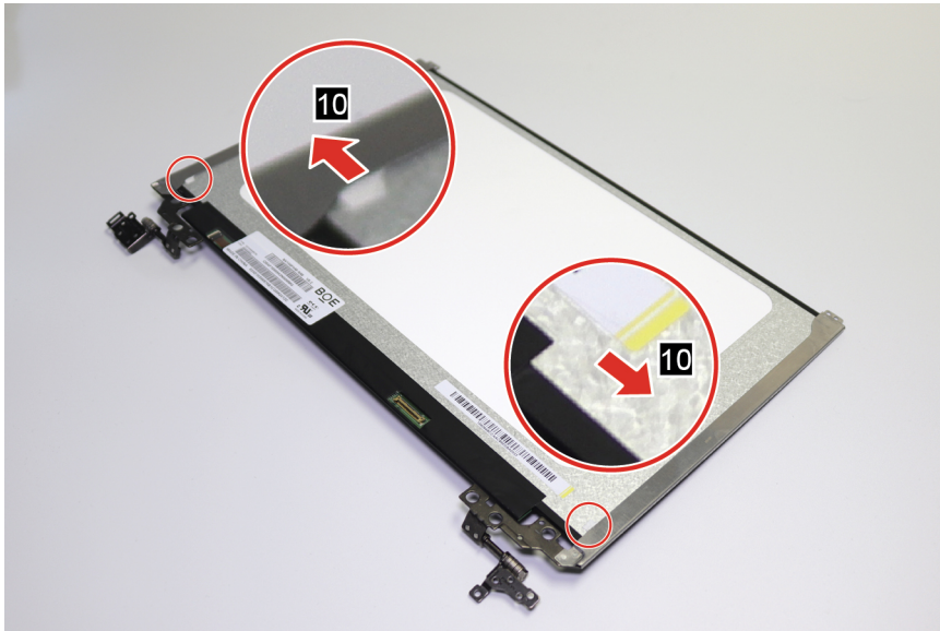
Figure 29. Remove the hinge modules
