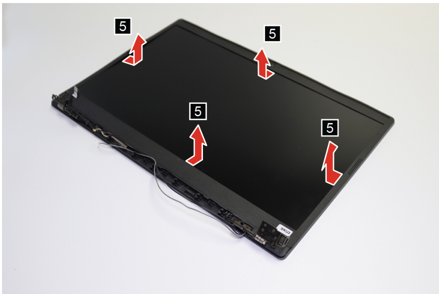
Figure 25. Remove the LCD front bezel
