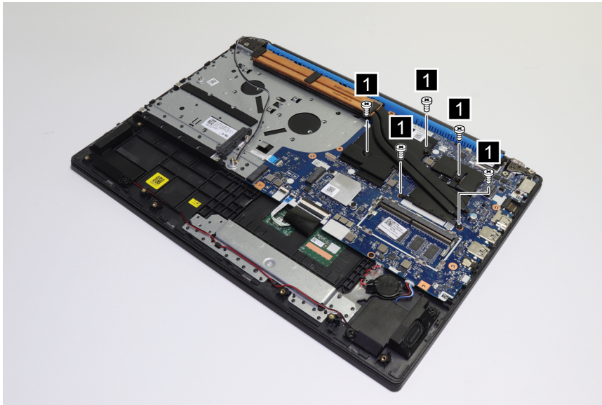
Figure 13. Remove the screws
