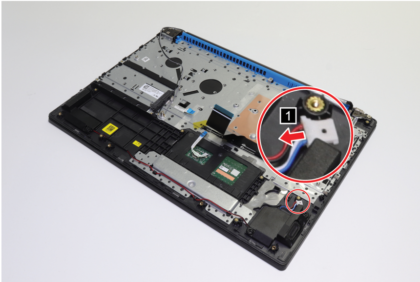
Figure 18. Disconnect the cable
