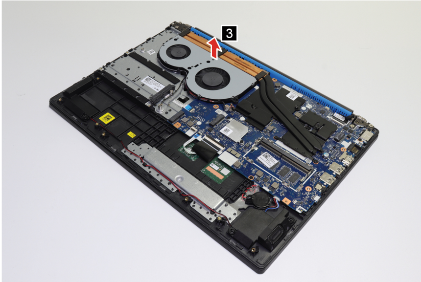
Figure 12. Remove the fans
