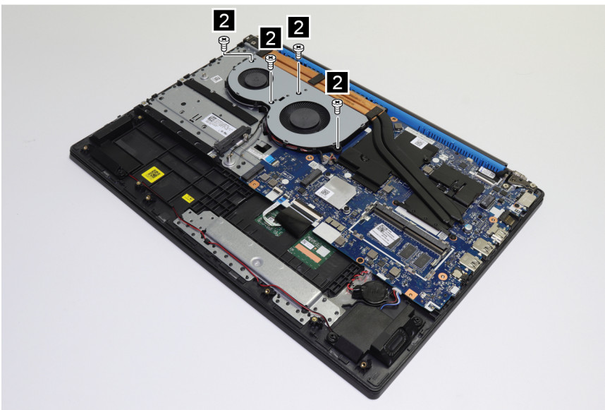
Figure 11. Remove the screws
