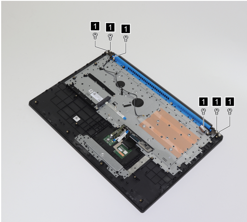
Figure 30. Remove the screws
