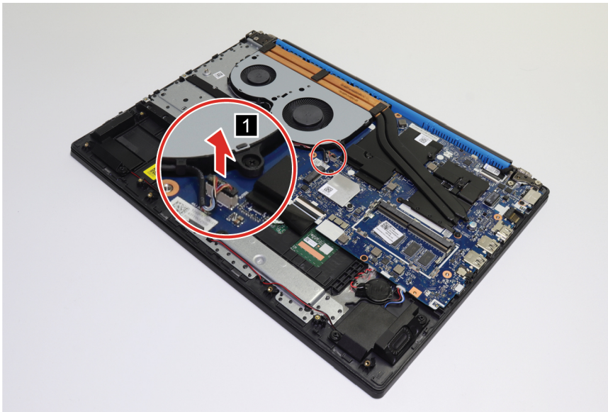
Figure 10. Disconnect the fan cables
