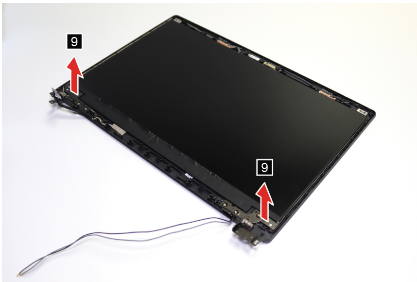
Figure 27. Remove the LCD hinges
