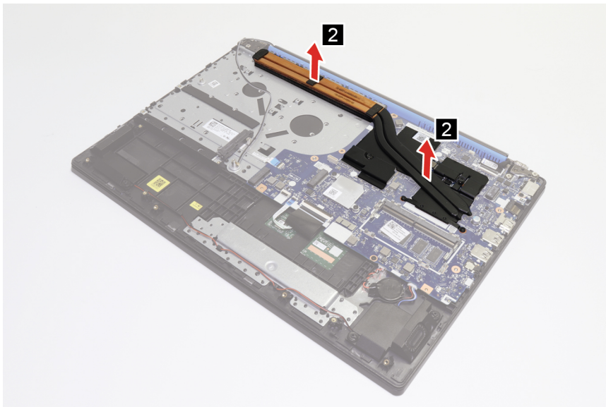
Figure 14. Remove the heat sink
