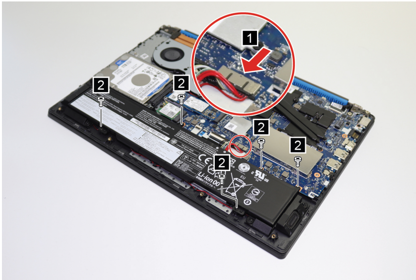
Figure 6. Remove the battery pack
