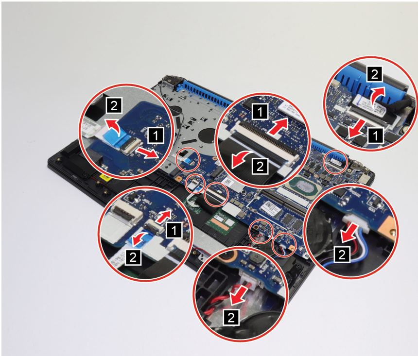
Figure 15. Release the latch and disconnect the cables
