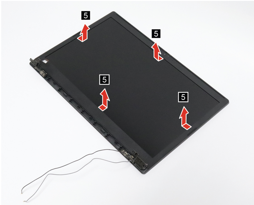
Figure 34. Remove the LCD front bezel
