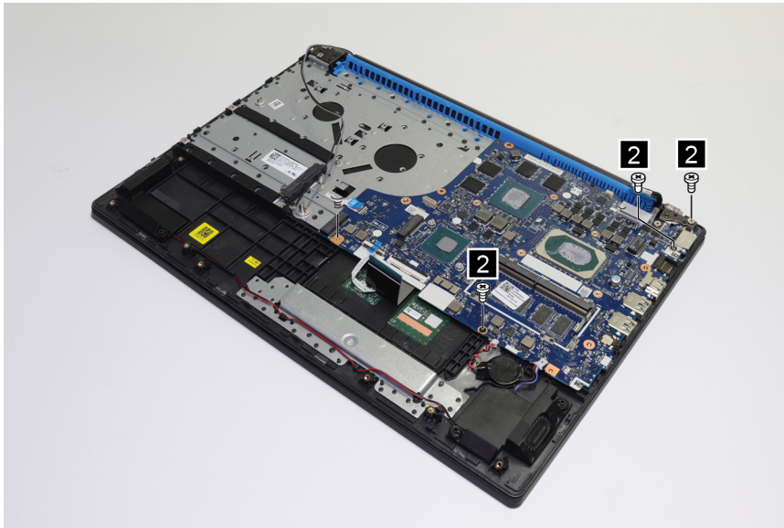
Figure 16. Remove the screws
