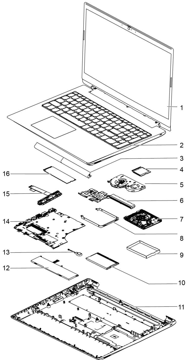
Figure 1. Lenovo IdeaPad L340 IRH Gaming exploded view
