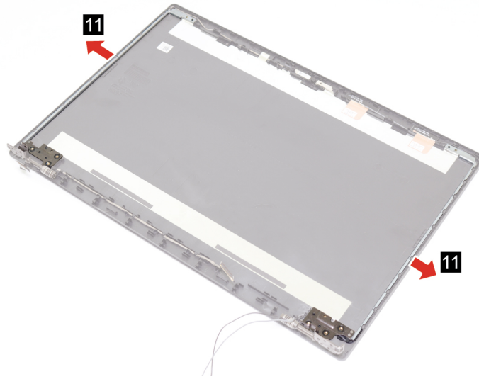
Figure 38. Remove the hinge modules
