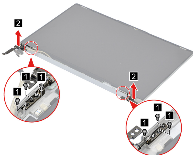
Figure 32. Remove six screws and remove the hinges.
