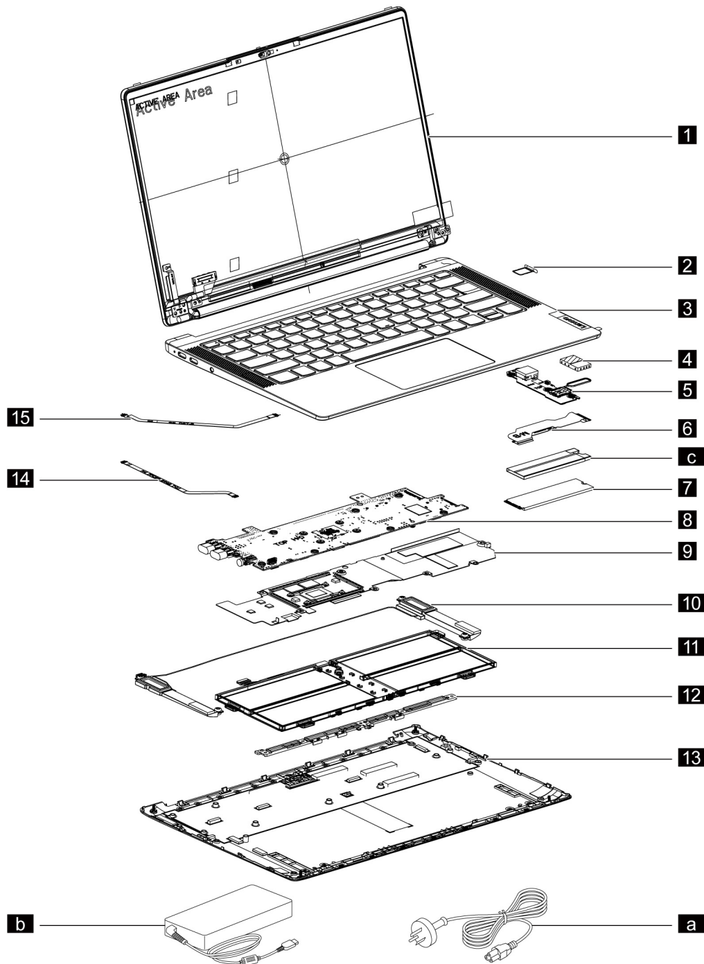
Figure 1. IdeaPad 4G (14", 05), IdeaPad 14m 4G 2021 and IdeaPad 14m 4G 2021 DM exploded view
