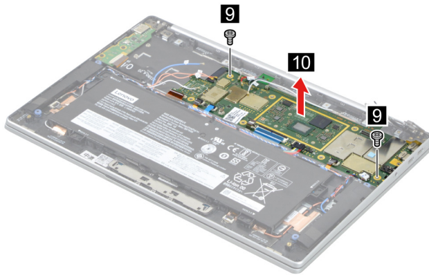
Figure 23. Remove two screws and then remove the system board.
