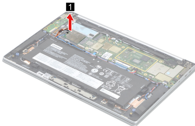
Figure 18. Detach the antenna cable connectors.
