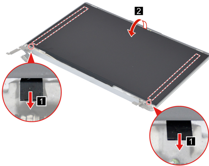
Figure 33. Remove the two pieces of removable tape with tweezers and turn over the LCD panel.
