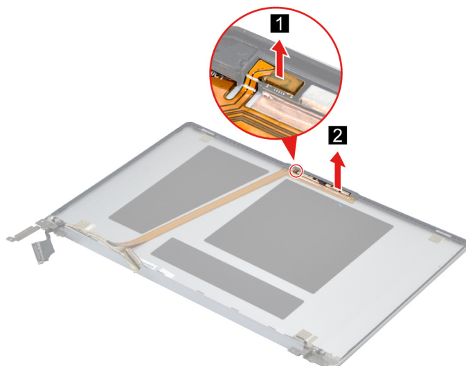
Figure 37. Disconnect the EDP cable from the camera and remove the camera.
