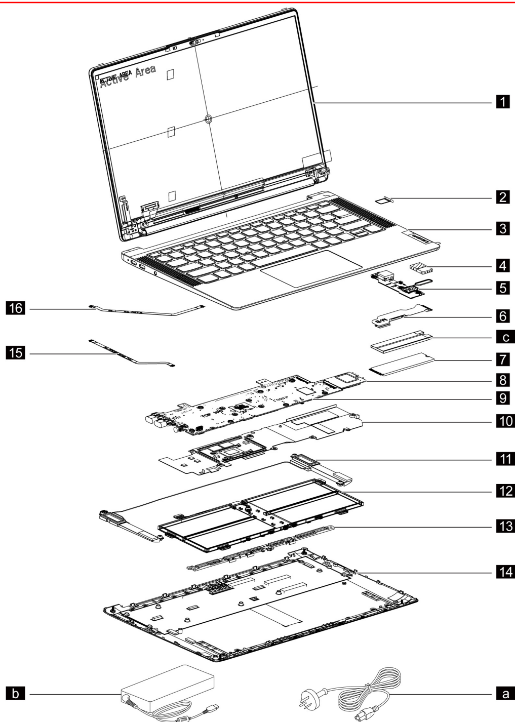
Figure 2. IdeaPad 5G (14", 05), IdeaPad 14m 5G 2021 and IdeaPad 14m 5G 2021 DM exploded view
