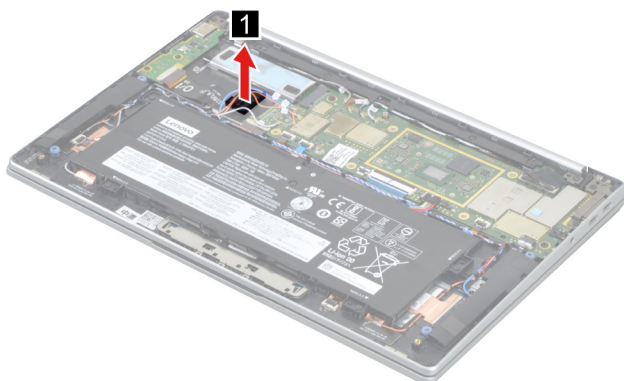
Figure 17. Remove the rubber foot.
