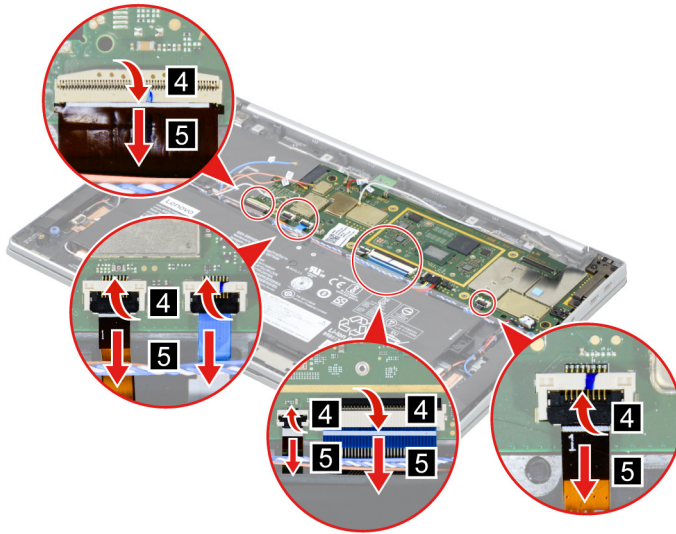
Figure 21. Disconnect cables connected to the system board.
