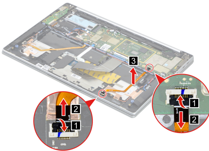
Figure 25. Remove the function board cable (left).
