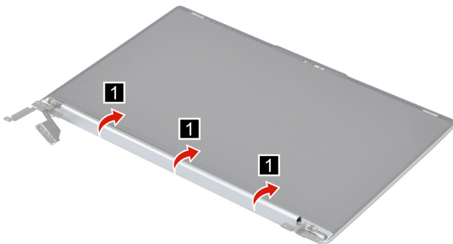
Figure 30. Remove the hinge cover.
