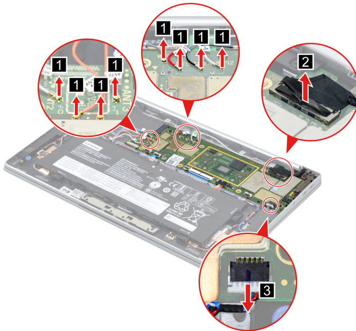
Figure 20. Detach the antenna cable connectors. Disconnect the EDP cable and the speaker cable from the system board.
