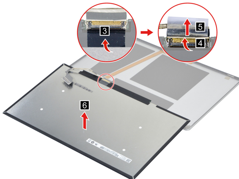
Figure 34. Remove the LCD panel.
