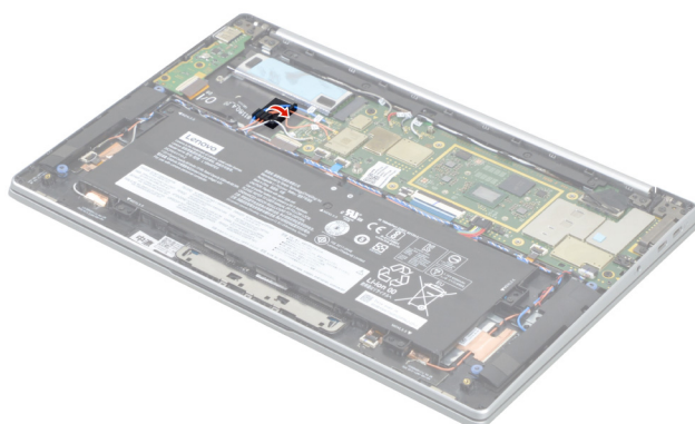
Figure 16. Release the antenna cables from the cable guide with tweezers carefully.
