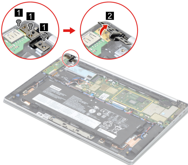
Figure 13. Remove three screws and open the hinge.
