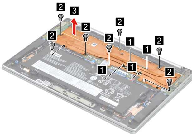
Figure 9. Remove the thermal module.
