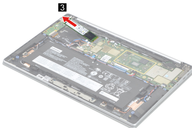
Figure 12. Remove the SSD by pulling it away from the slot.
