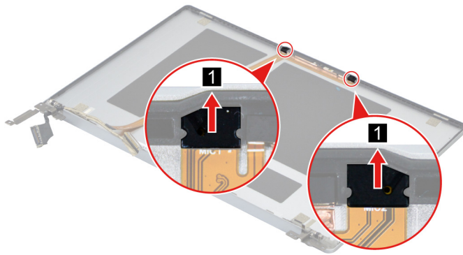
Figure 36. Remove the microphone rubbers.
