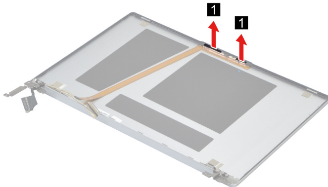
Figure 35. Remove the camera rubbers.
