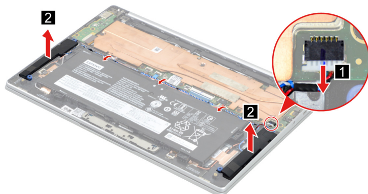
Figure 8. Remove the speakers.
