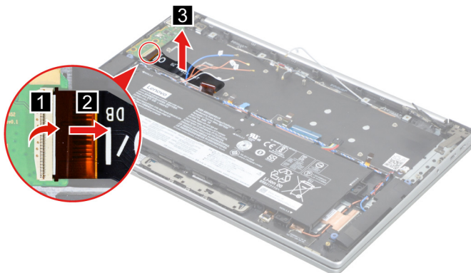
Figure 24. Disconnect the USB board cable from the USB board and remove the USB board cable.
