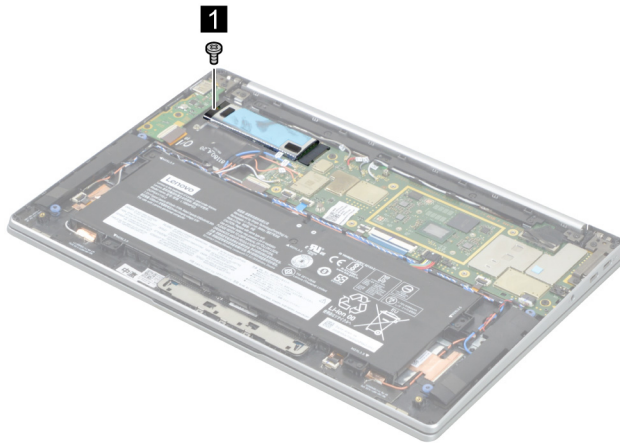
Figure 10. Remove one screw.
