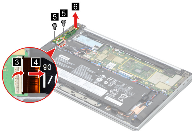
Figure 14. Remove two screws and remove the USB board.
