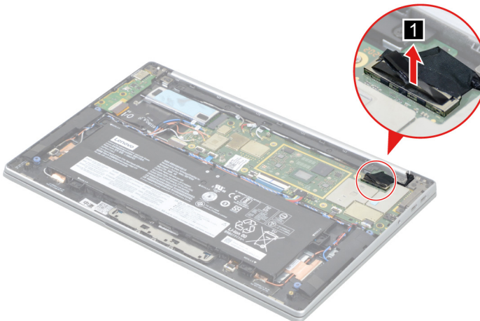
Figure 27. Disconnect the EDP cable from the system board.
