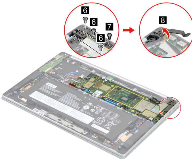
Figure 22. Remove four screws and open the hinge.
