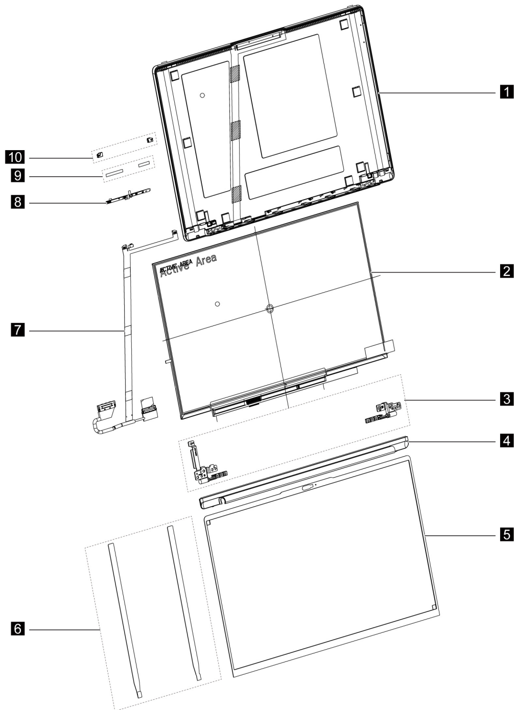
Figure 3. IdeaPad 4G (14", 05), IdeaPad 5G (14", 05), IdeaPad 14m 4G 2021, IdeaPad 14m 5G 2021, IdeaPad 14m 4G 2021 DM and IdeaPad 14m 5G 2021 DM LCD module - exploded view
