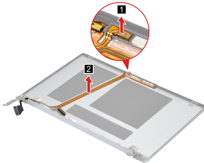
Figure 38. Disconnect the EDP cable from the camera and remove the EDP cable.
