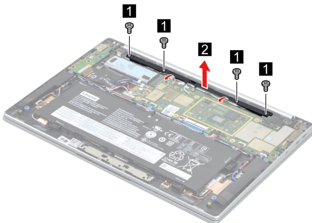
Figure 15. Remove four screws and remove the antenna bracket.
