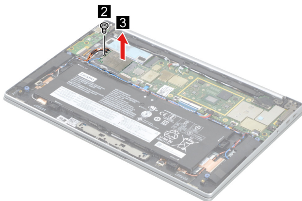
Figure 19. Remove one screw and then remove the 5G module.
