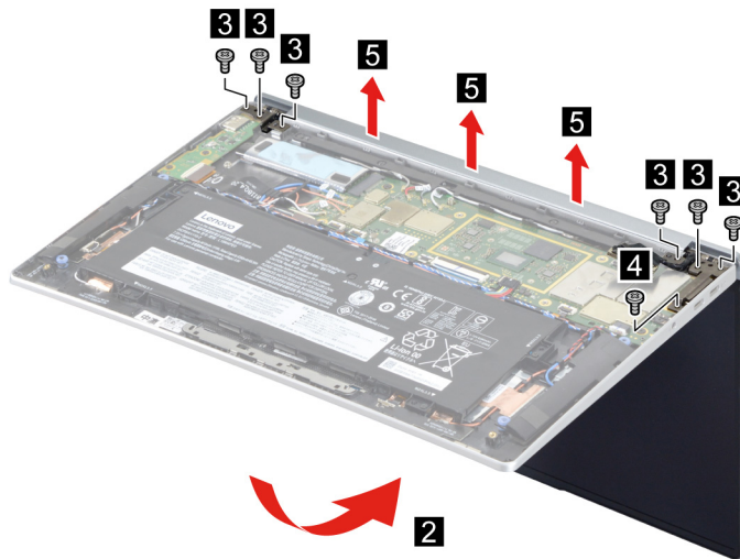
Figure 28. Remove seven screws and remove the LCD module.
