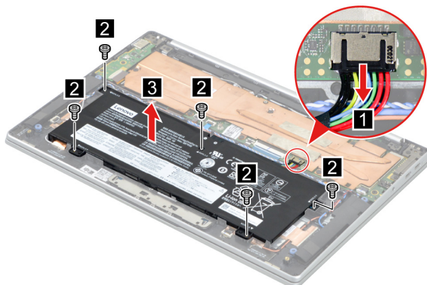
Figure 7. Remove five screws and remove the battery pack.
