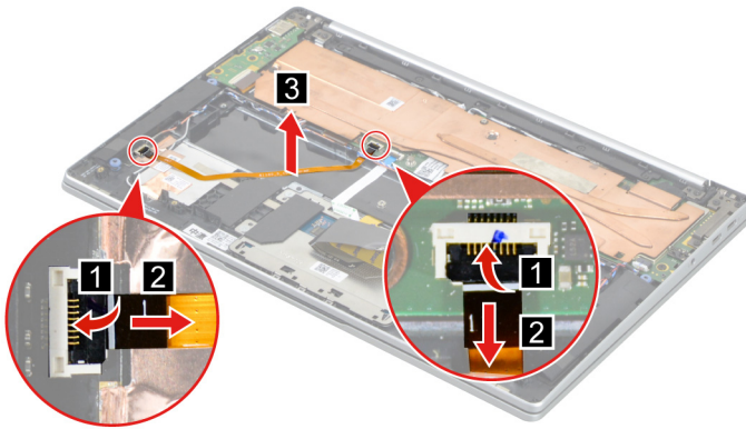
Figure 26. Remove the function board cable (right).
