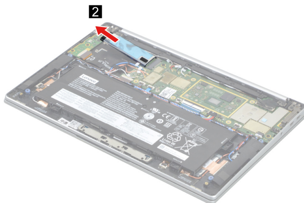
Figure 11. Remove the SSD foil.
