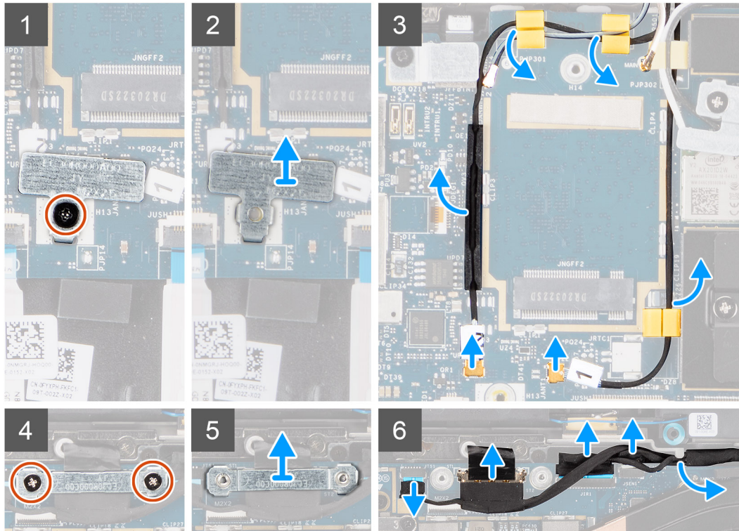
Figure 3. Display assembly with WLAN and WWAN antenna
